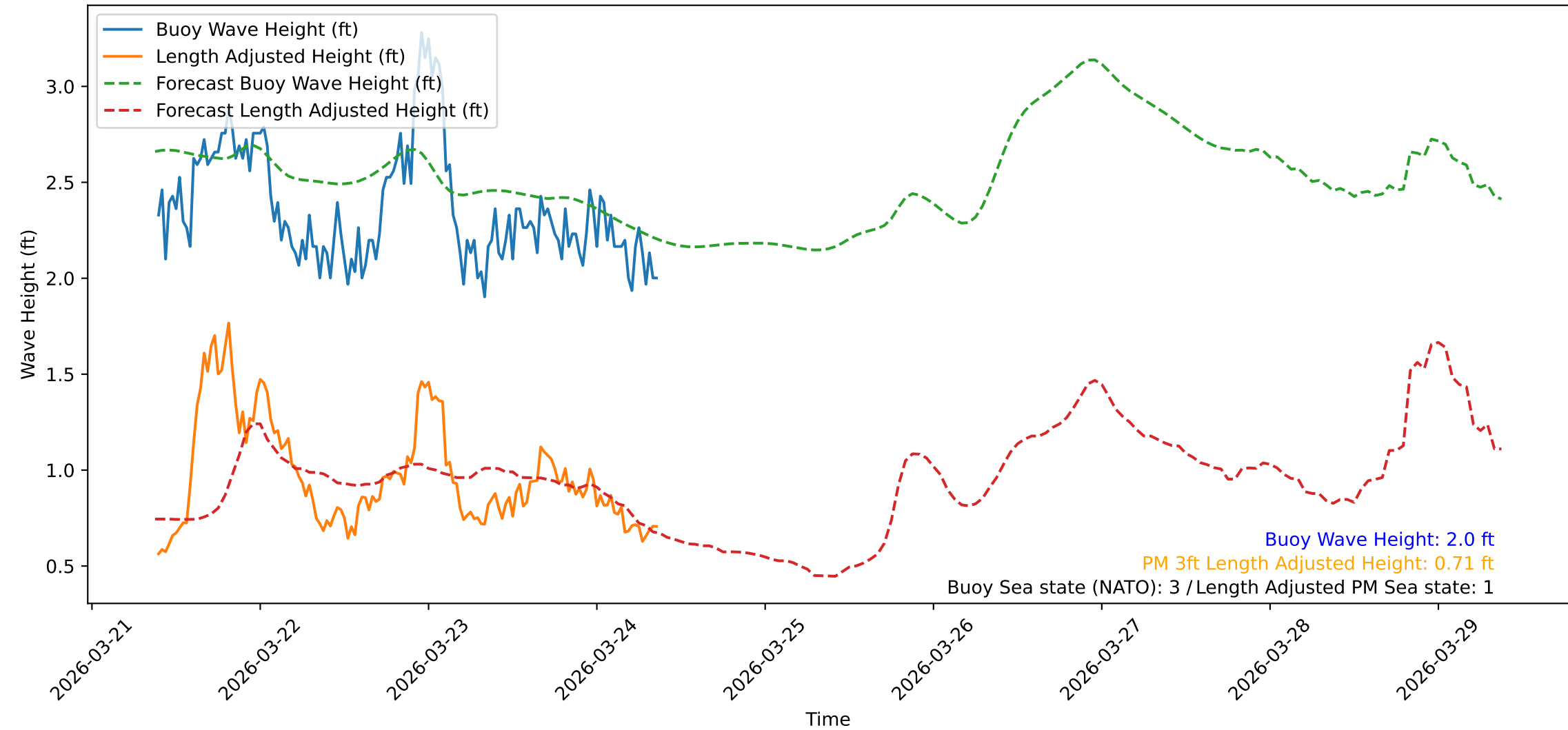
Wave Heights over Time for Green Beach at 2026-03-24 09:21:09
