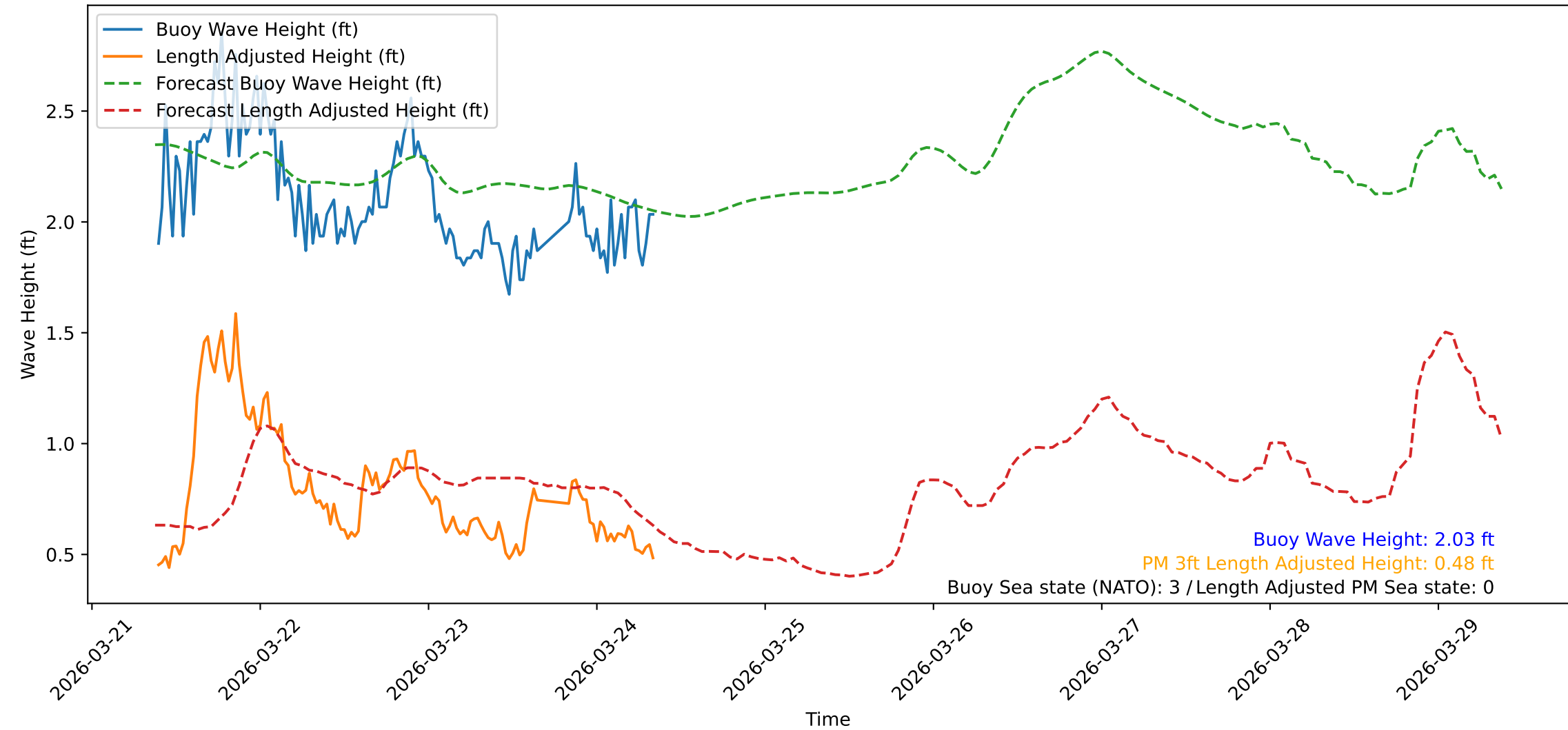
Wave Heights over Time for Red Beach at 2026-03-24 09:20:47
