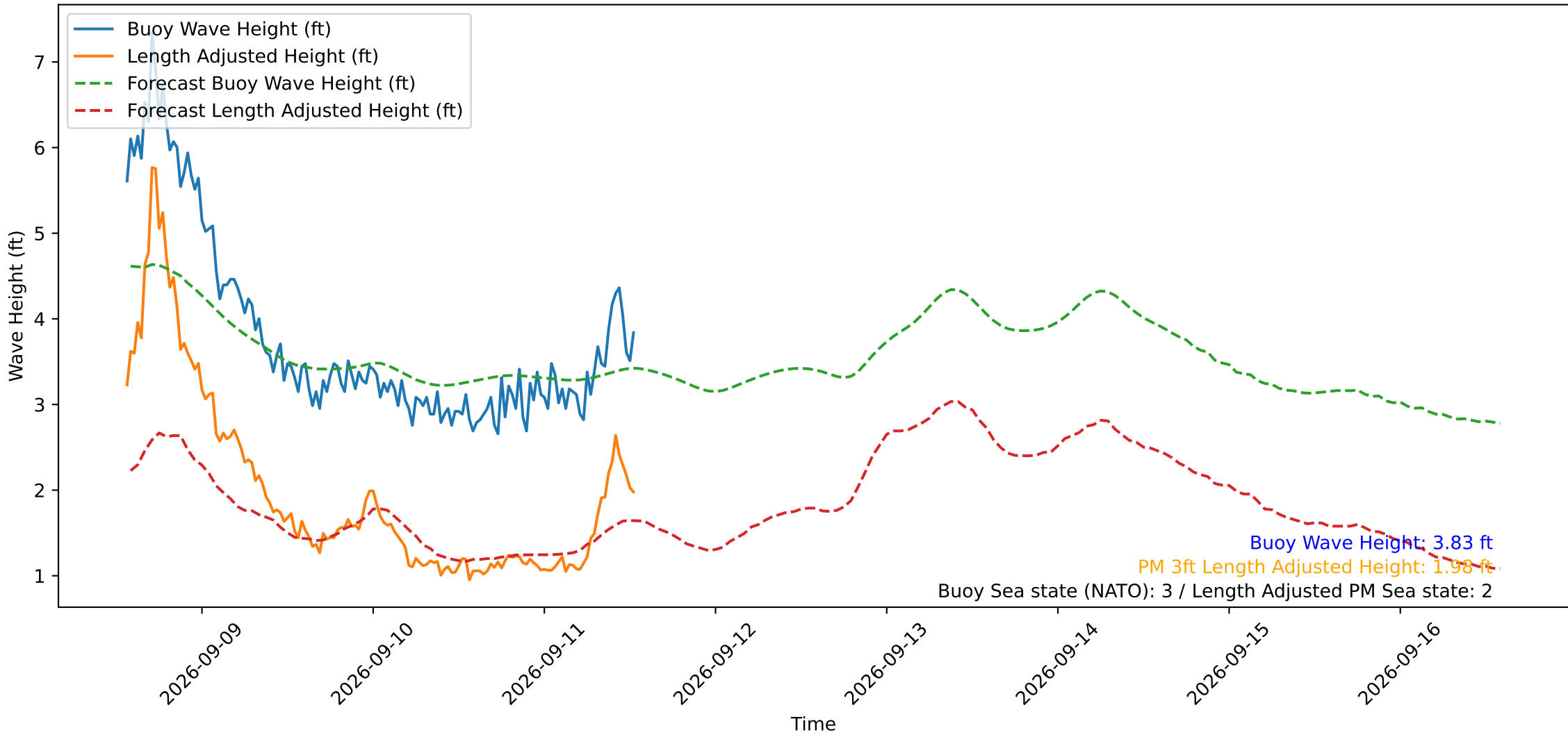
Wave Heights over Time for Oceanside Harbor at 2026-09-11 13:30:30
