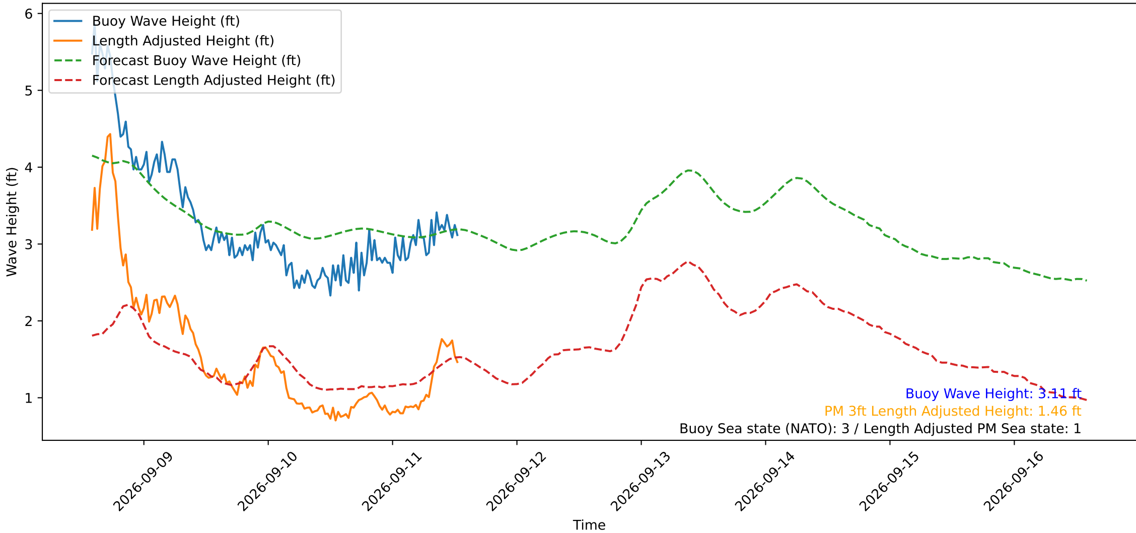
Wave Heights over Time for Red Beach at 2026-09-11 13:30:50
