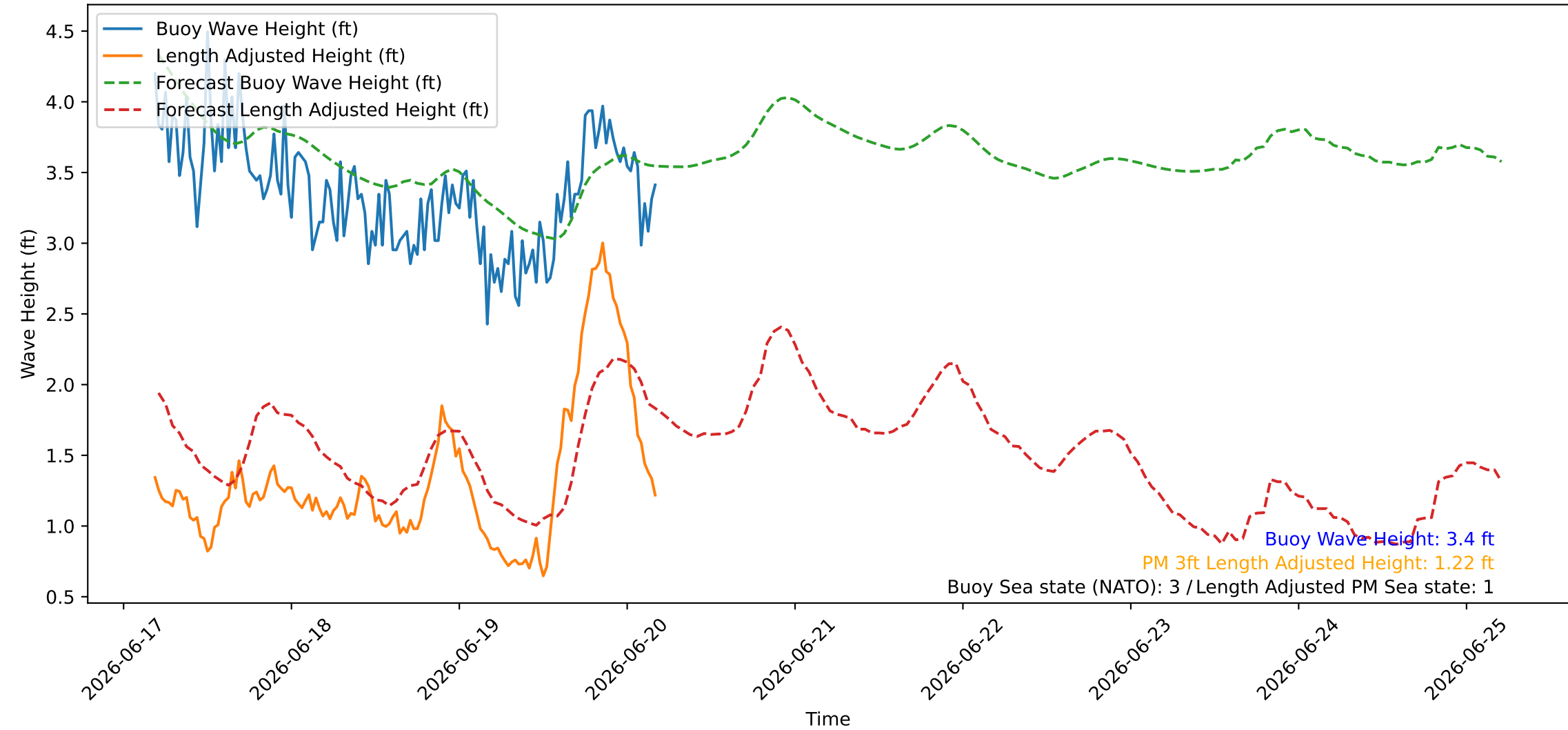
Wave Heights over Time for Green Beach at 2026-06-20 04:41:08
