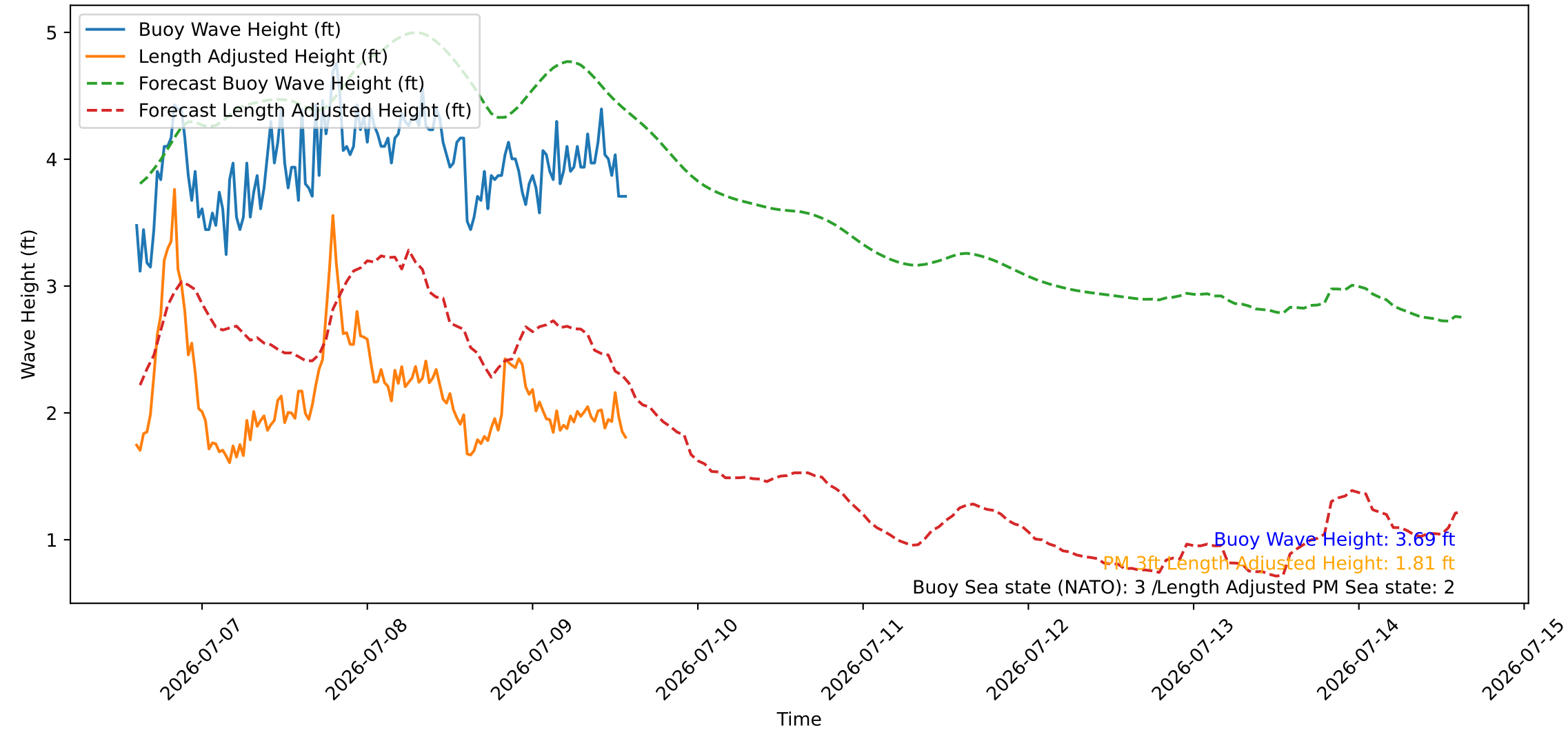
Wave Heights over Time for Green Beach at 2026-07-09 14:31:08
