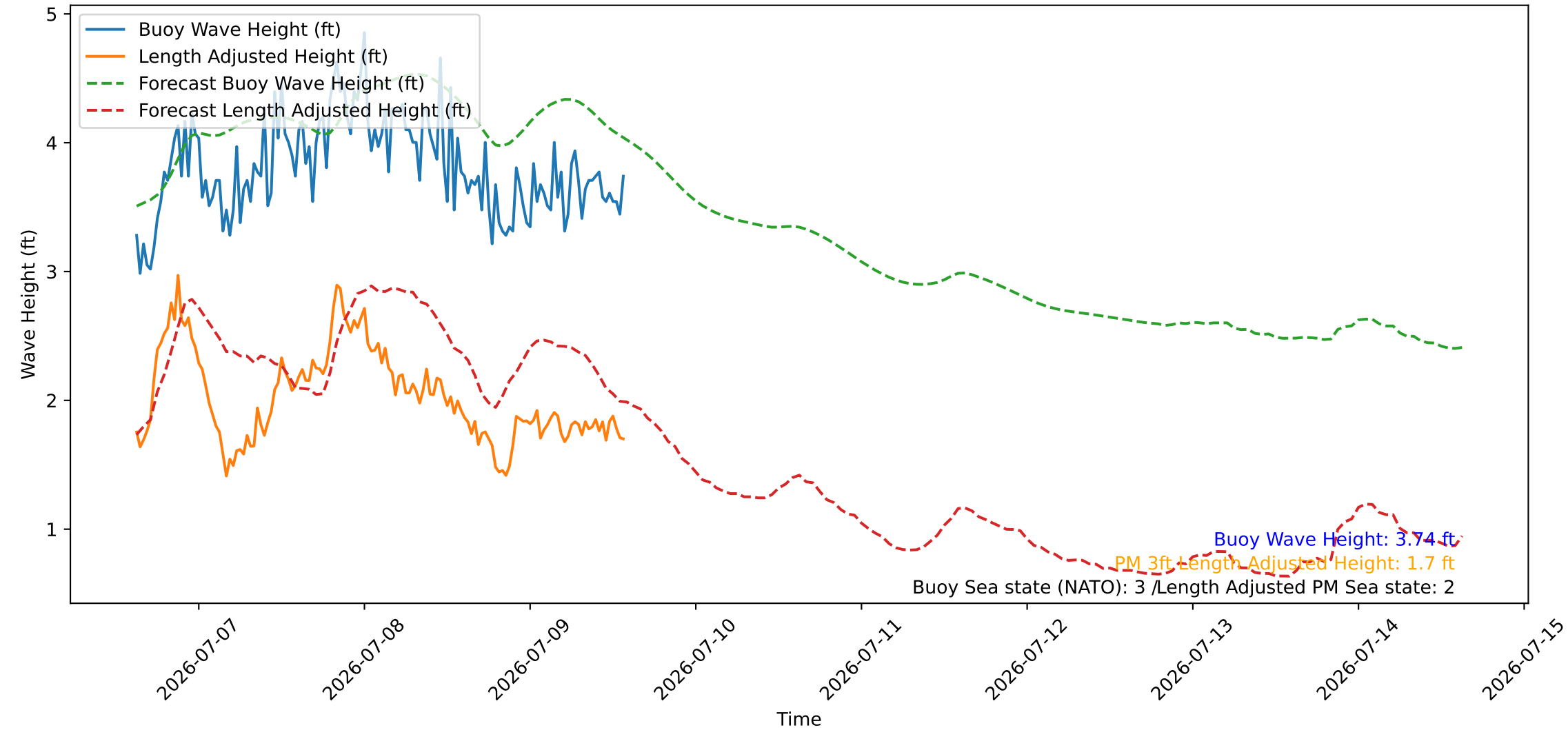
Wave Heights over Time for Red Beach at 2026-07-09 14:30:46
