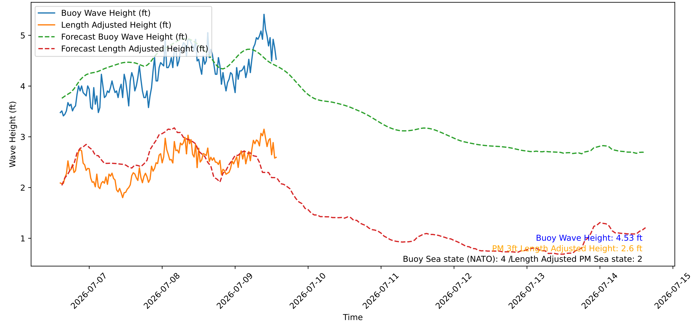
Wave Heights over Time for Oceanside Harbor at 2026-07-09 14:30:26
