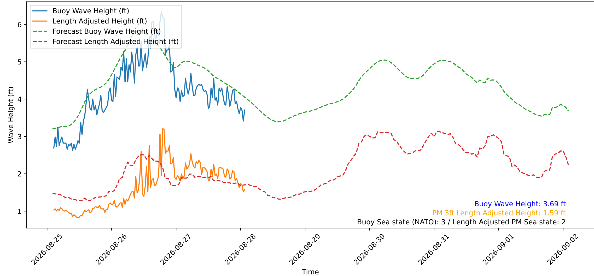
Wave Heights over Time for Green Beach at 2026-08-28 02:11:11
