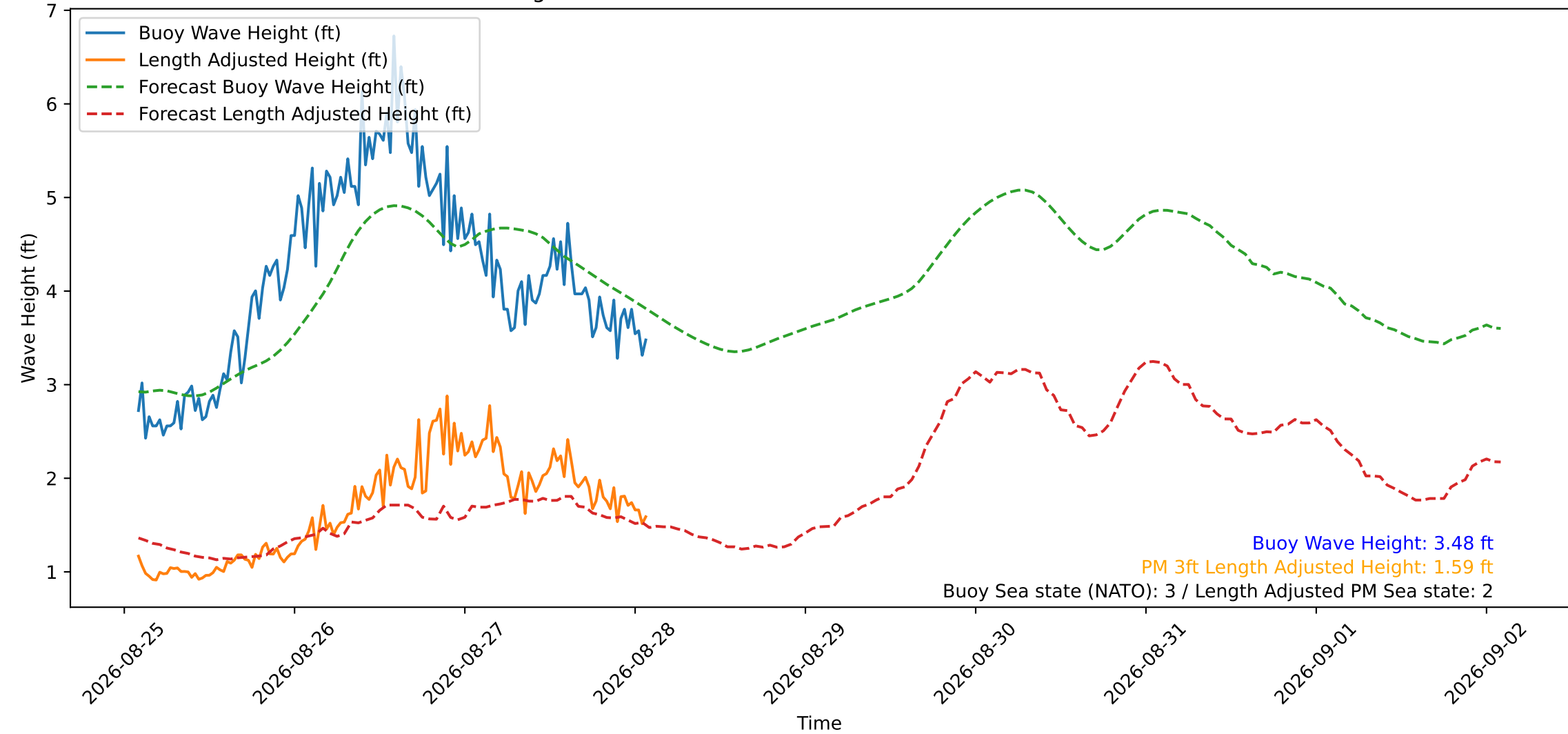
Wave Heights over Time for Oceanside Harbor at 2026-08-28 02:10:29
