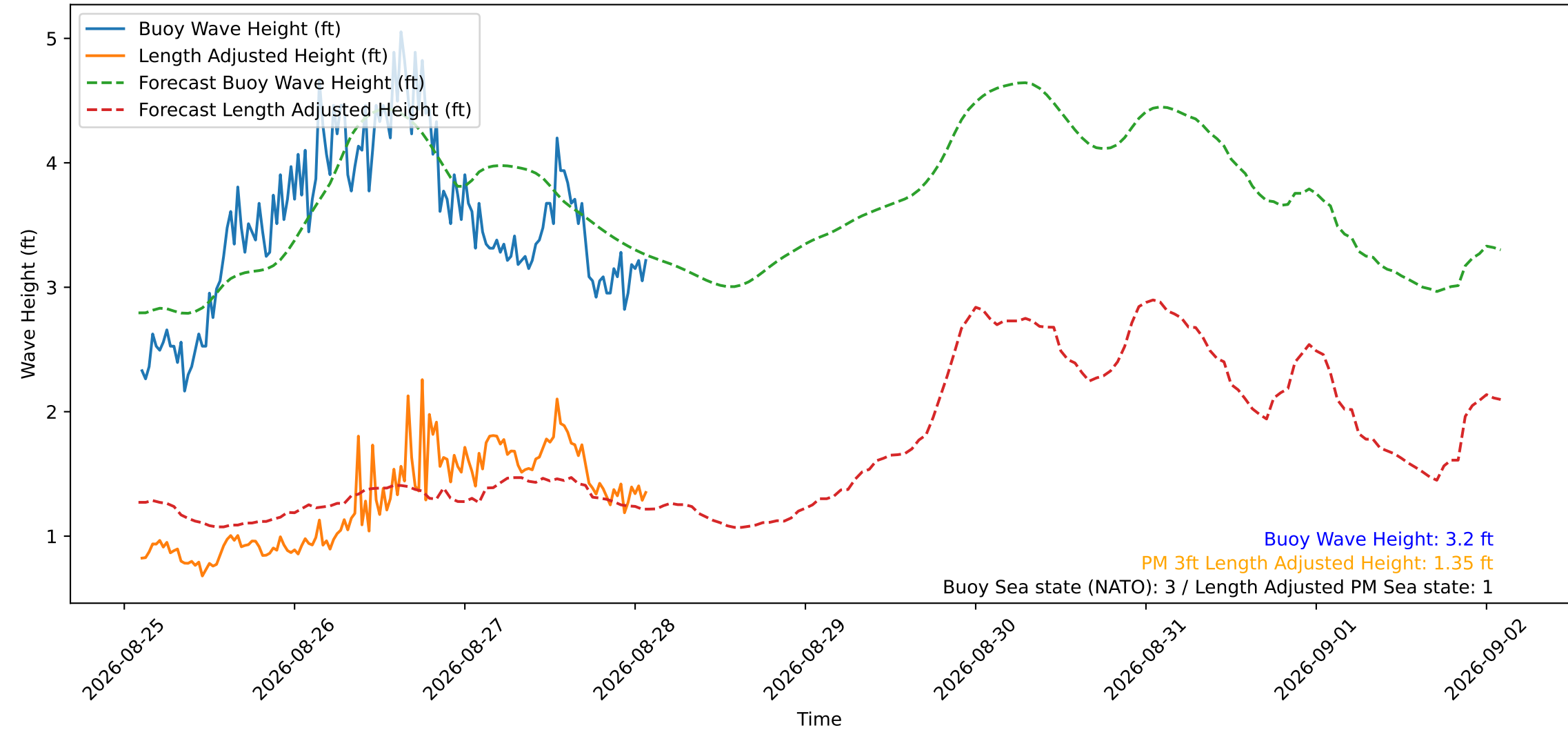
Wave Heights over Time for Red Beach at 2026-08-28 02:10:49
