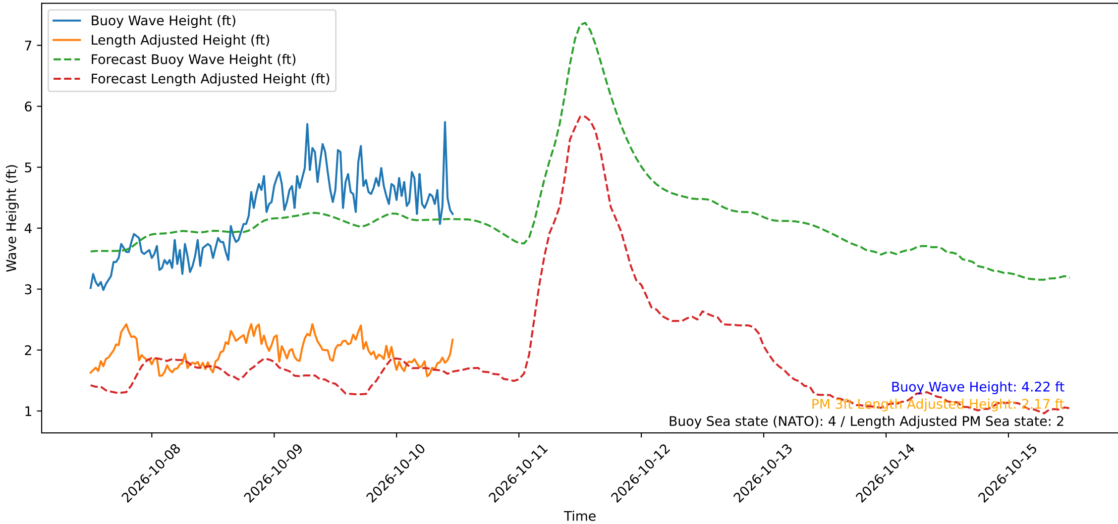
Wave Heights over Time for Red Beach at 2026-10-10 11:40:50
