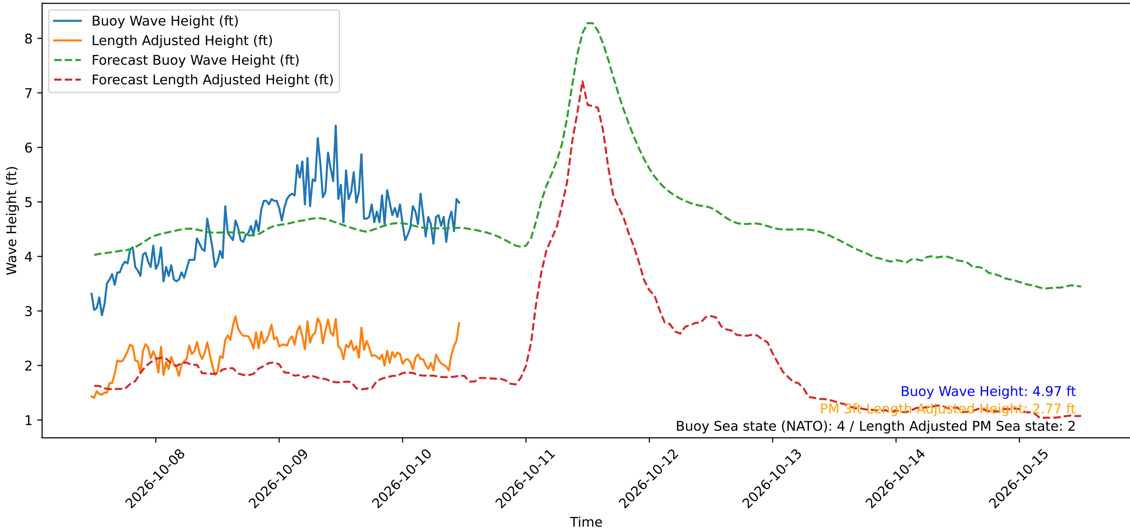
Wave Heights over Time for Oceanside Harbor at 2026-10-10 11:40:30
