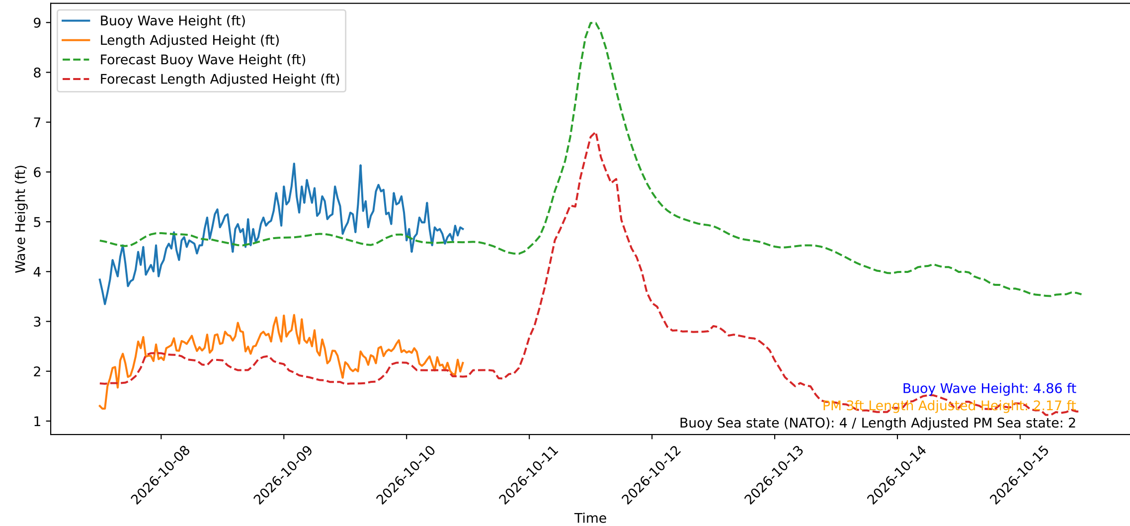
Wave Heights over Time for Green Beach at 2026-10-10 11:41:12
