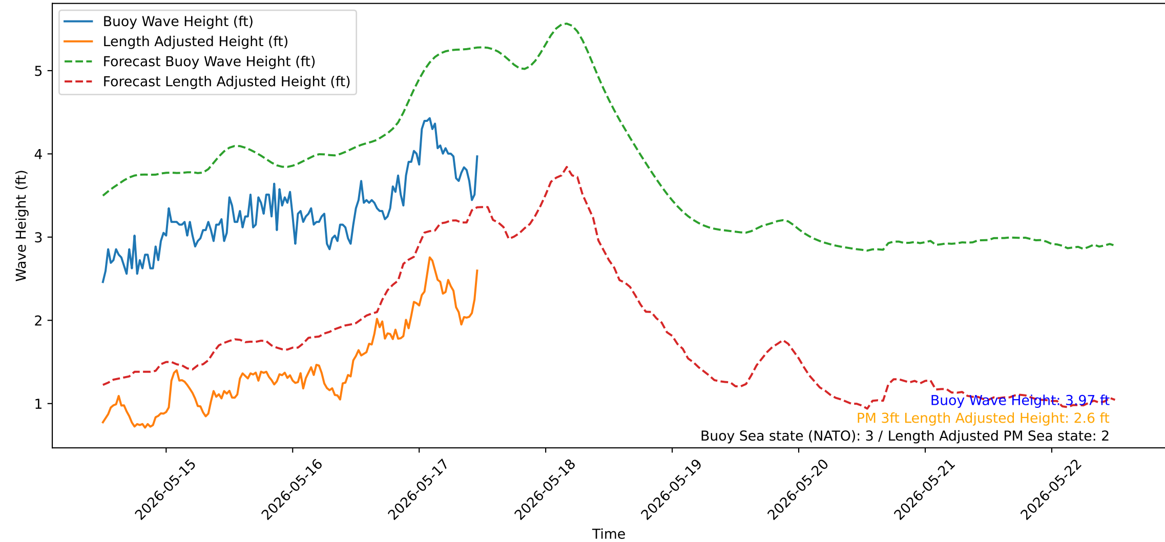
Wave Heights over Time for Green Beach at 2026-05-17 11:51:13
