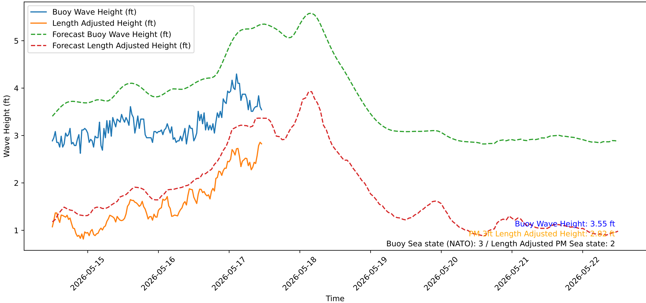
Wave Heights over Time for Oceanside Harbor at 2026-05-17 11:50:31
