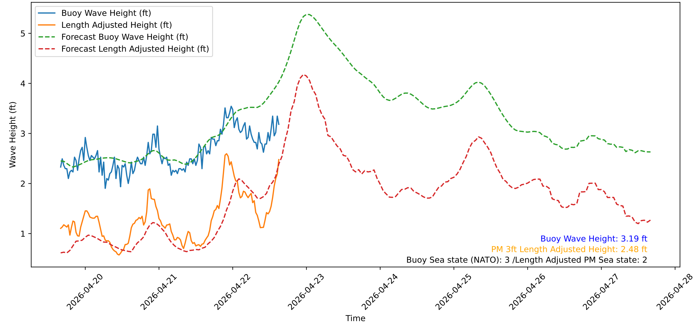
Wave Heights over Time for Green Beach at 2026-04-22 16:11:12
