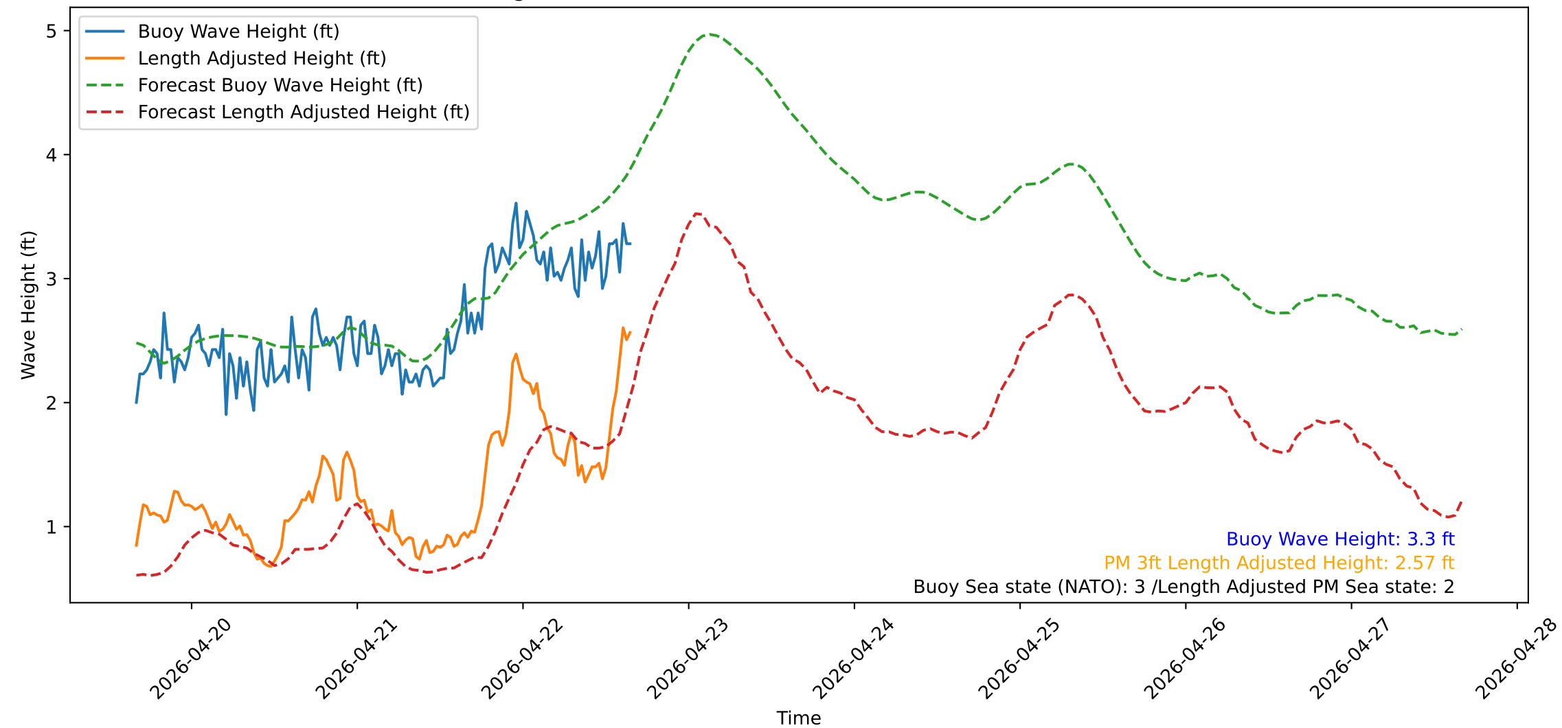
Wave Heights over Time for Oceanside Harbor at 2026-04-22 16:10:31
