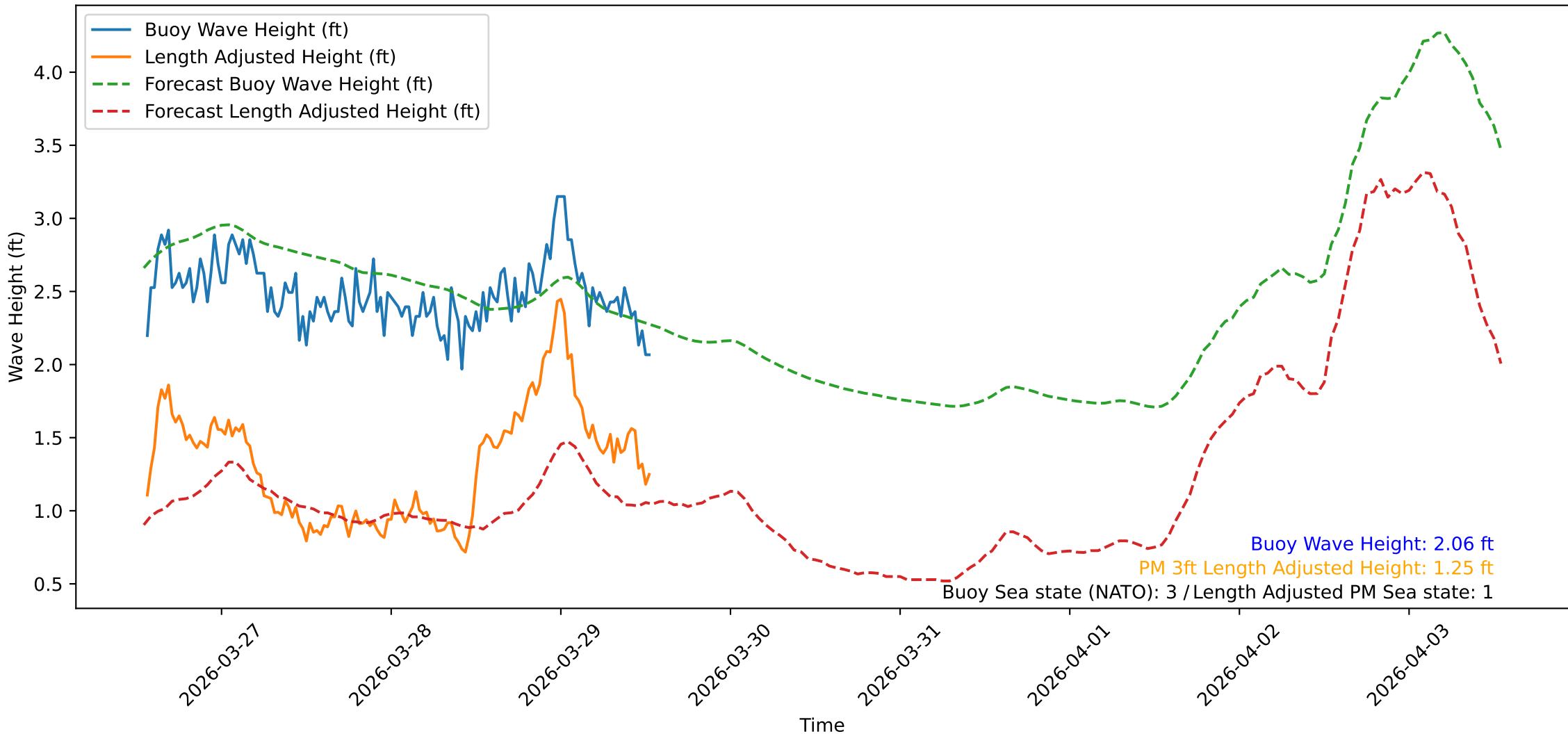
Wave Heights over Time for Oceanside Harbor at 2026-03-29 13:20:32
