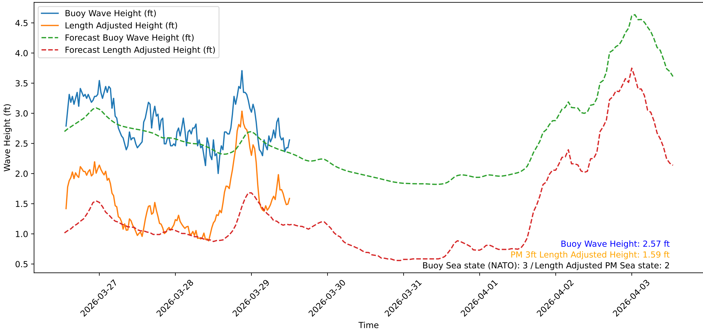
Wave Heights over Time for Green Beach at 2026-03-29 13:21:10
