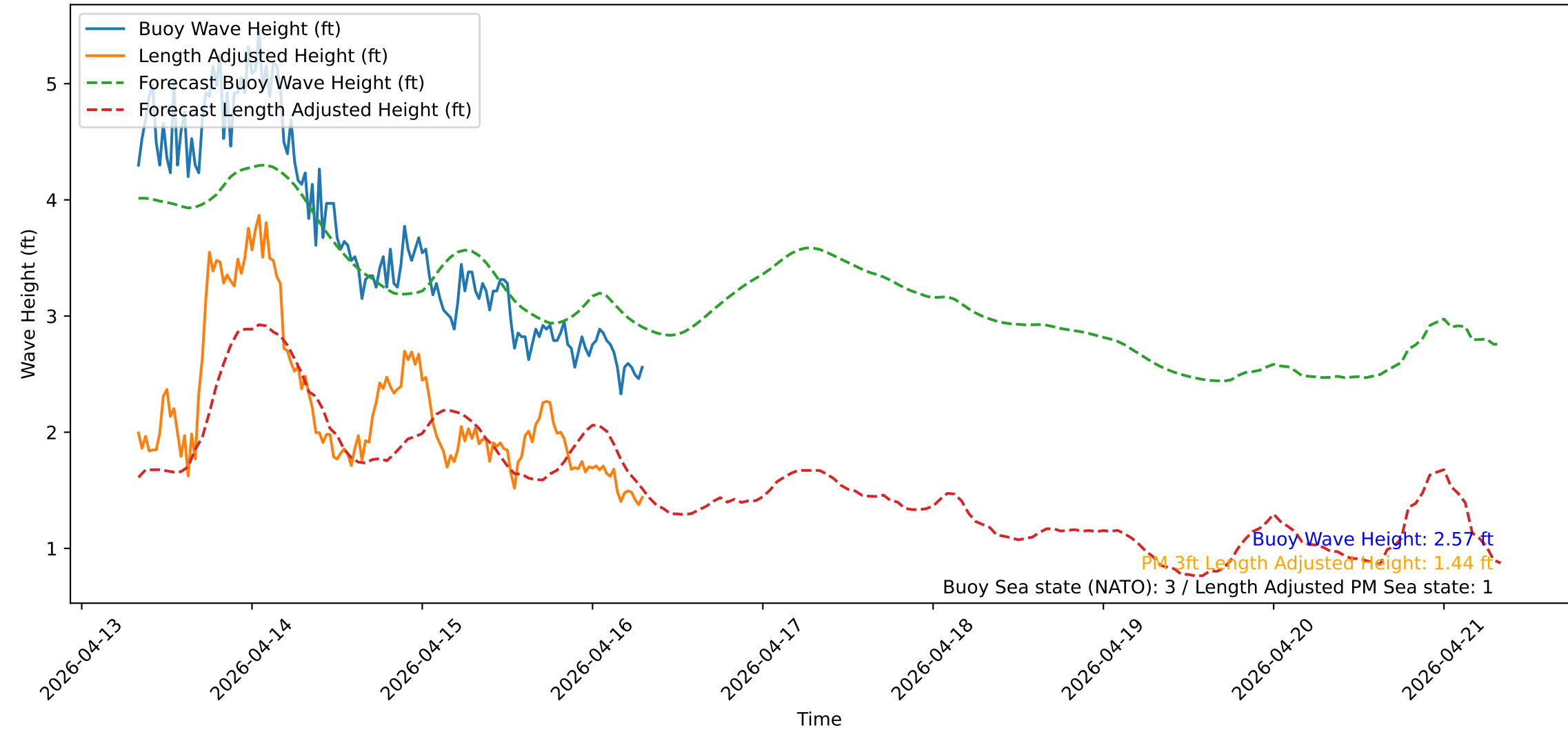
Wave Heights over Time for Oceanside Harbor at 2026-04-16 08:00:32
