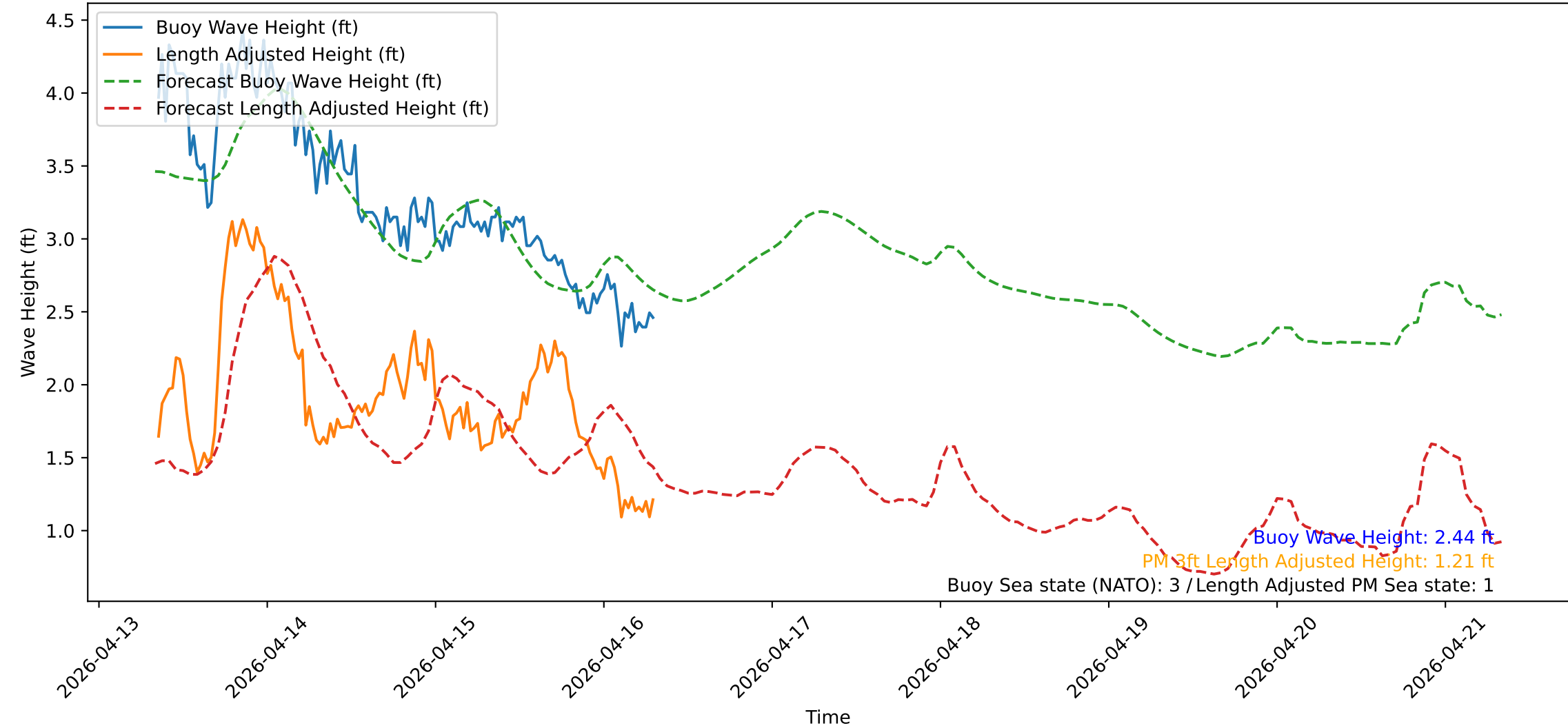
Wave Heights over Time for Red Beach at 2026-04-16 08:00:51
