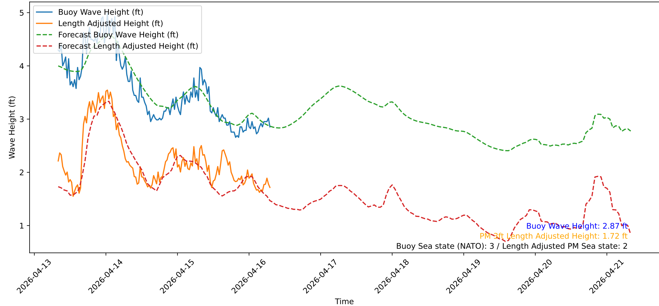
Wave Heights over Time for Green Beach at 2026-04-16 08:01:13
