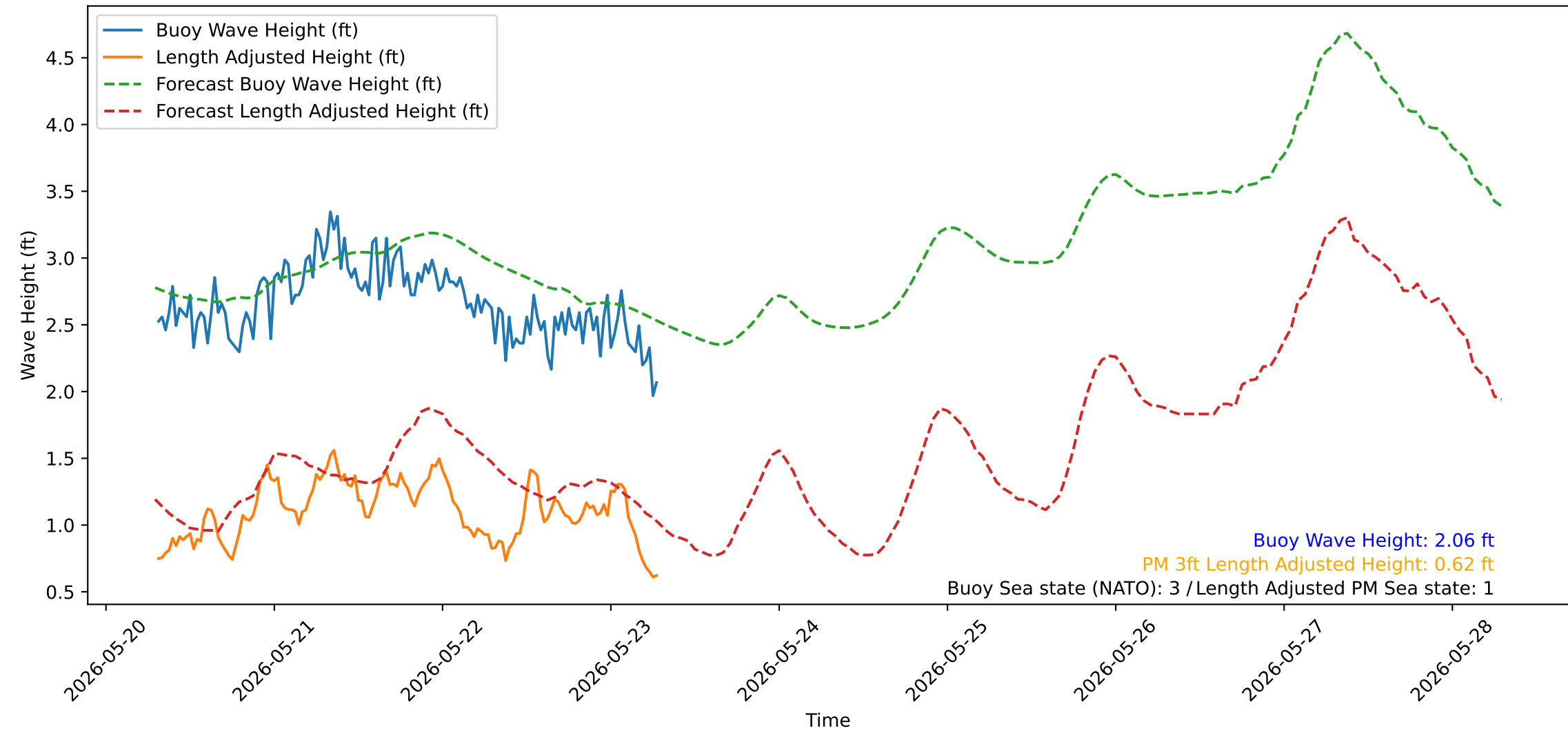
Wave Heights over Time for Red Beach at 2026-05-23 07:10:51
