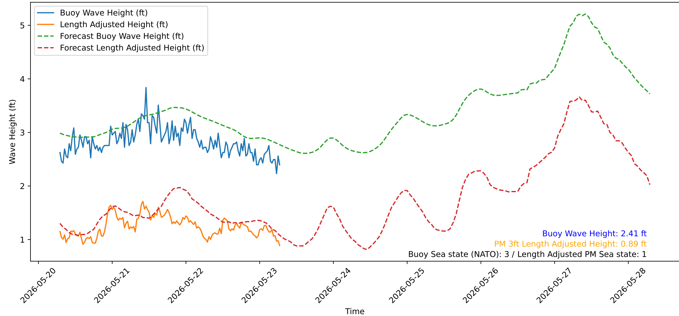
Wave Heights over Time for Oceanside Harbor at 2026-05-23 07:10:31
