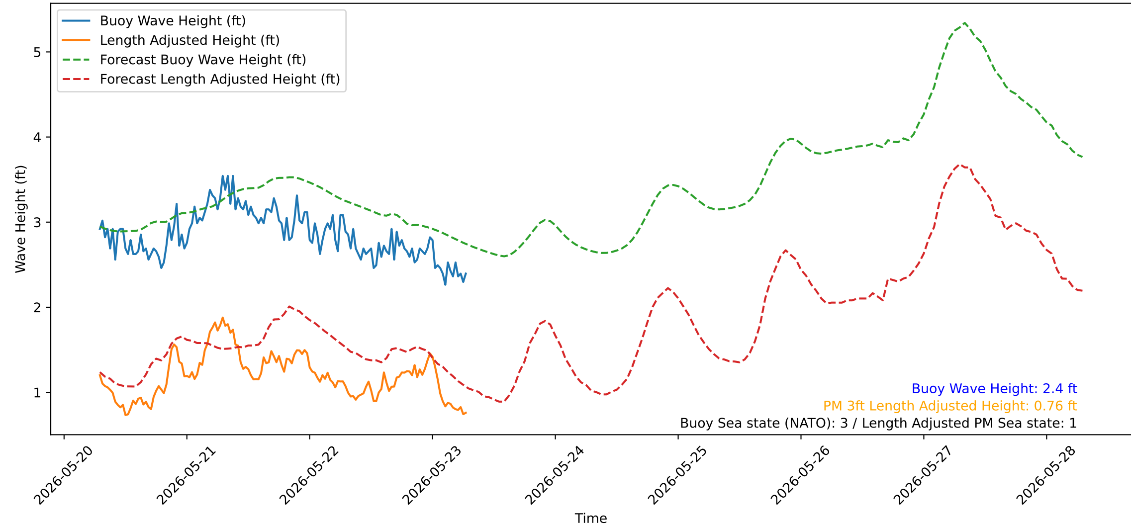
Wave Heights over Time for Green Beach at 2026-05-23 07:11:13
