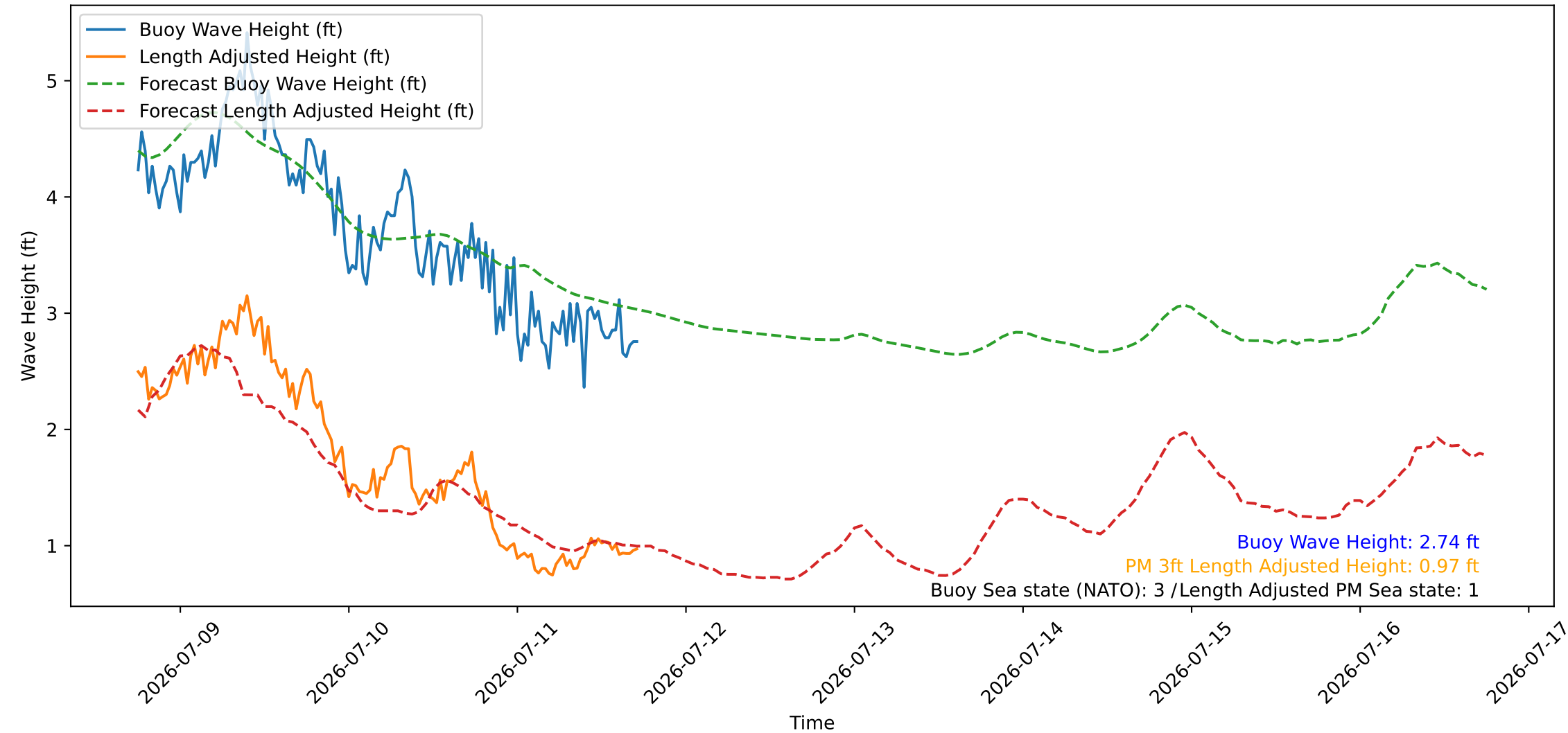
Wave Heights over Time for Oceanside Harbor at 2026-07-11 17:50:27
