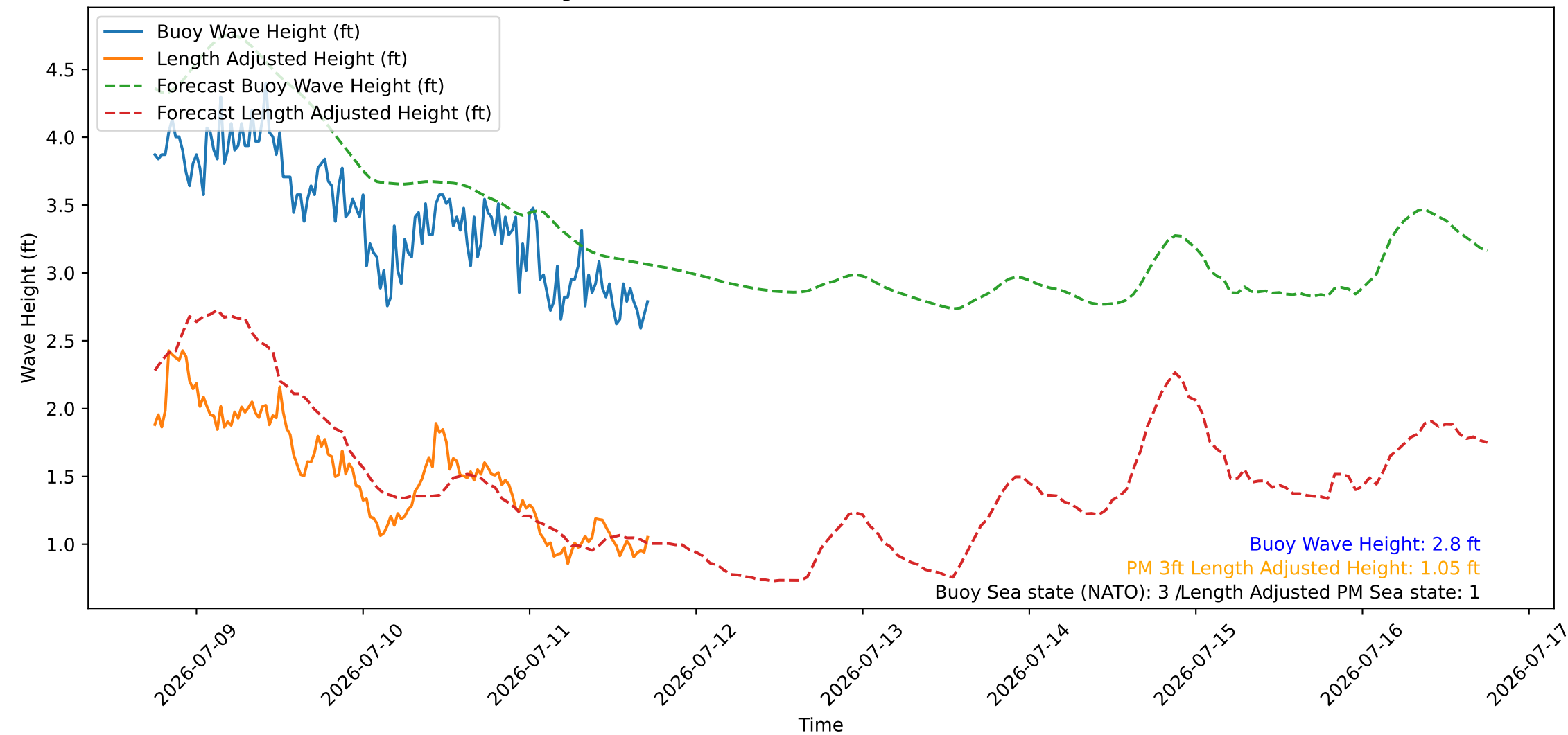
Wave Heights over Time for Green Beach at 2026-07-11 17:51:11
