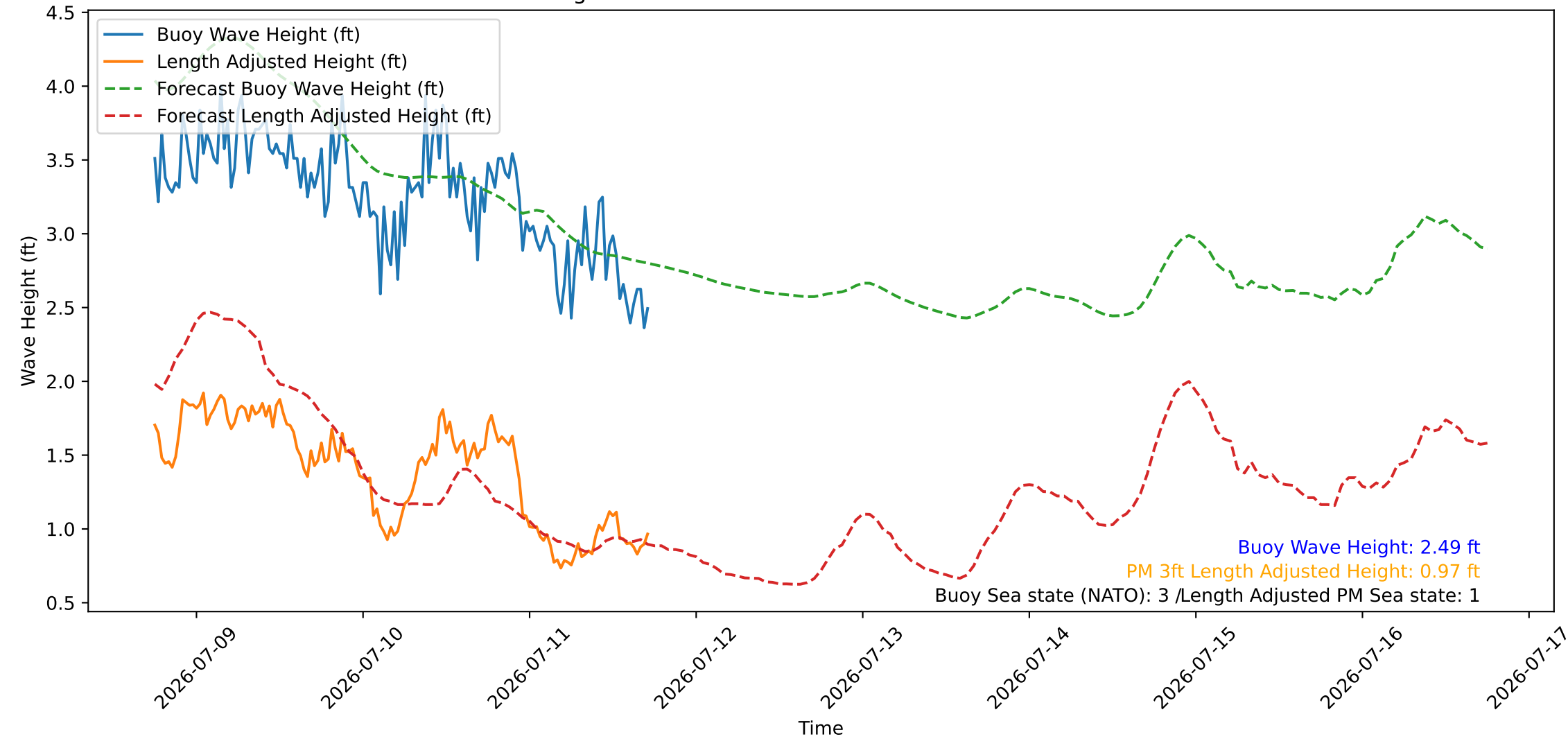
Wave Heights over Time for Red Beach at 2026-07-11 17:50:48
