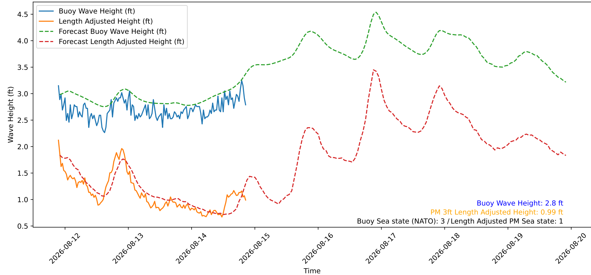
Wave Heights over Time for Green Beach at 2026-08-14 21:31:08
