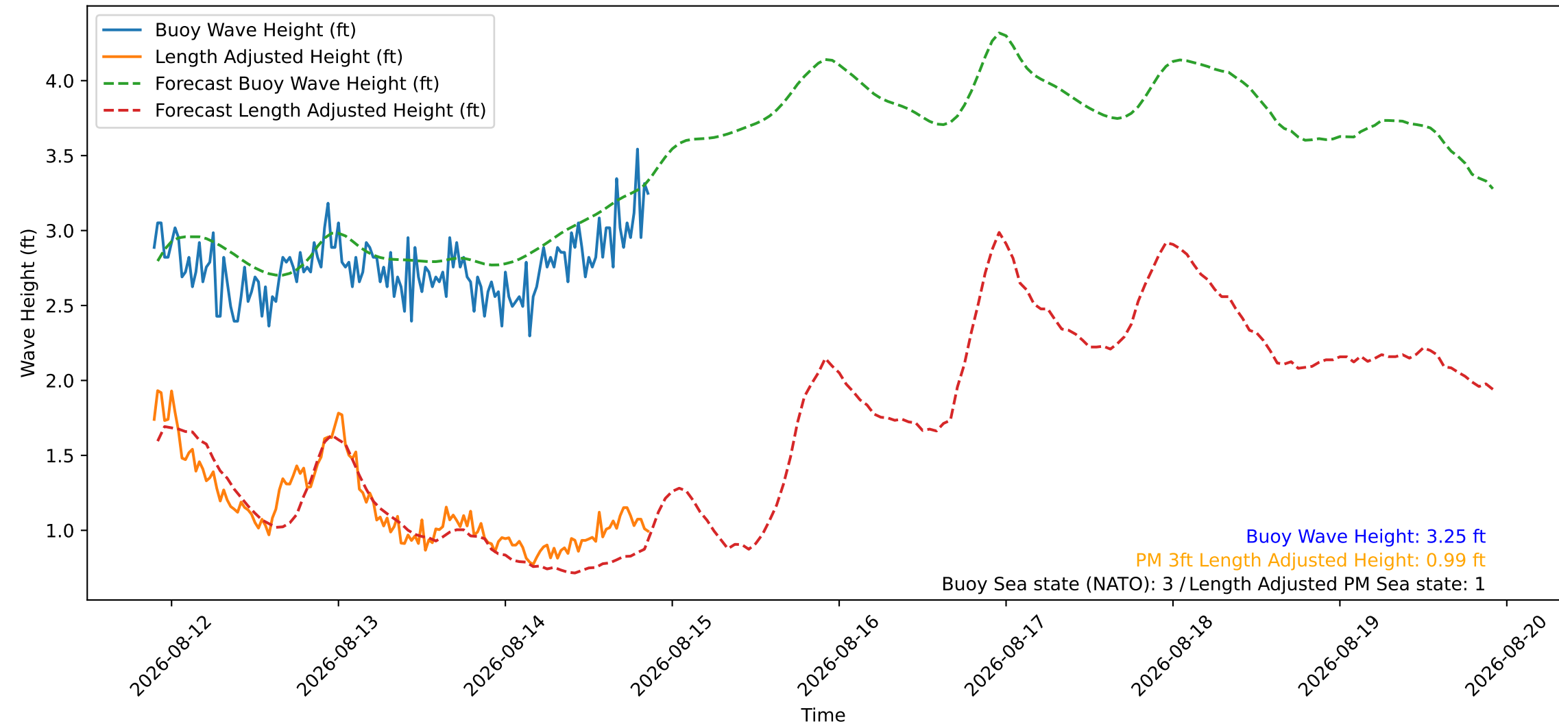
Wave Heights over Time for Oceanside Harbor at 2026-08-14 21:30:26
