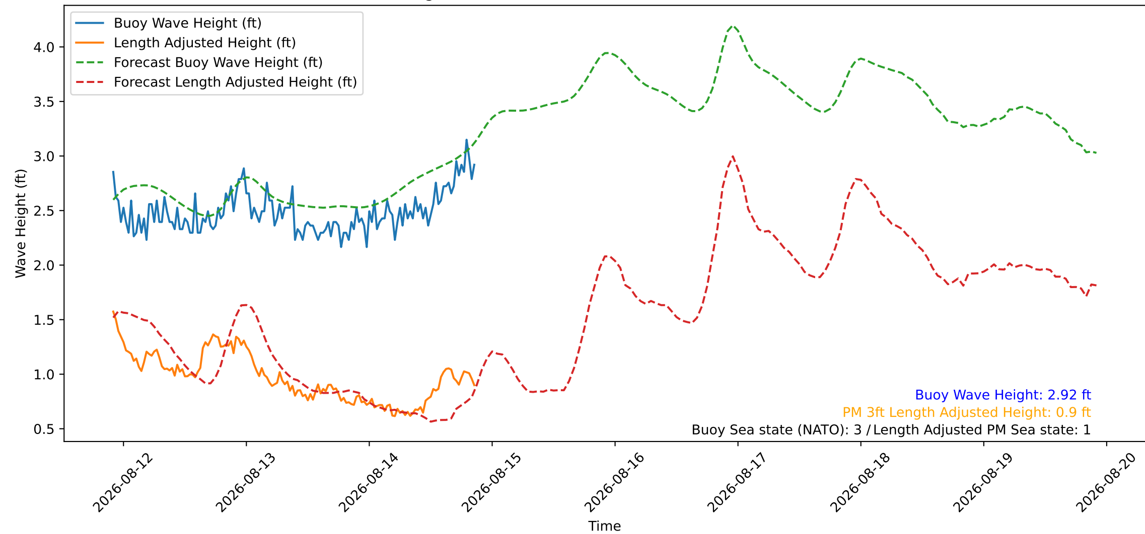
Wave Heights over Time for Red Beach at 2026-08-14 21:30:46
