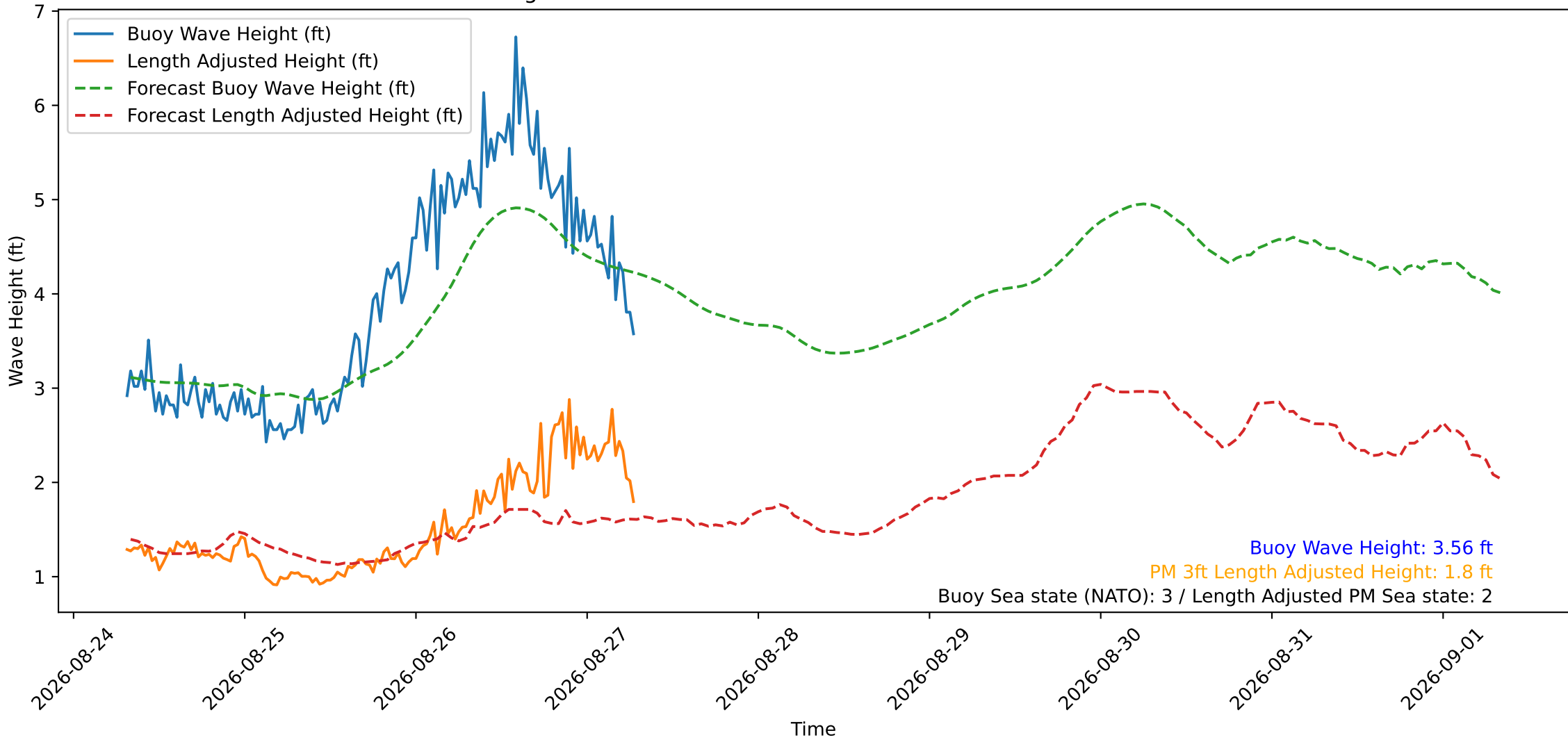
Wave Heights over Time for Oceanside Harbor at 2026-08-27 07:30:29
