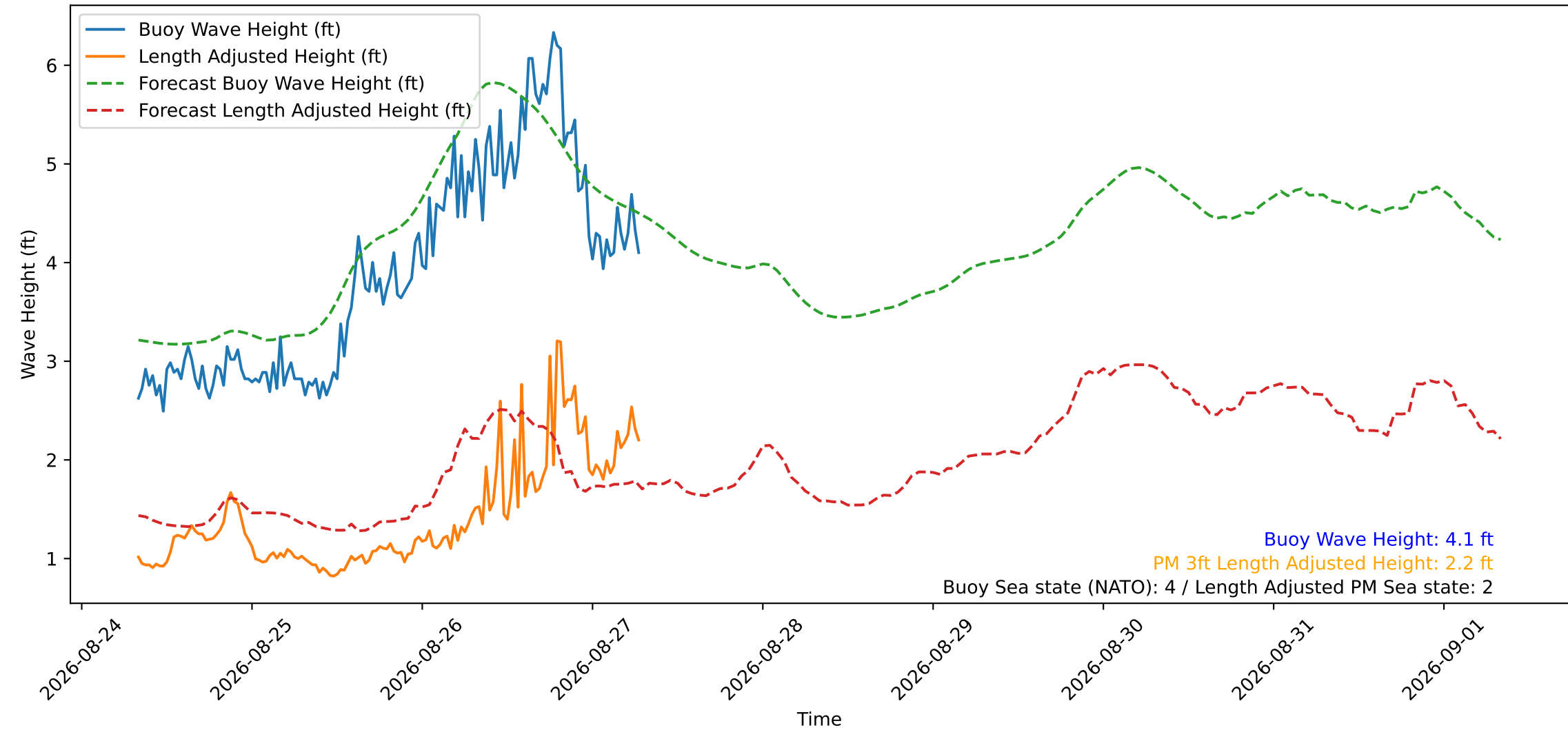
Wave Heights over Time for Green Beach at 2026-08-27 07:31:12
