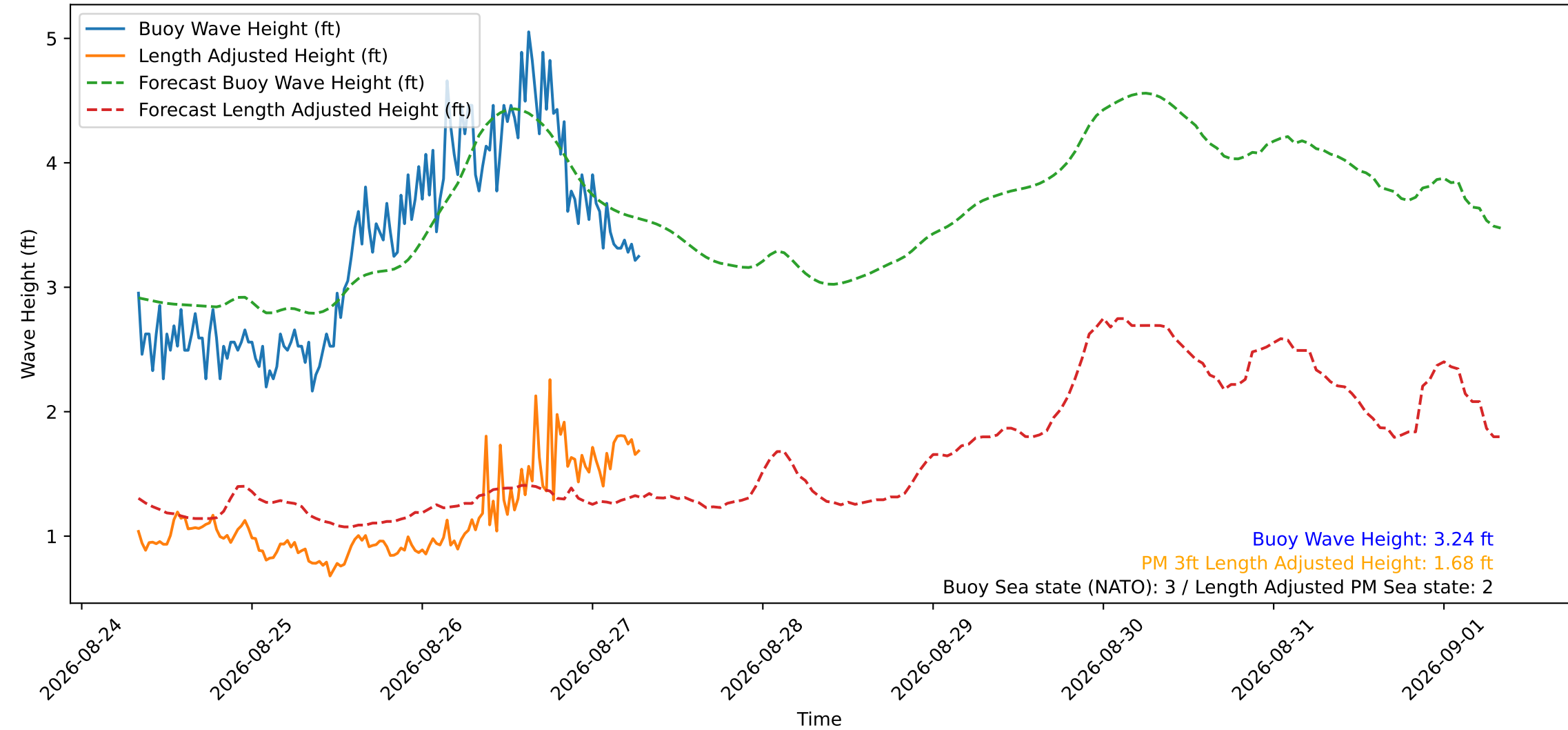
Wave Heights over Time for Red Beach at 2026-08-27 07:30:49
