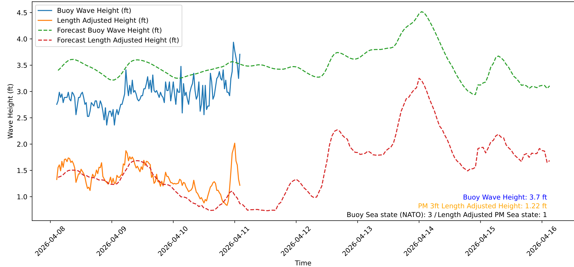
Wave Heights over Time for Green Beach at 2026-04-11 02:41:13
