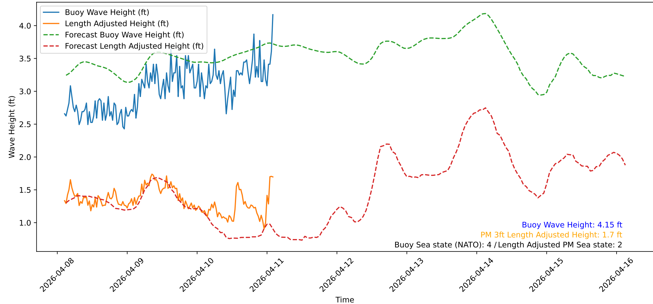
Wave Heights over Time for Oceanside Harbor at 2026-04-11 02:40:32
