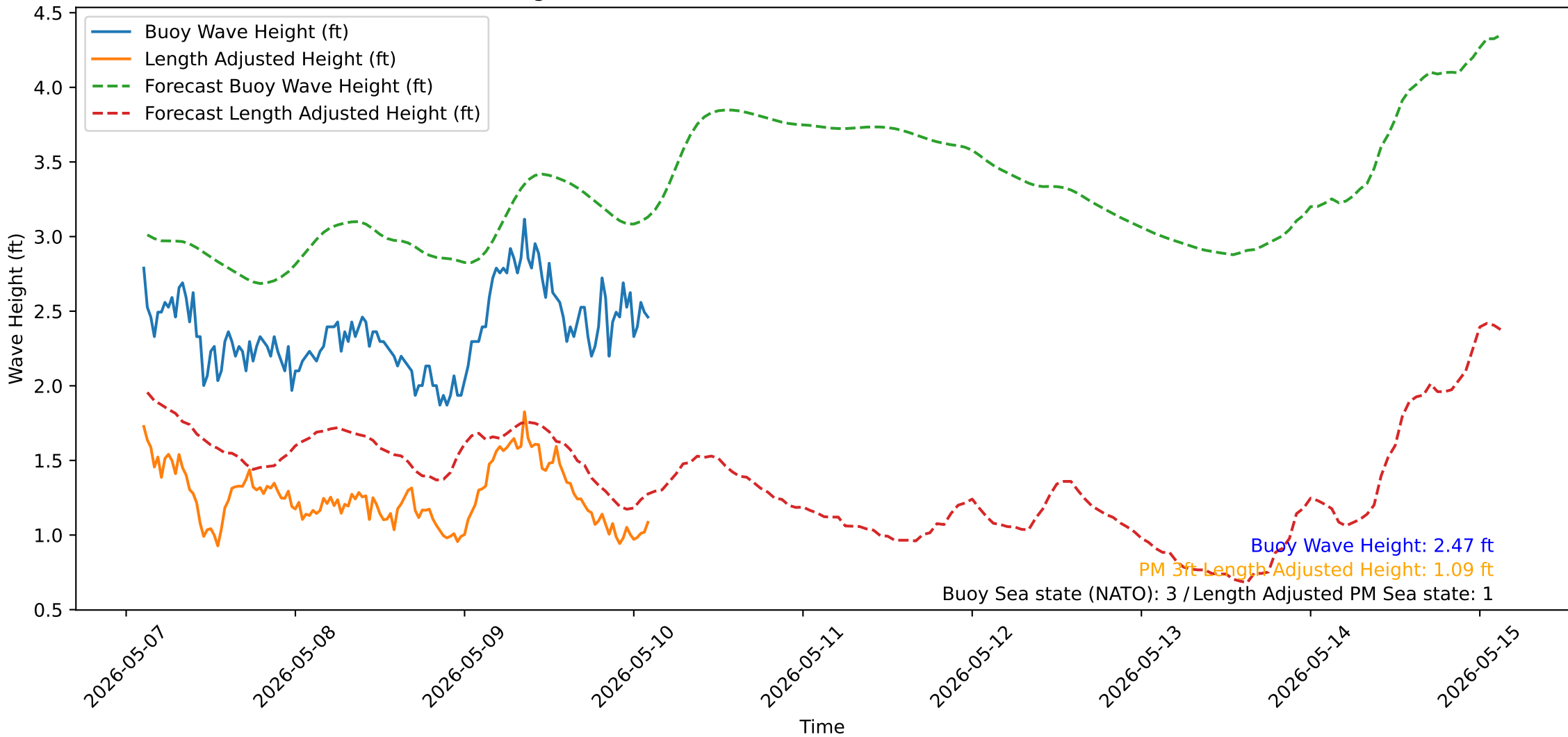
Wave Heights over Time for Oceanside Harbor at 2026-05-10 02:30:31
