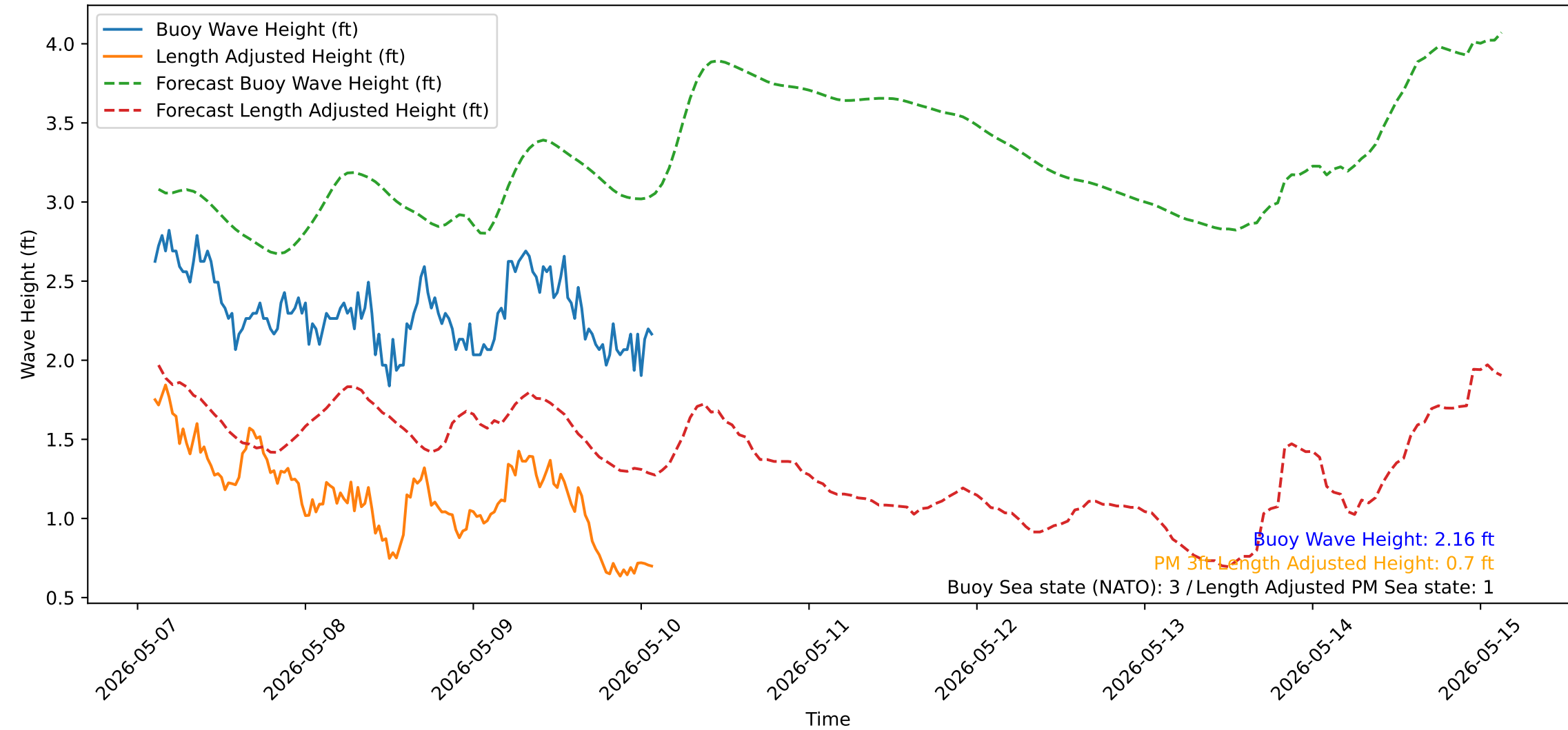
Wave Heights over Time for Green Beach at 2026-05-10 02:31:14
