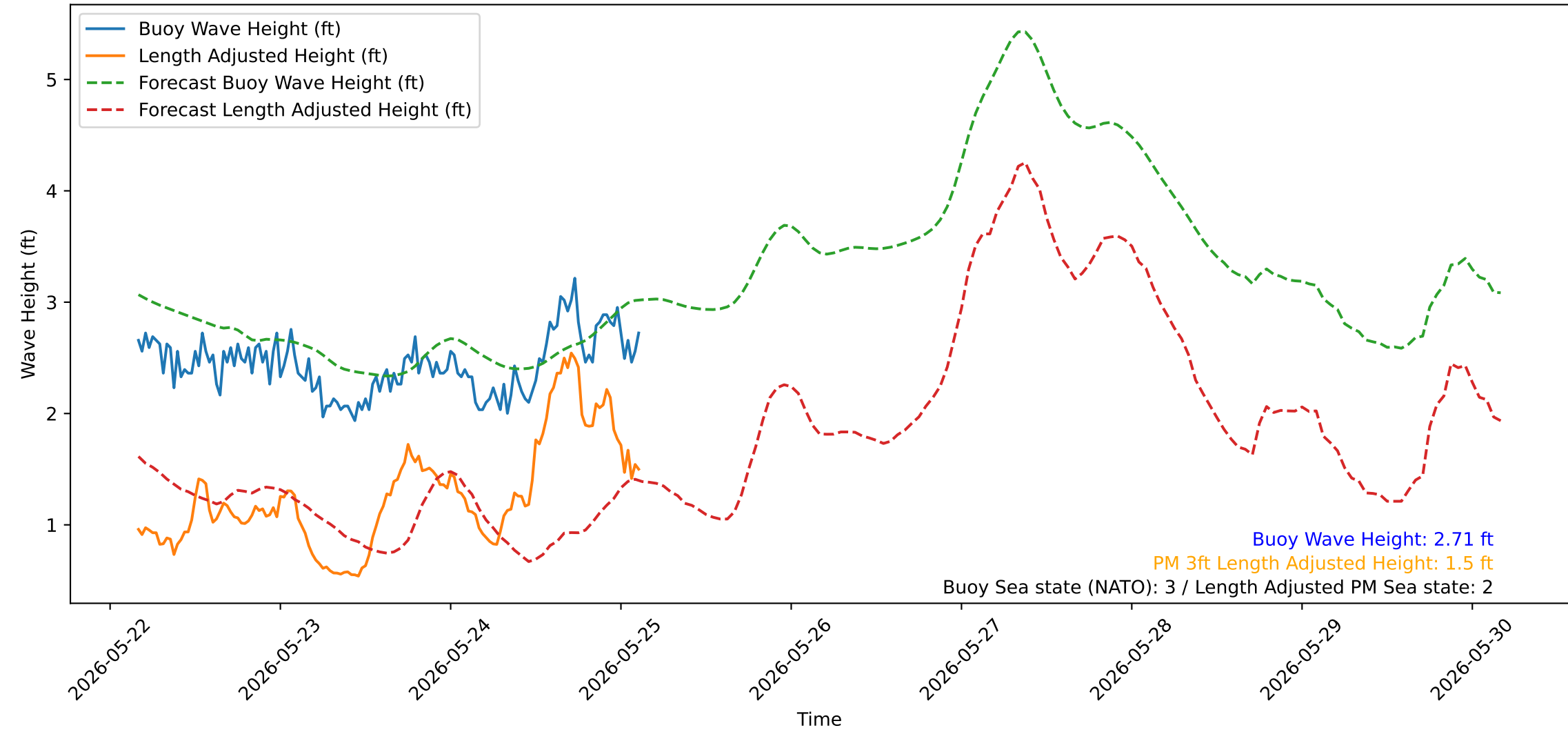
Wave Heights over Time for Red Beach at 2026-05-25 03:40:50
