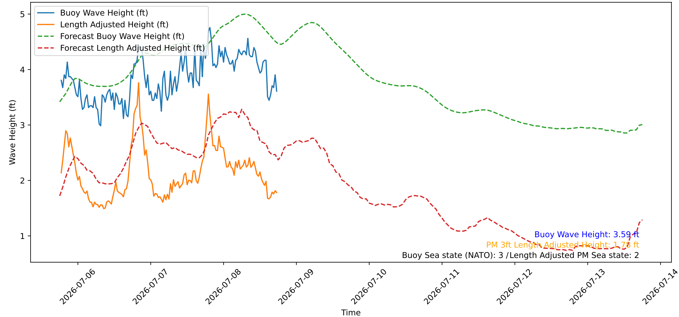
Wave Heights over Time for Green Beach at 2026-07-08 18:21:09
