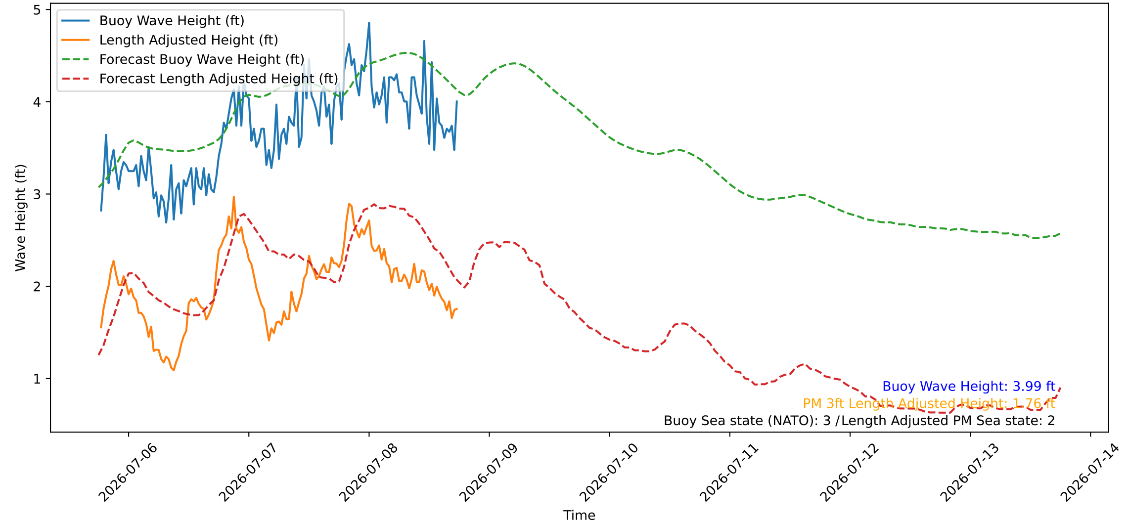
Wave Heights over Time for Red Beach at 2026-07-08 18:20:47
