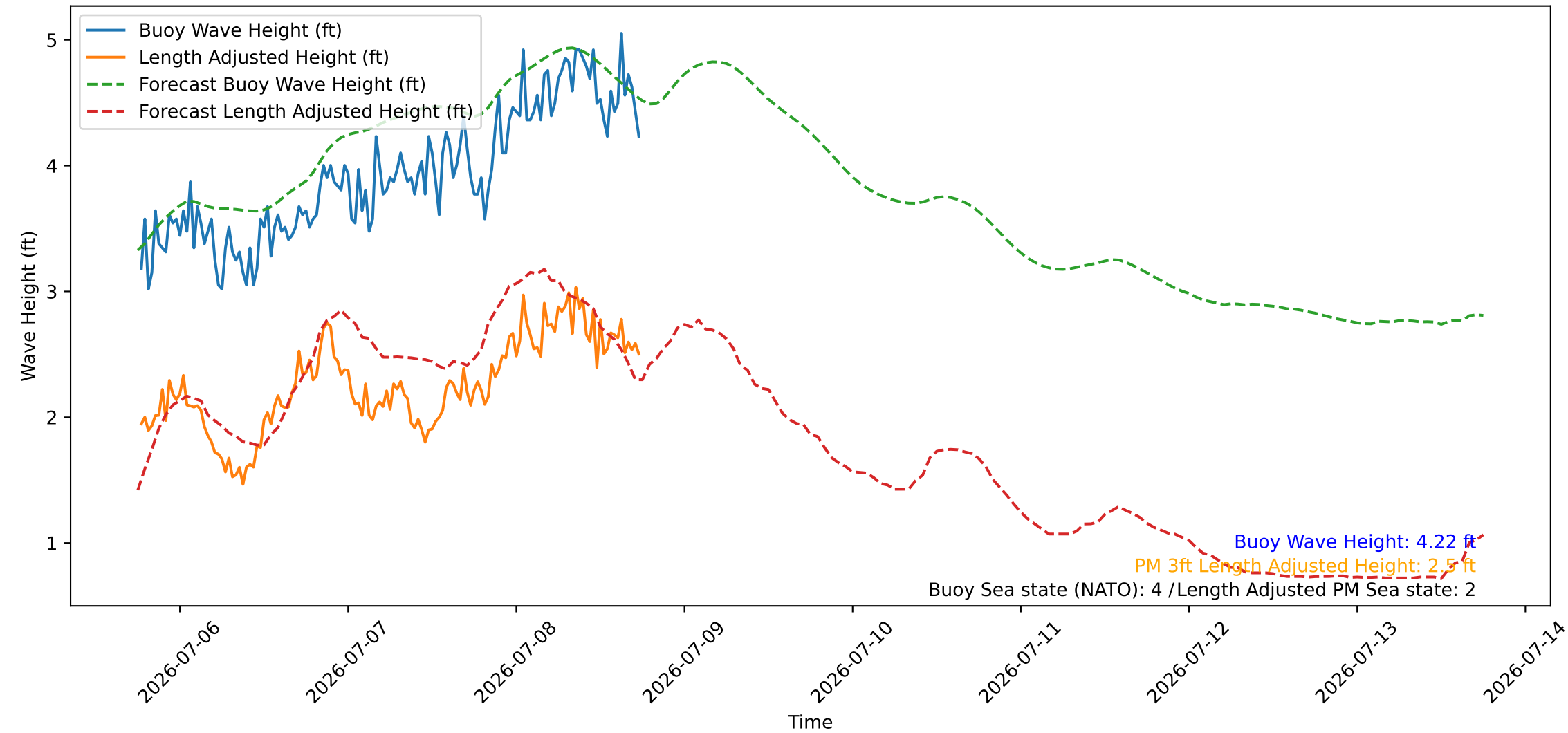
Wave Heights over Time for Oceanside Harbor at 2026-07-08 18:20:26
