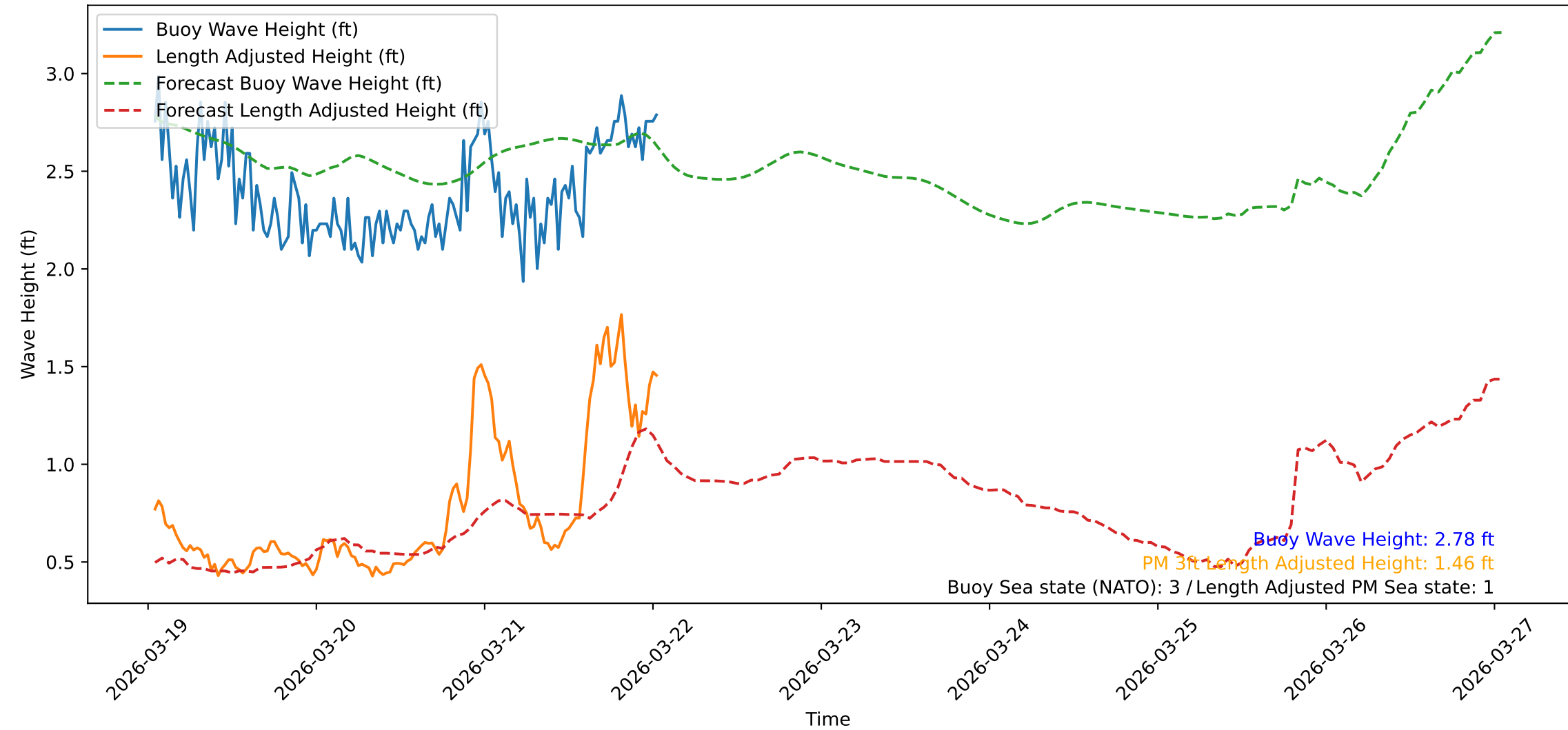
Wave Heights over Time for Green Beach at 2026-03-22 01:11:10
