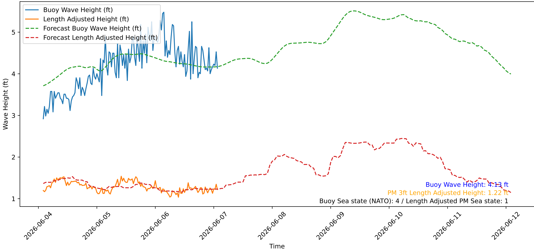
Wave Heights over Time for Oceanside Harbor at 2026-06-07 02:10:26
