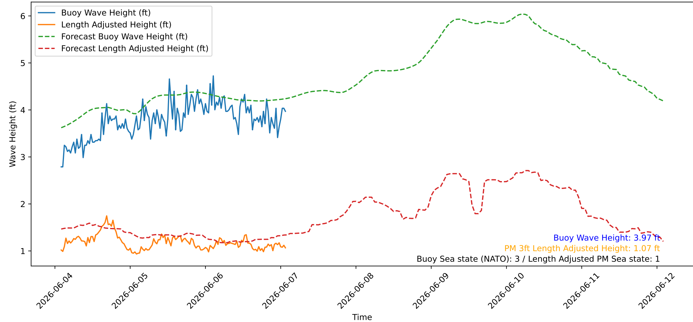
Wave Heights over Time for Green Beach at 2026-06-07 02:11:08
