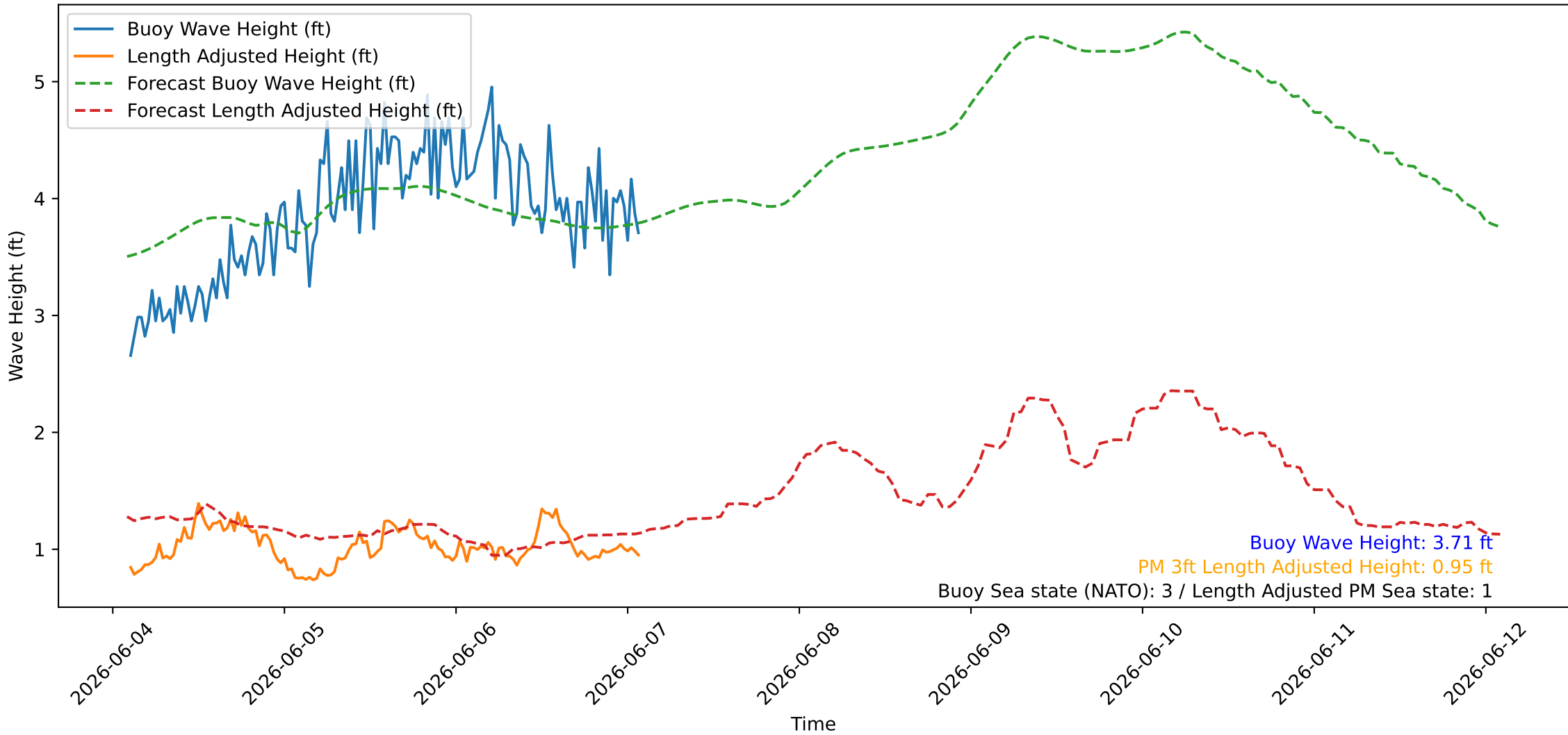
Wave Heights over Time for Red Beach at 2026-06-07 02:10:45
