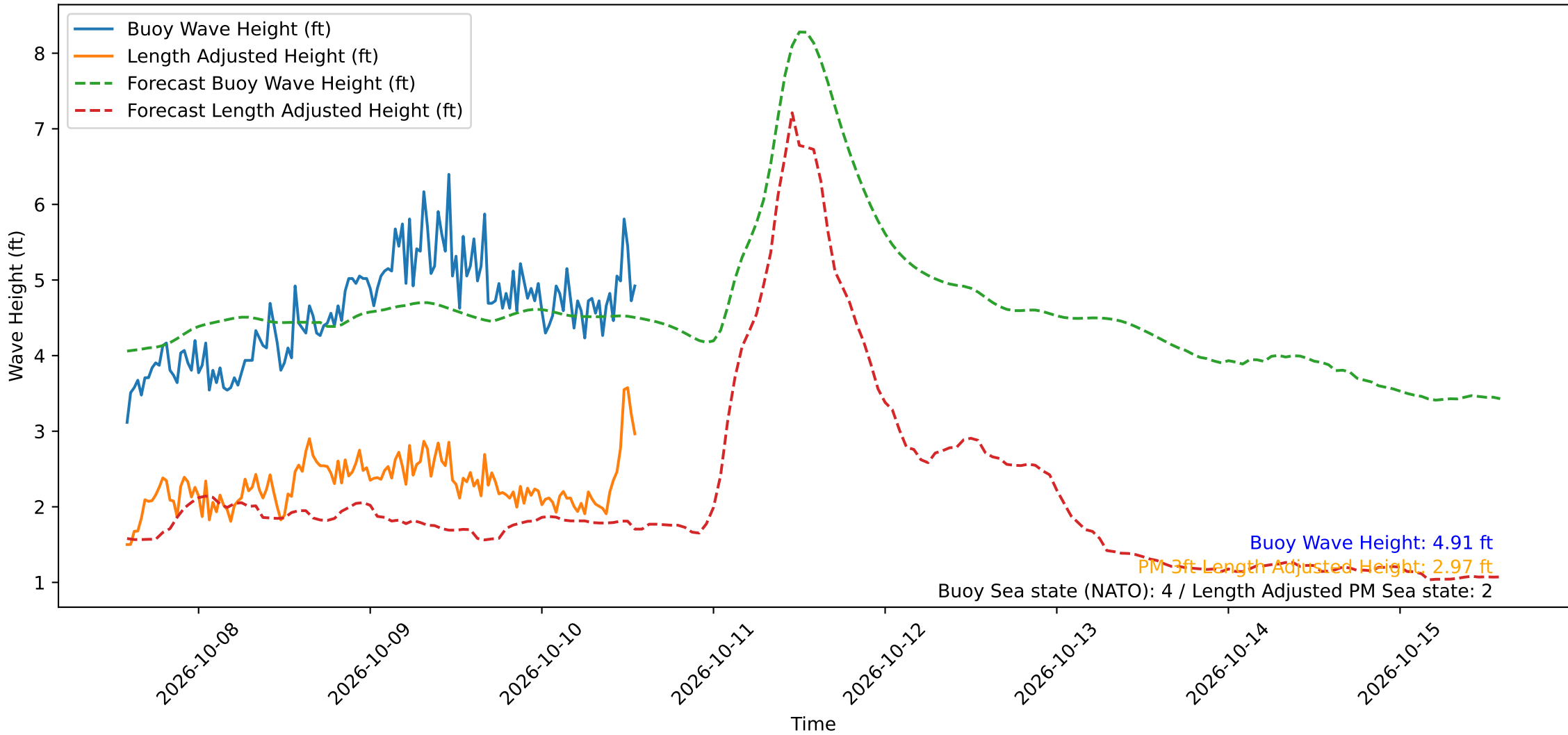
Wave Heights over Time for Oceanside Harbor at 2026-10-10 13:50:29
