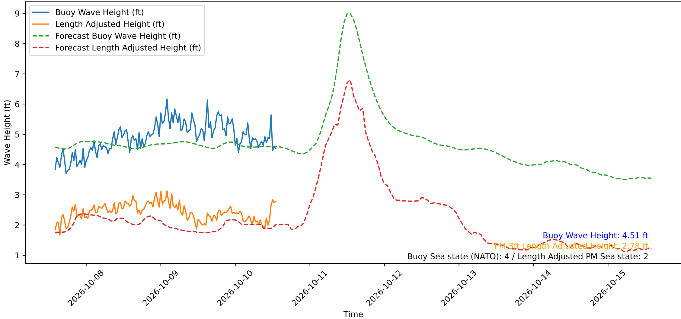
Wave Heights over Time for Green Beach at 2026-10-10 13:51:13
