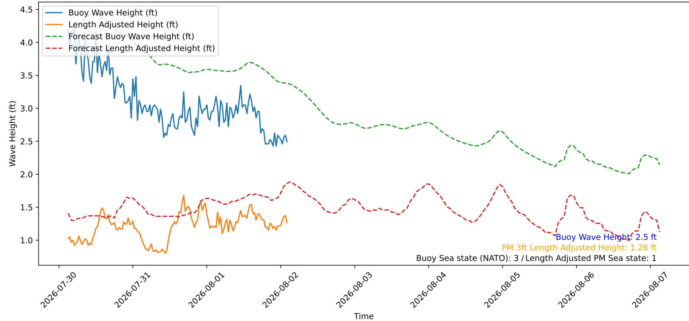
Wave Heights over Time for Red Beach at 2026-08-02 02:40:46
