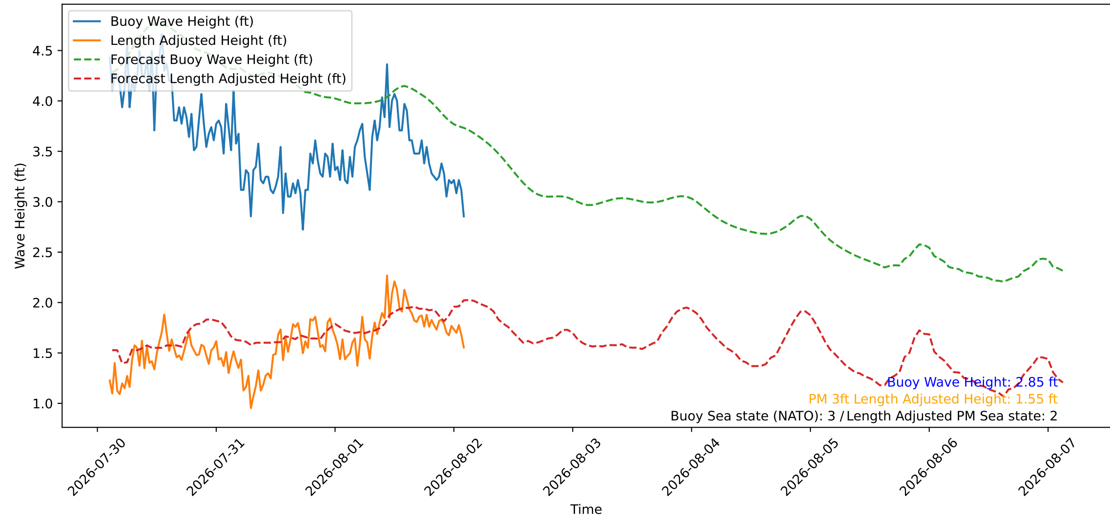
Wave Heights over Time for Oceanside Harbor at 2026-08-02 02:40:26
