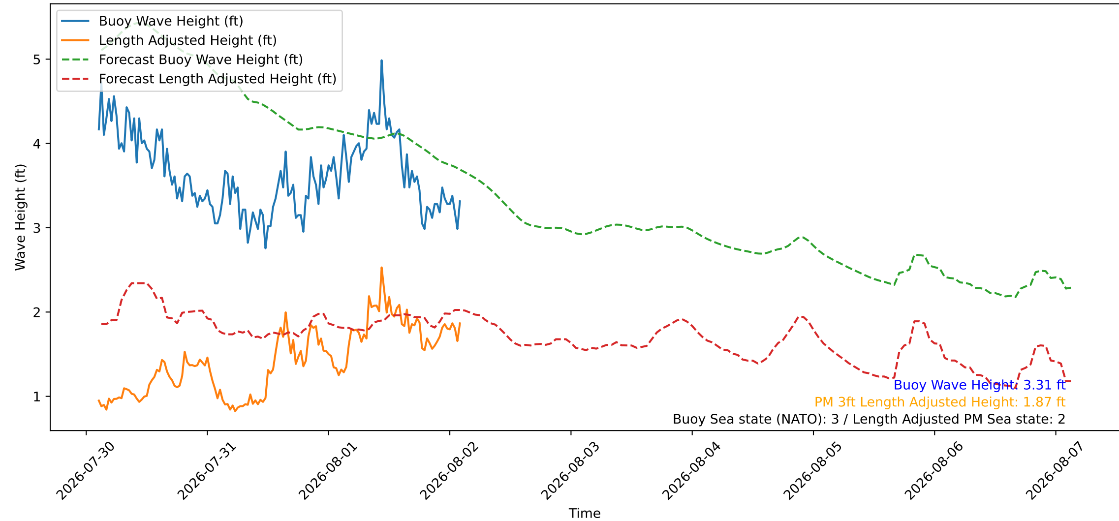
Wave Heights over Time for Green Beach at 2026-08-02 02:41:08
