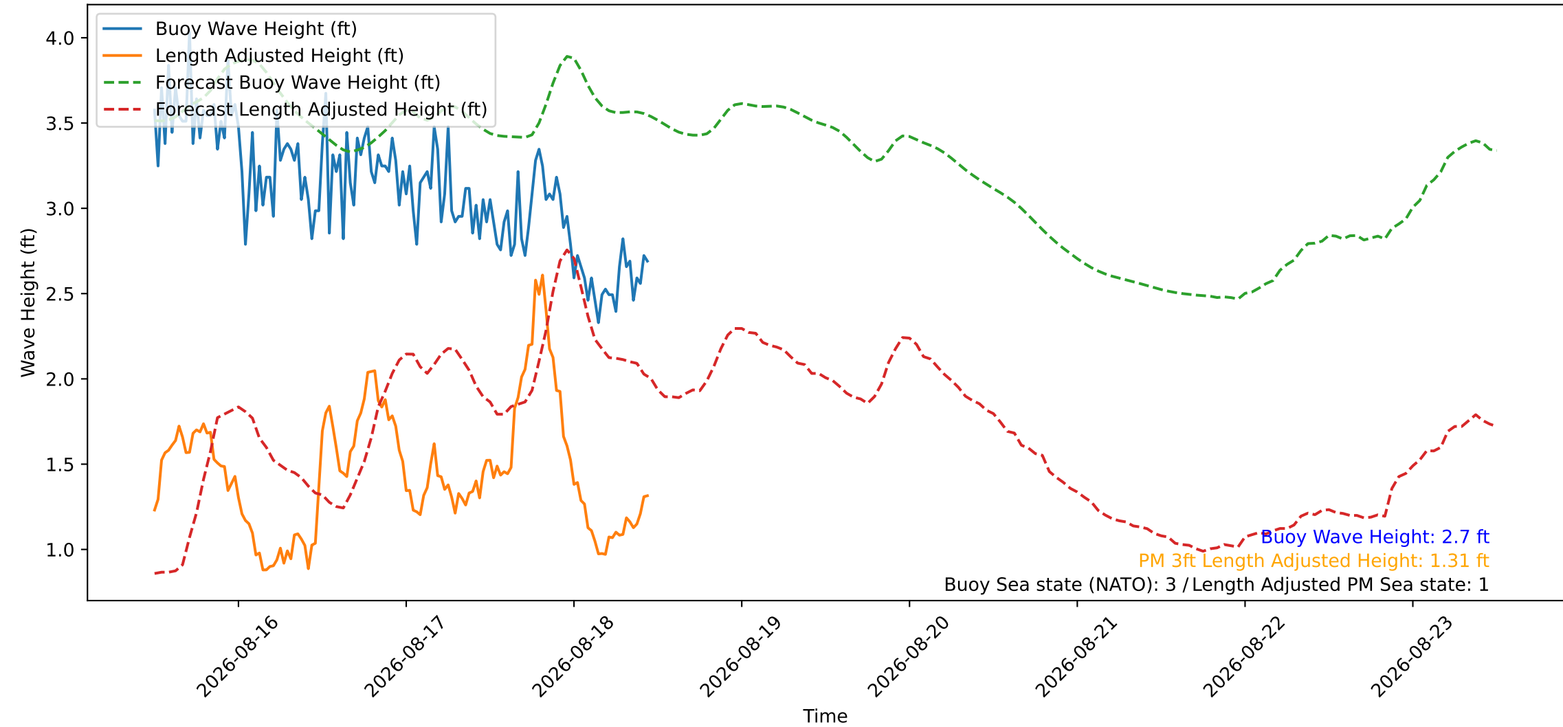
Wave Heights over Time for Red Beach at 2026-08-18 11:50:47
