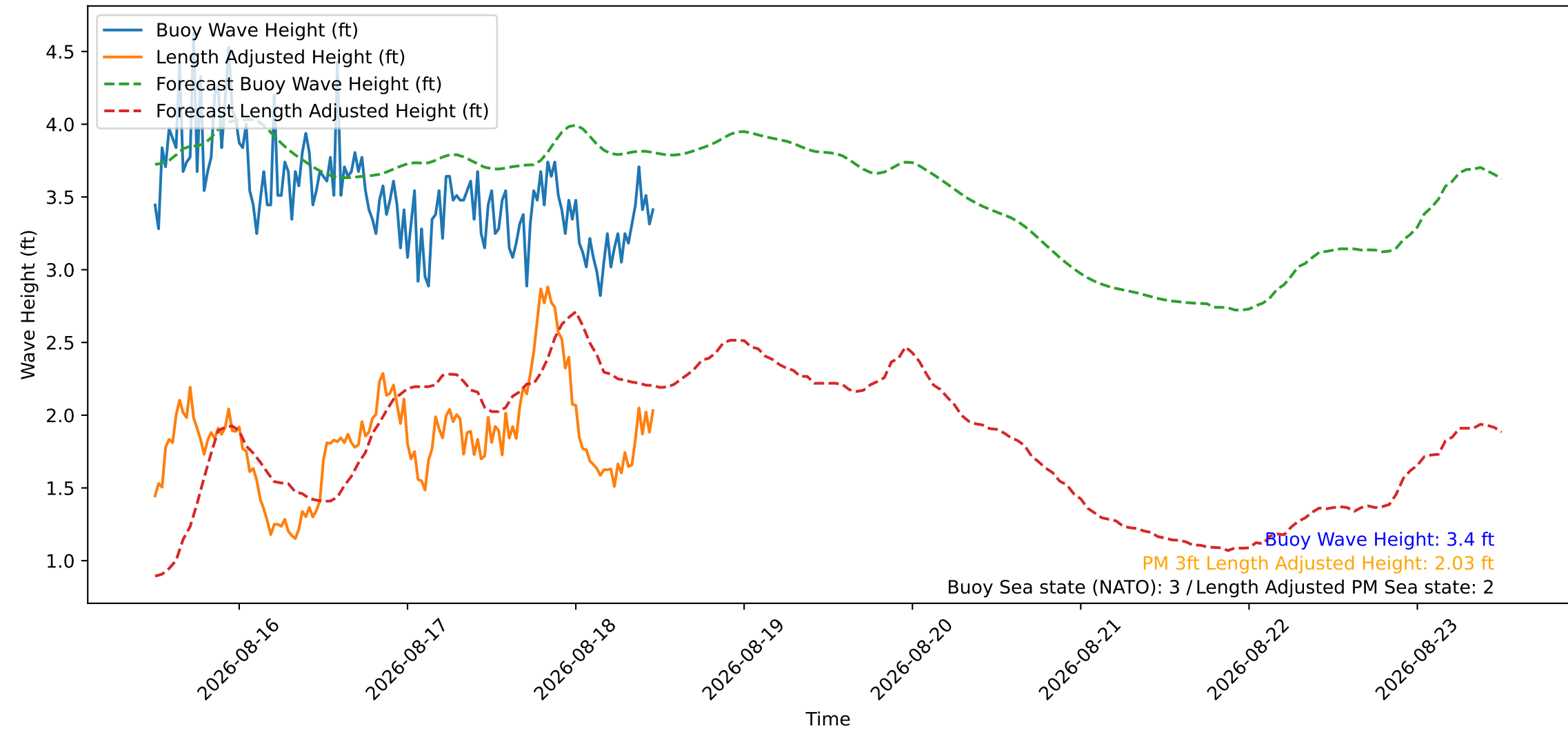
Wave Heights over Time for Oceanside Harbor at 2026-08-18 11:50:27
