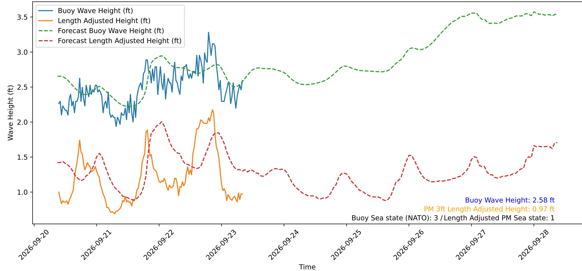
Wave Heights over Time for Red Beach at 2026-09-23 09:00:49
