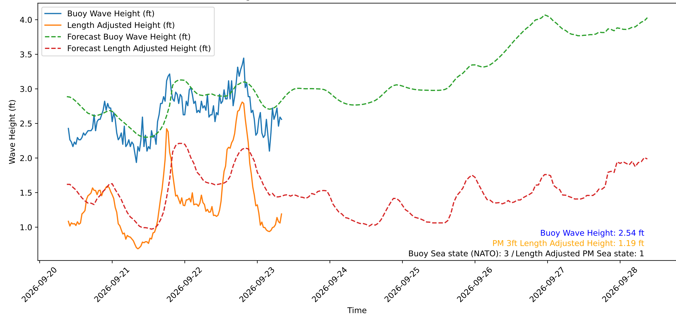
Wave Heights over Time for Green Beach at 2026-09-23 09:01:11
