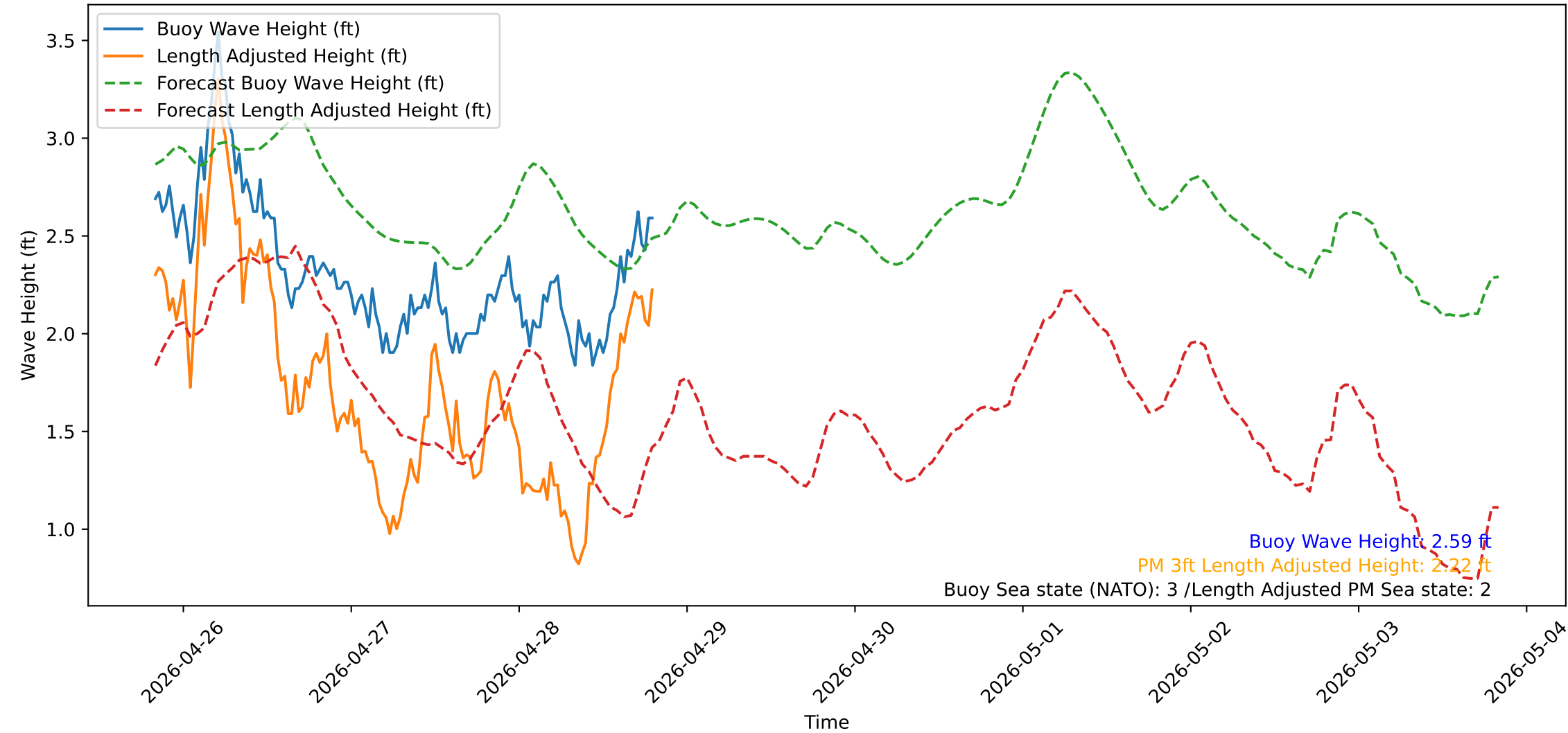
Wave Heights over Time for Red Beach at 2026-04-28 19:40:51
