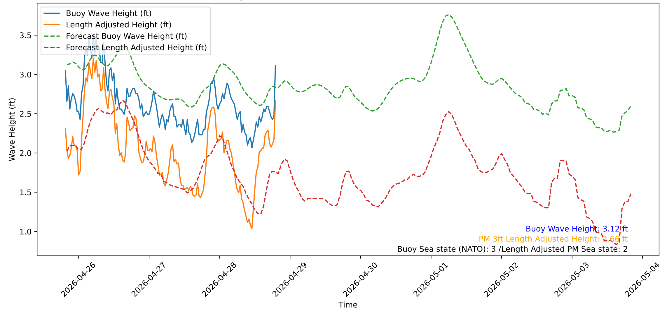
Wave Heights over Time for Green Beach at 2026-04-28 19:41:14
