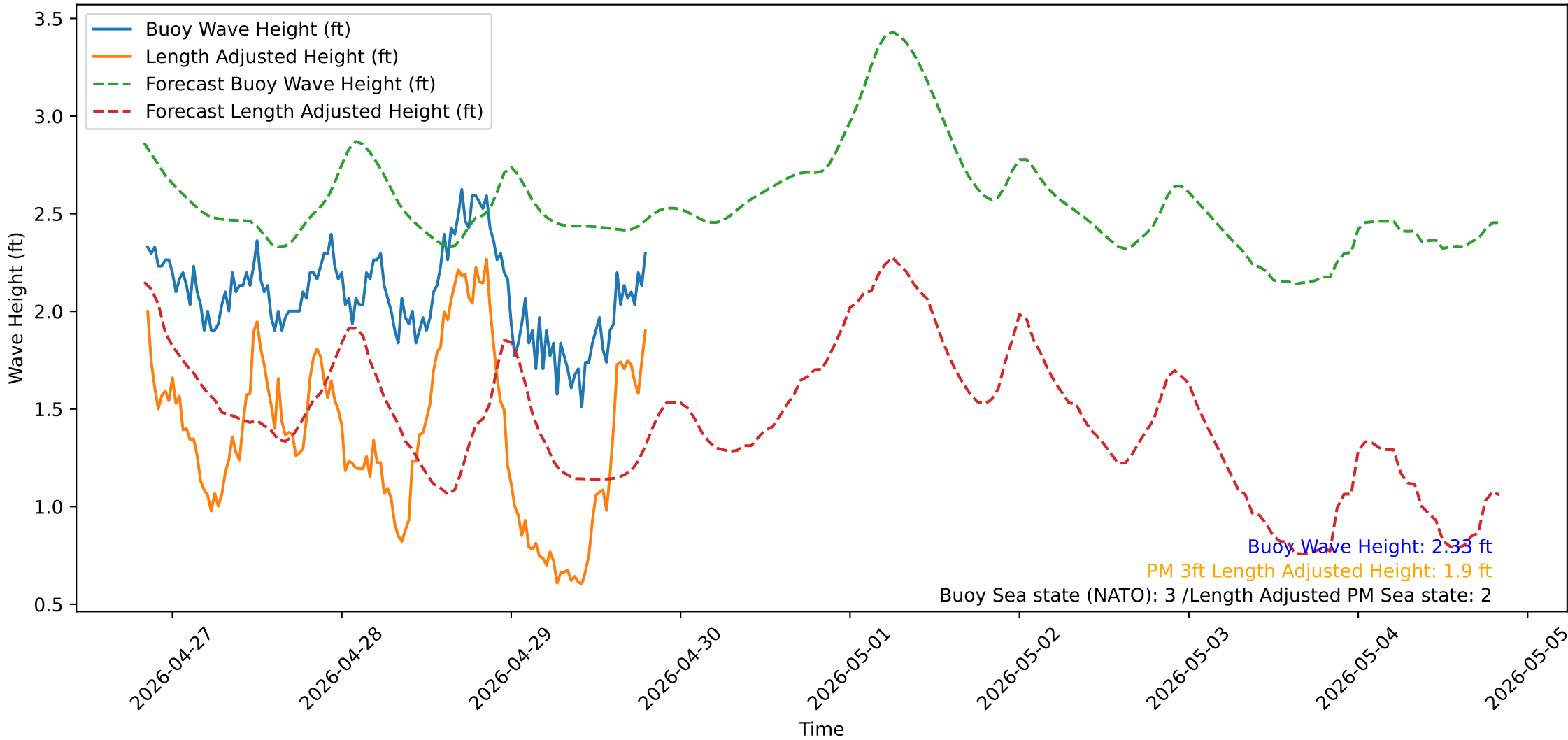
Wave Heights over Time for Red Beach at 2026-04-29 20:10:50
