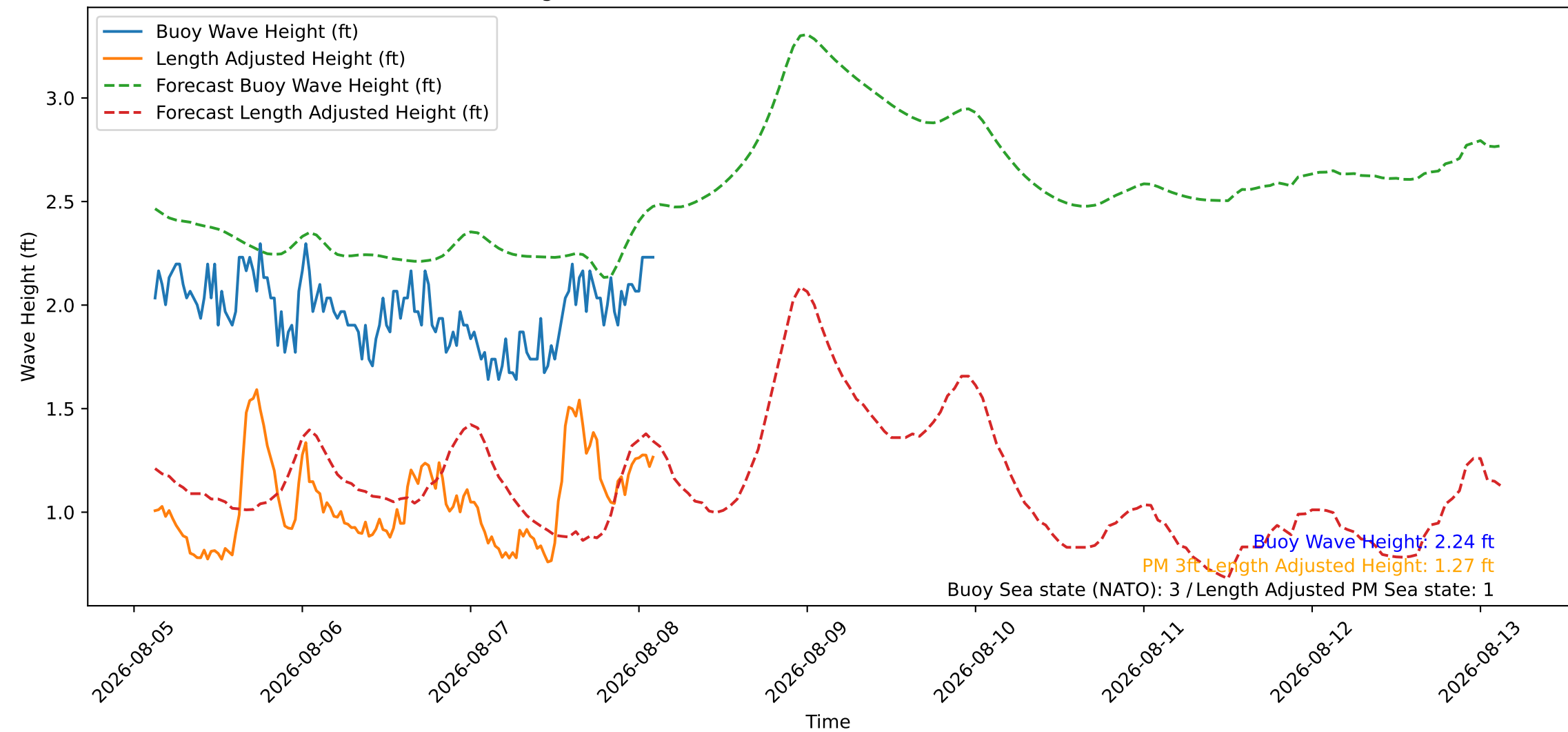
Wave Heights over Time for Oceanside Harbor at 2026-08-08 03:00:27
