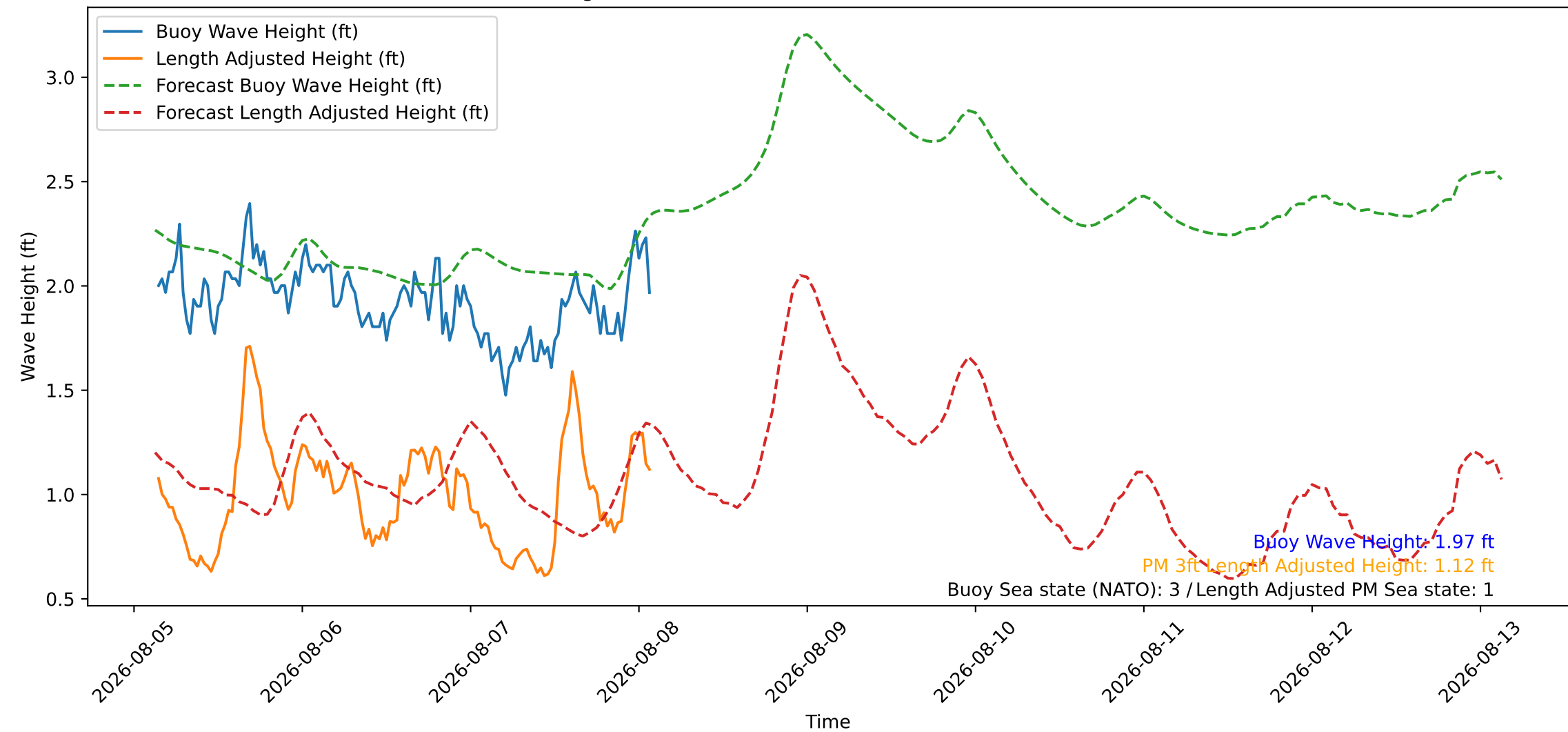
Wave Heights over Time for Red Beach at 2026-08-08 03:00:46
