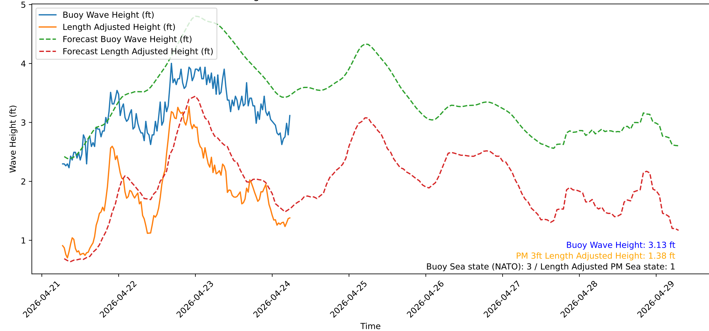
Wave Heights over Time for Green Beach at 2026-04-24 06:31:11
