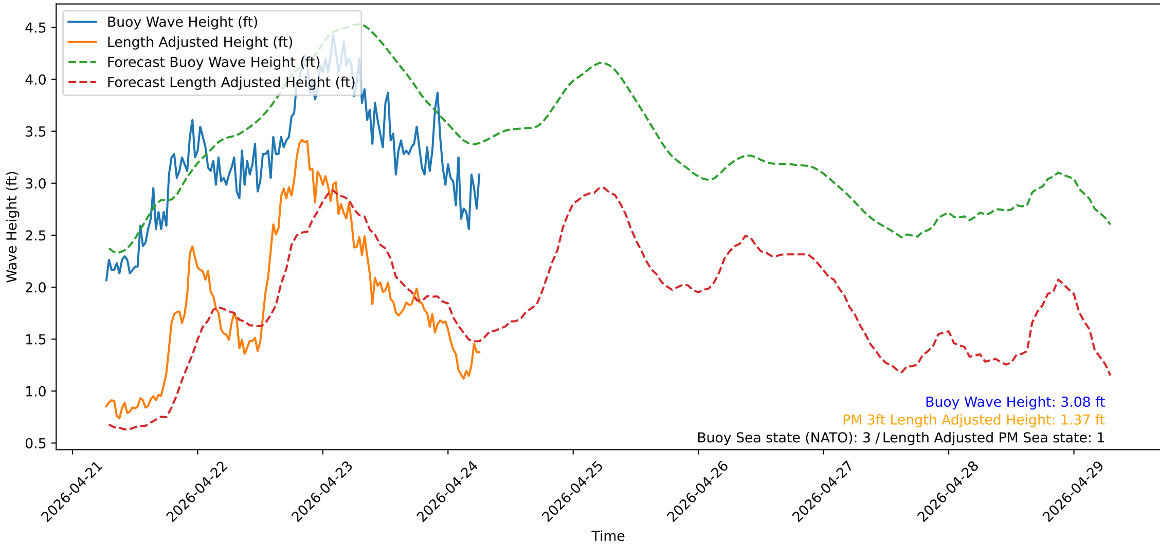
Wave Heights over Time for Oceanside Harbor at 2026-04-24 06:30:31
