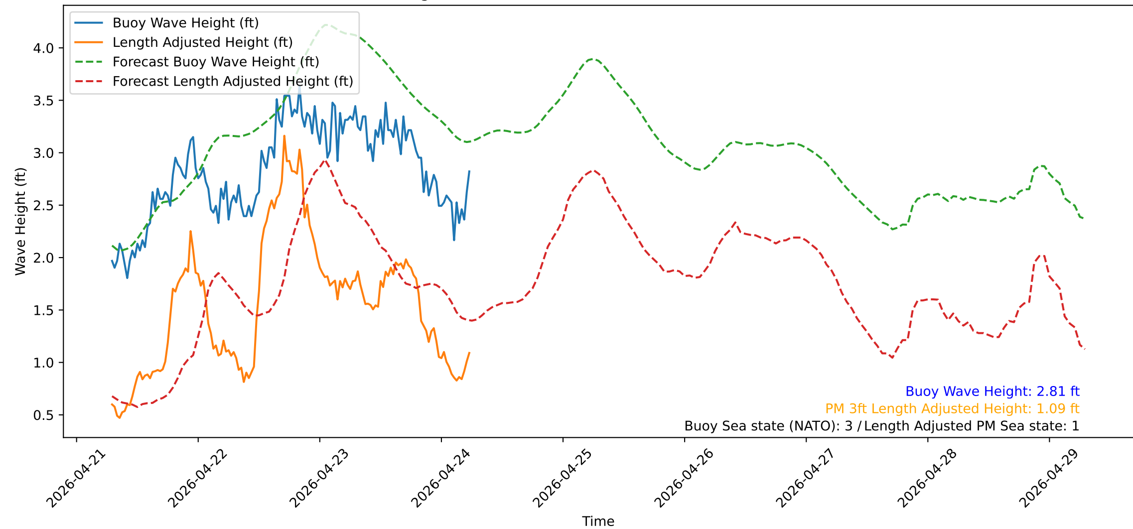
Wave Heights over Time for Red Beach at 2026-04-24 06:30:49
