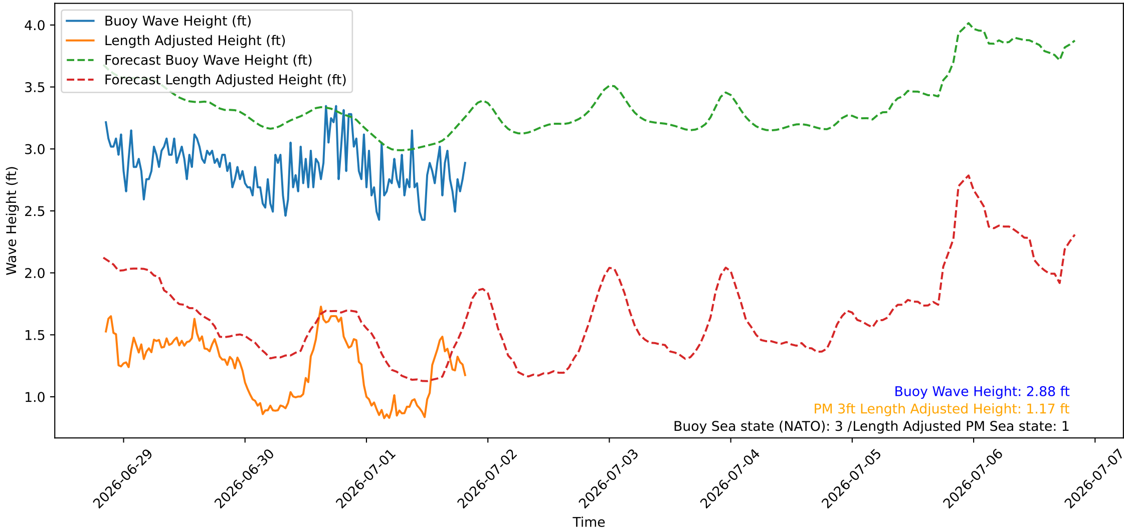
Wave Heights over Time for Red Beach at 2026-07-01 20:20:47
