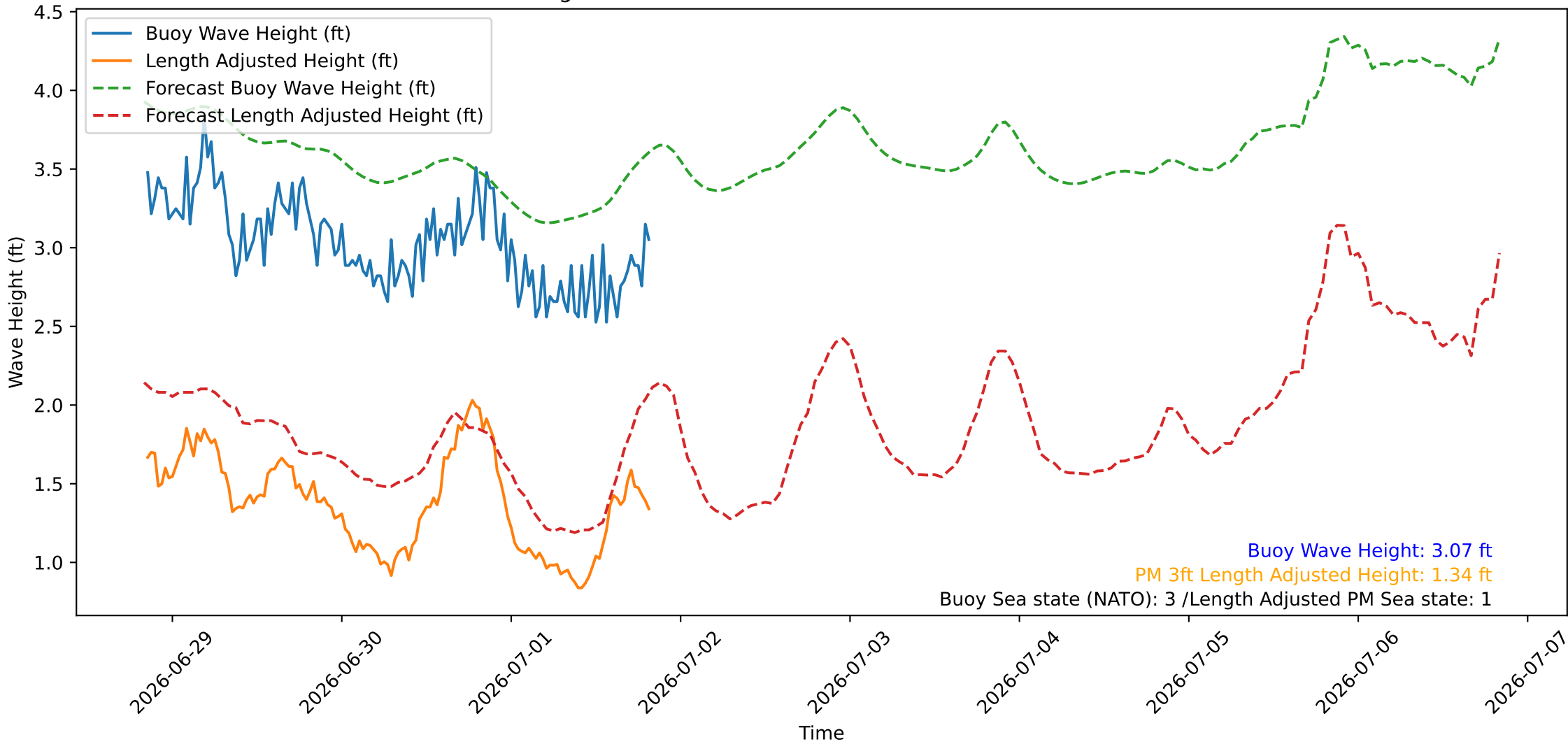
Wave Heights over Time for Green Beach at 2026-07-01 20:21:09
