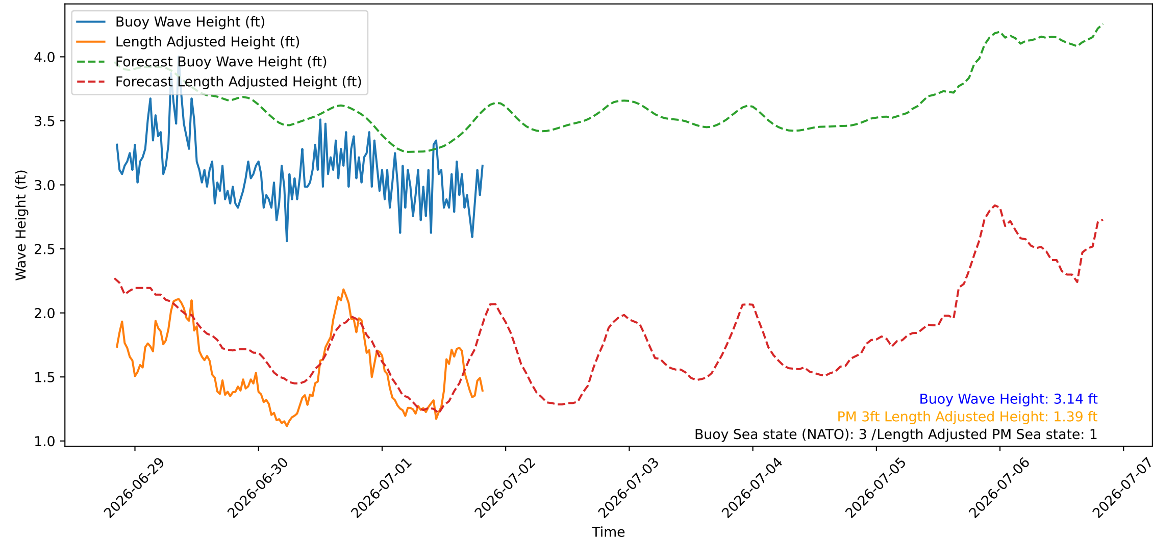
Wave Heights over Time for Oceanside Harbor at 2026-07-01 20:20:26
