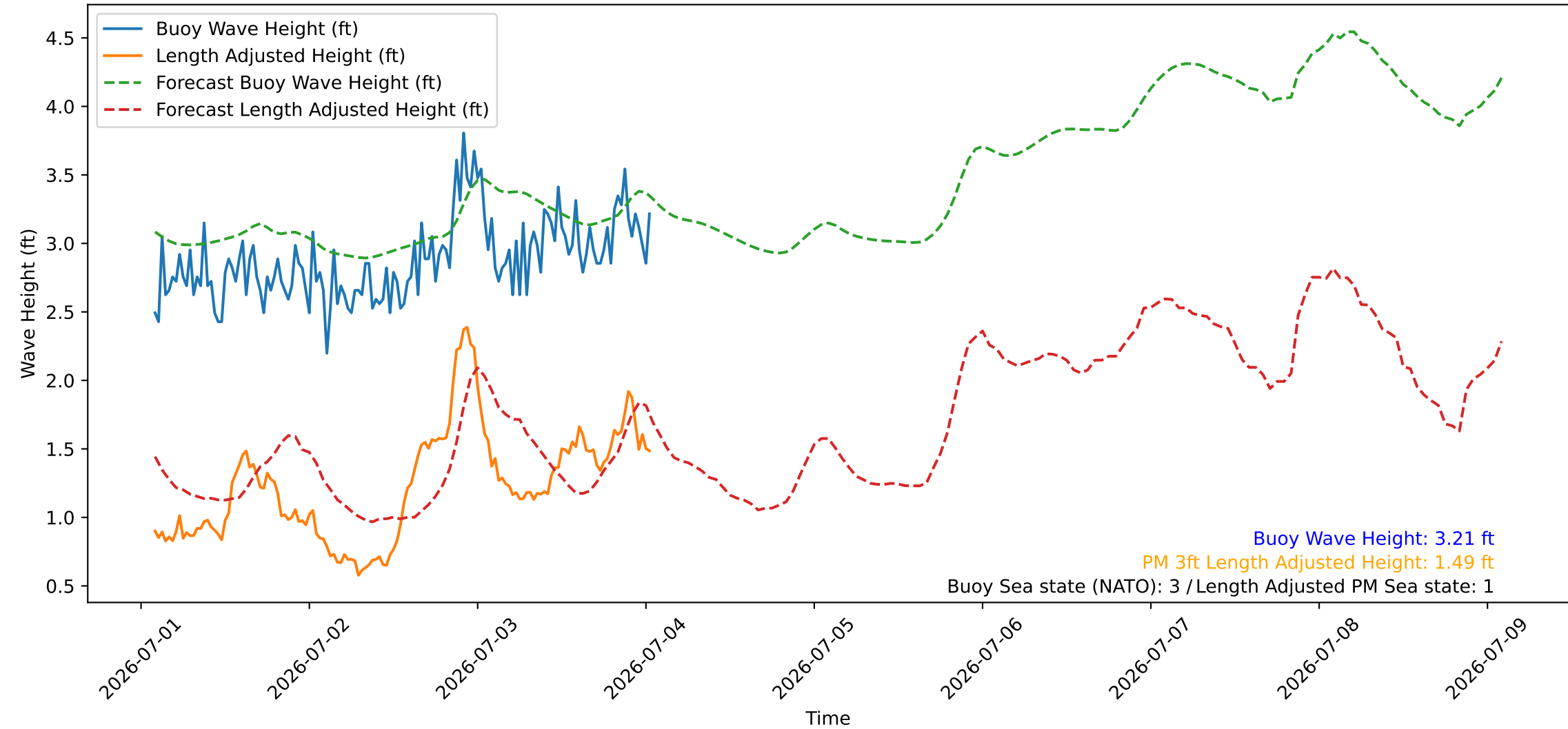
Wave Heights over Time for Red Beach at 2026-07-04 01:40:46
