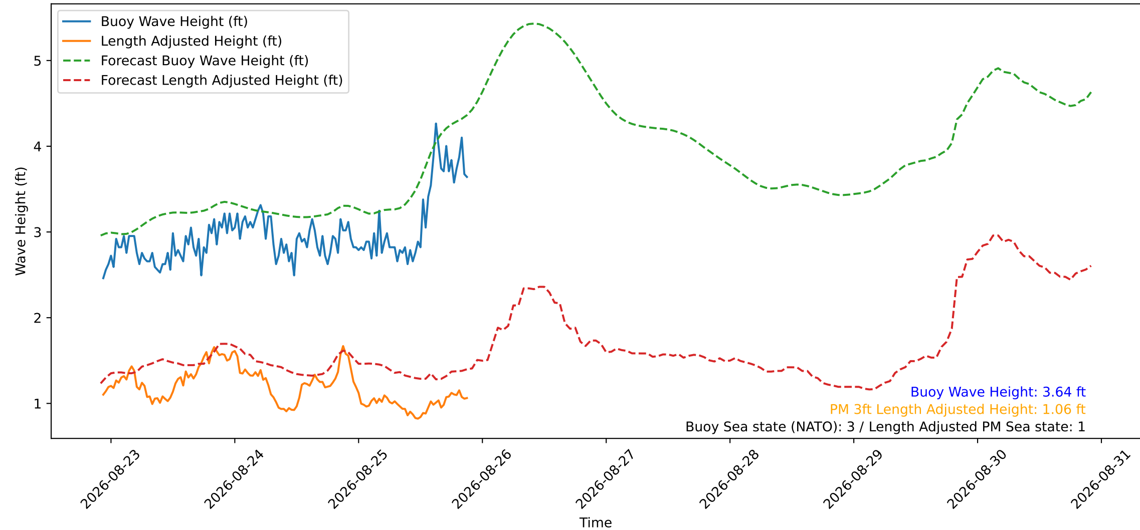
Wave Heights over Time for Green Beach at 2026-08-25 22:01:12
