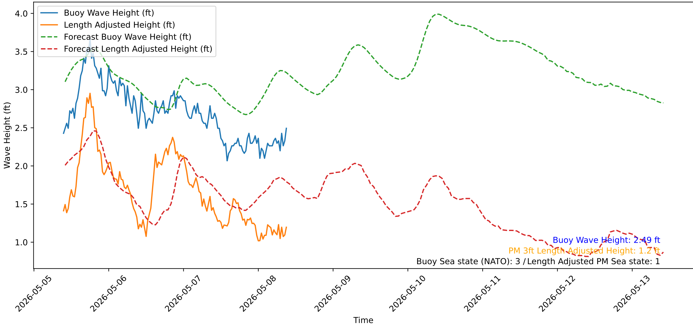
Wave Heights over Time for Green Beach at 2026-05-08 09:41:13
