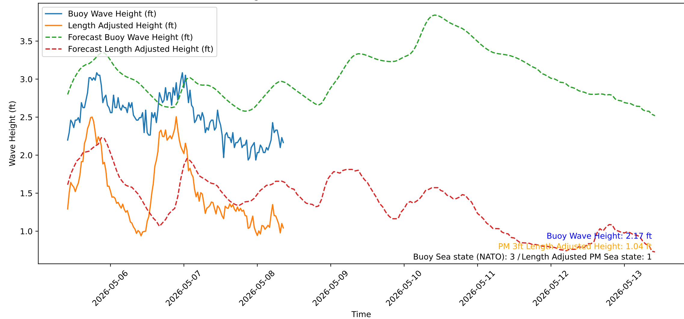
Wave Heights over Time for Red Beach at 2026-05-08 09:40:50
