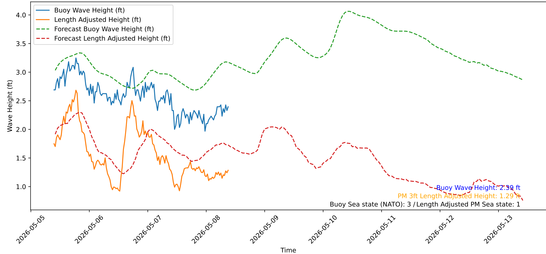
Wave Heights over Time for Oceanside Harbor at 2026-05-08 09:40:31
