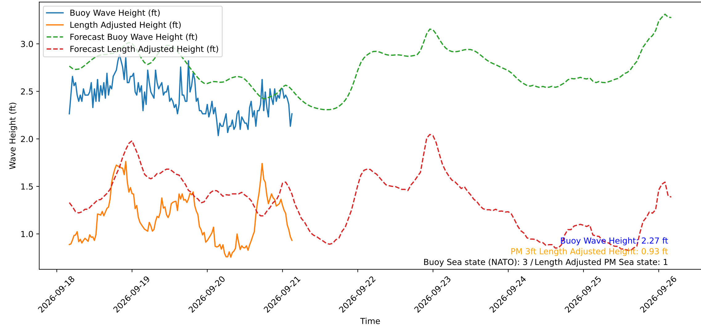
Wave Heights over Time for Red Beach at 2026-09-21 03:50:51
