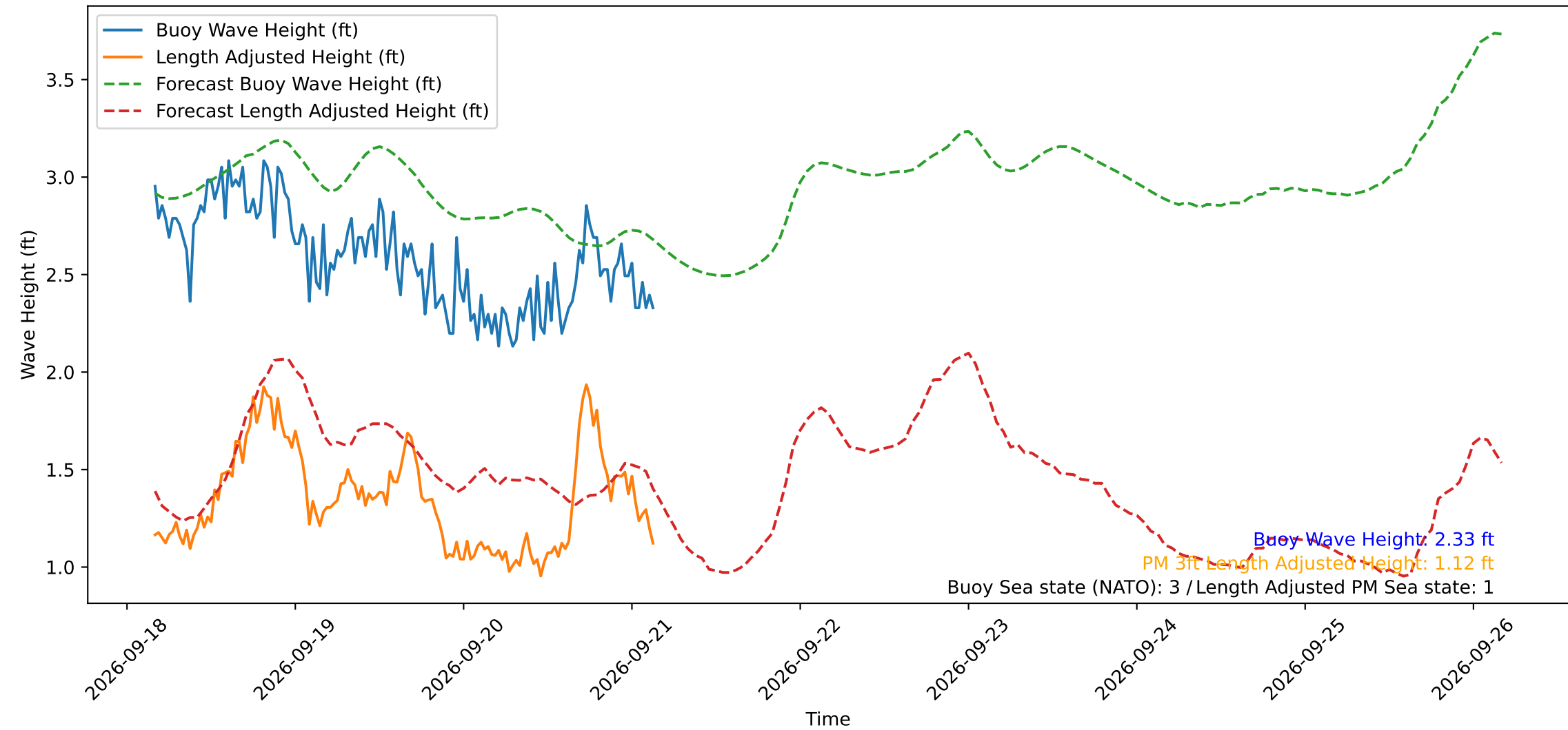
Wave Heights over Time for Oceanside Harbor at 2026-09-21 03:50:30
