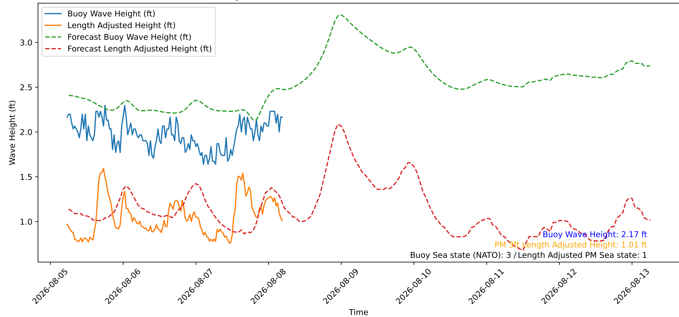
Wave Heights over Time for Oceanside Harbor at 2026-08-08 05:30:26
