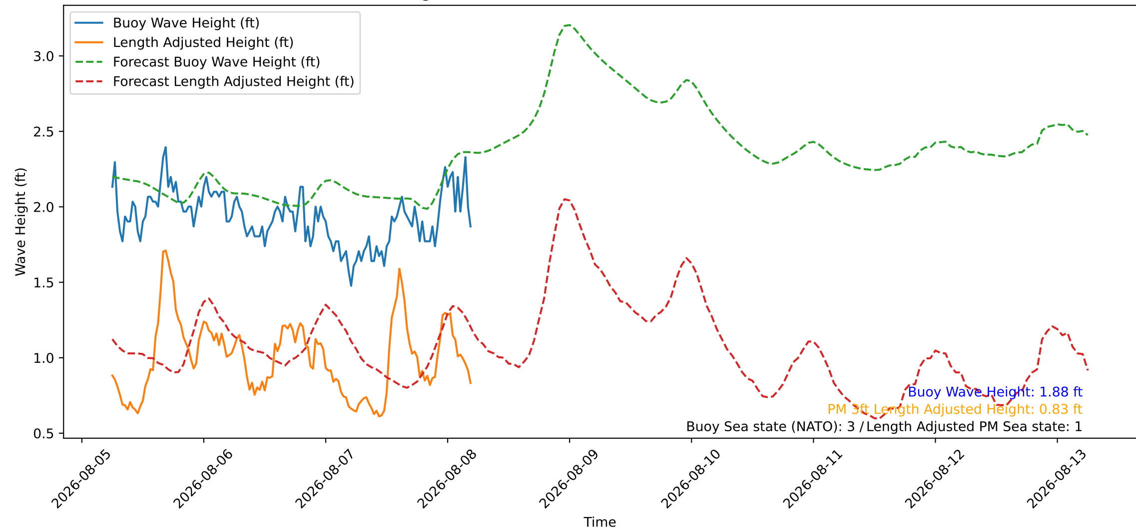
Wave Heights over Time for Red Beach at 2026-08-08 05:30:46
