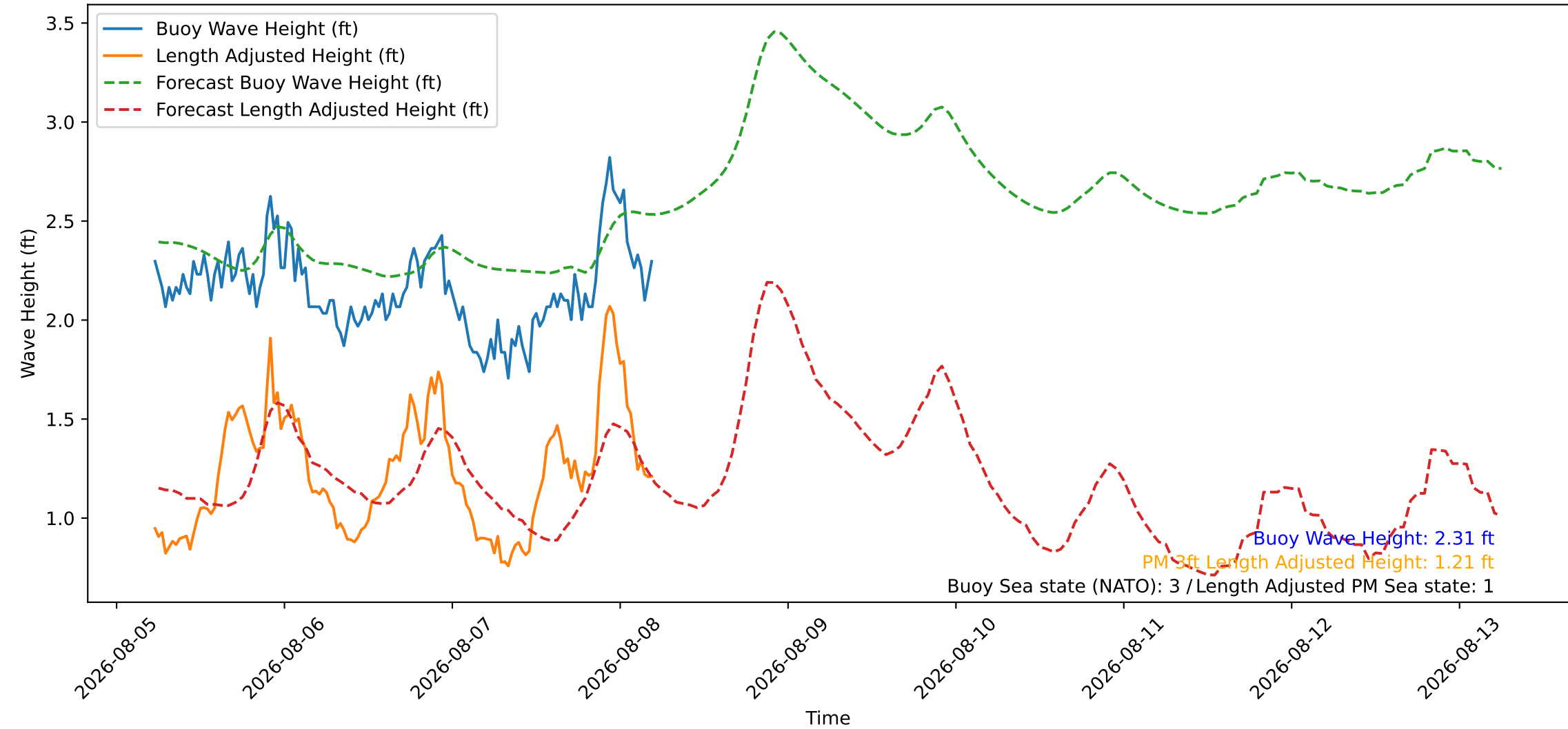
Wave Heights over Time for Green Beach at 2026-08-08 05:31:08
