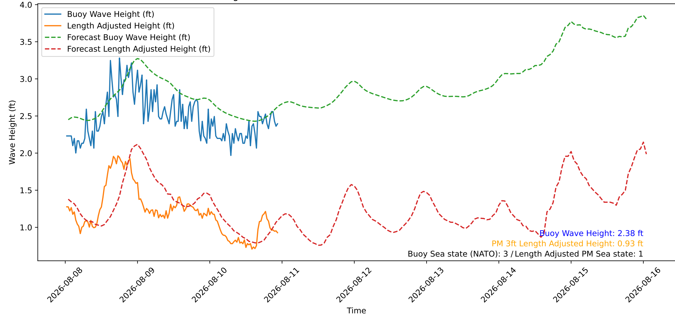
Wave Heights over Time for Oceanside Harbor at 2026-08-11 00:30:26
