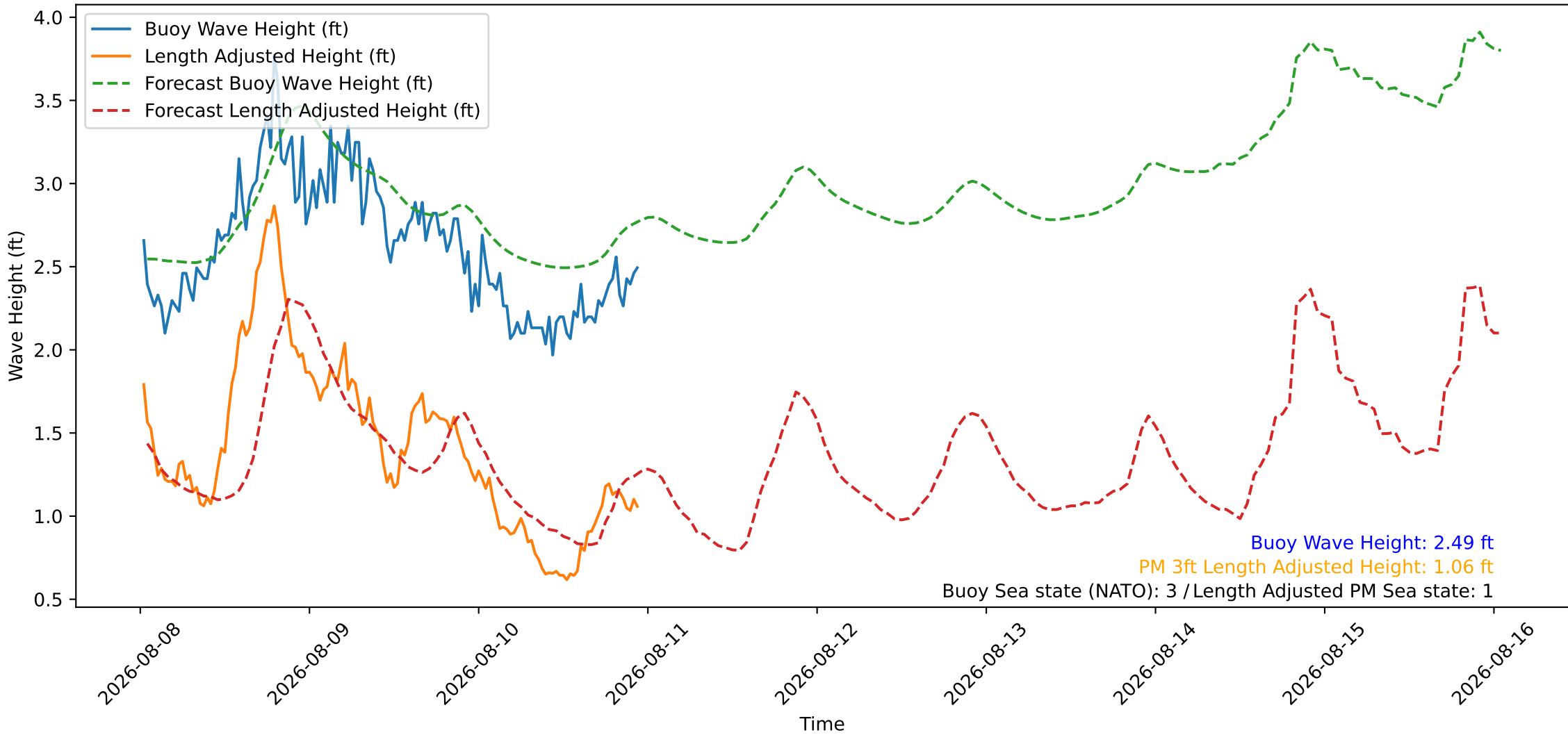
Wave Heights over Time for Green Beach at 2026-08-11 00:31:09
