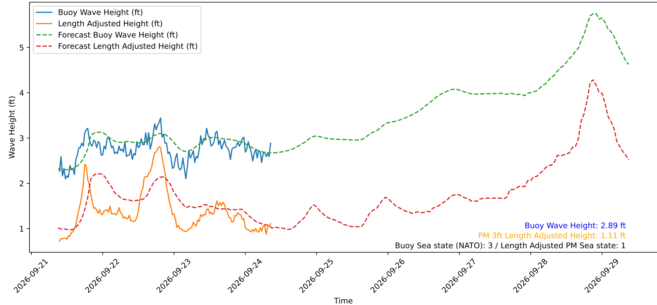
Wave Heights over Time for Green Beach at 2026-09-24 09:11:12
