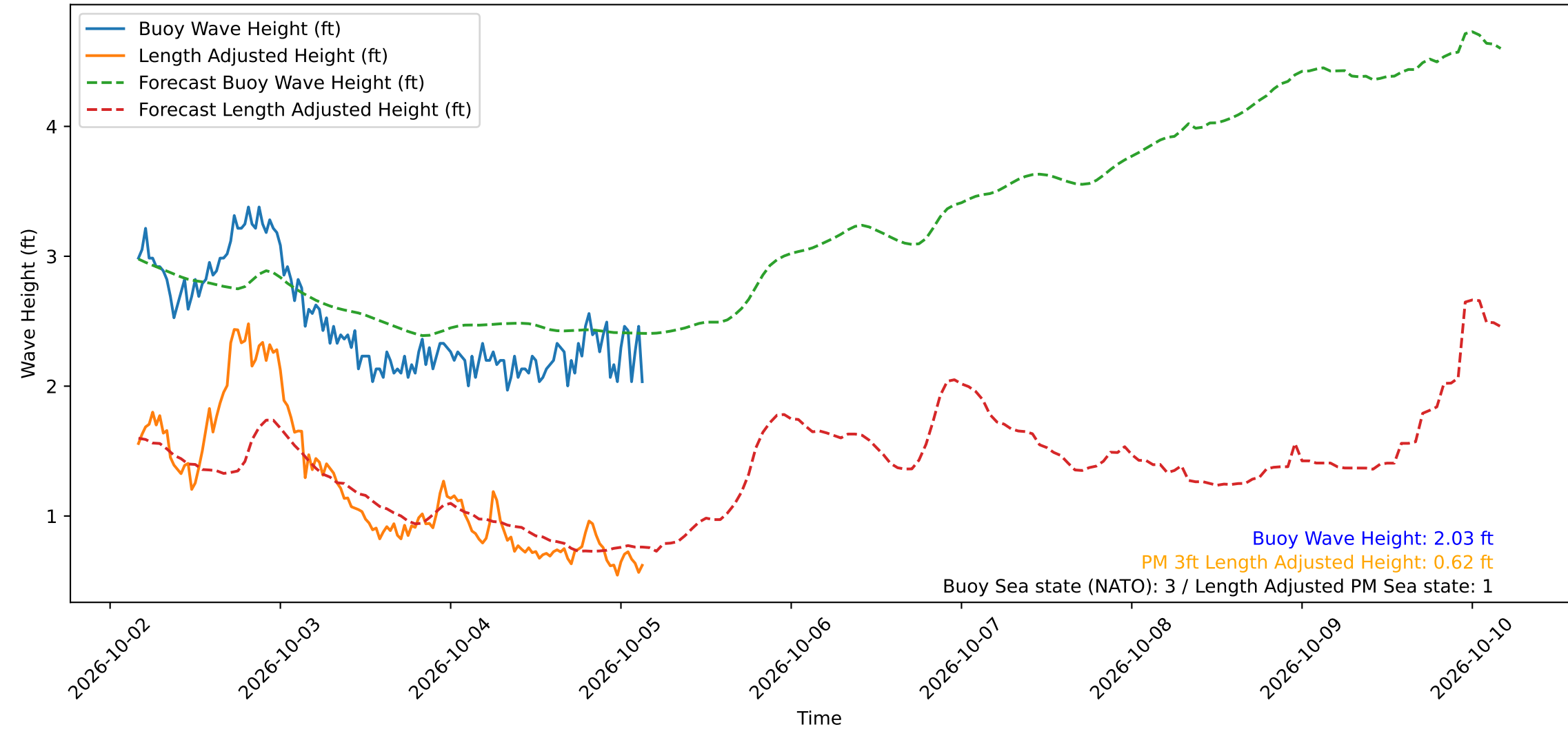
Wave Heights over Time for Green Beach at 2026-10-05 03:51:14
