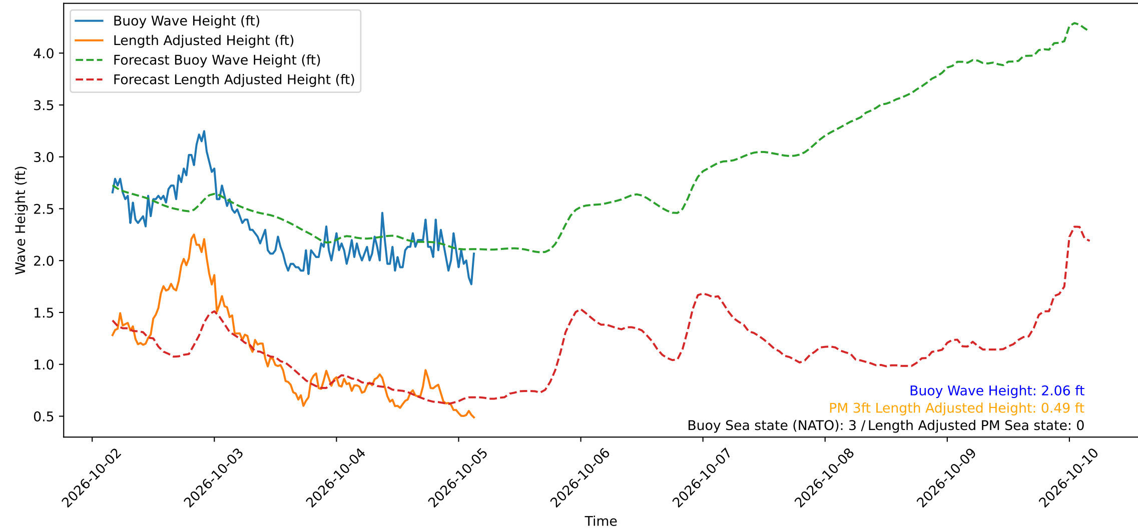
Wave Heights over Time for Red Beach at 2026-10-05 03:50:50
