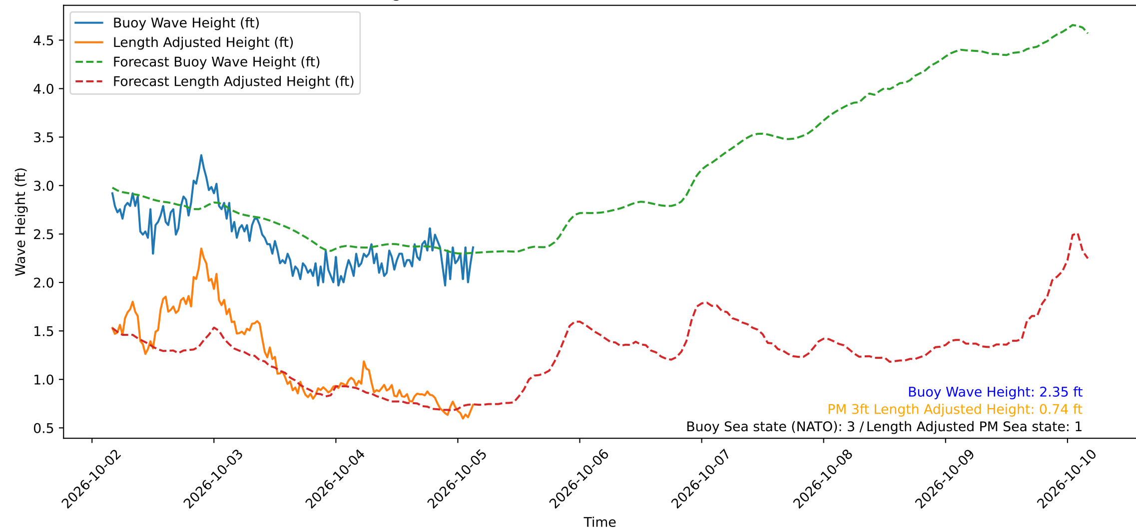
Wave Heights over Time for Oceanside Harbor at 2026-10-05 03:50:29
