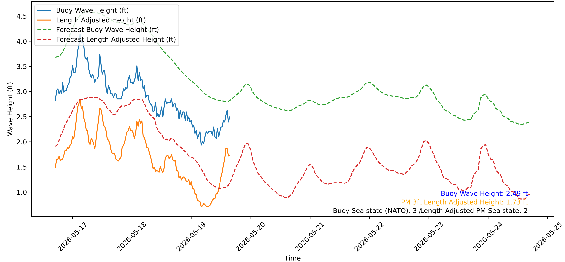
Wave Heights over Time for Red Beach at 2026-05-19 16:50:52
