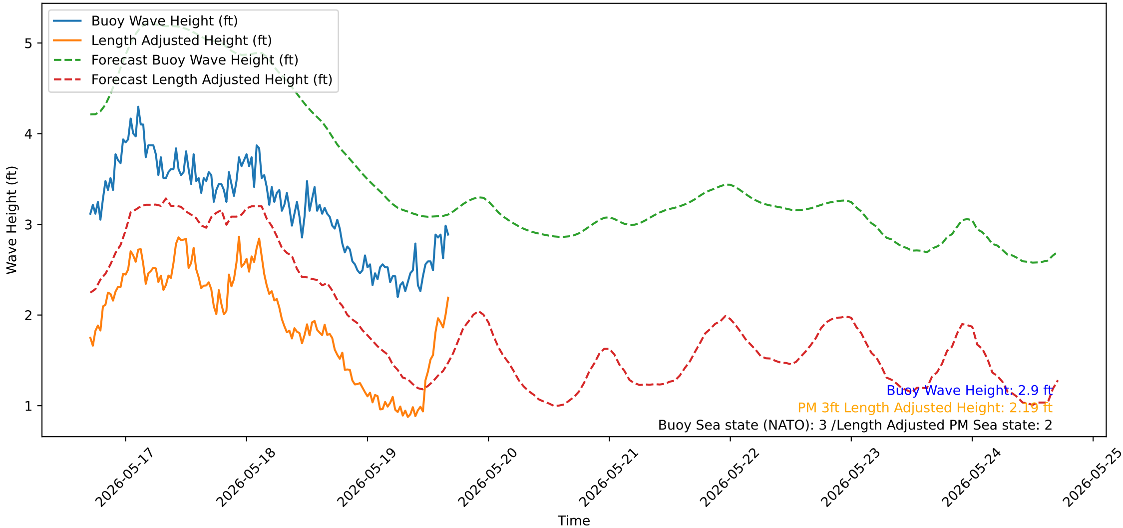
Wave Heights over Time for Oceanside Harbor at 2026-05-19 16:50:31
