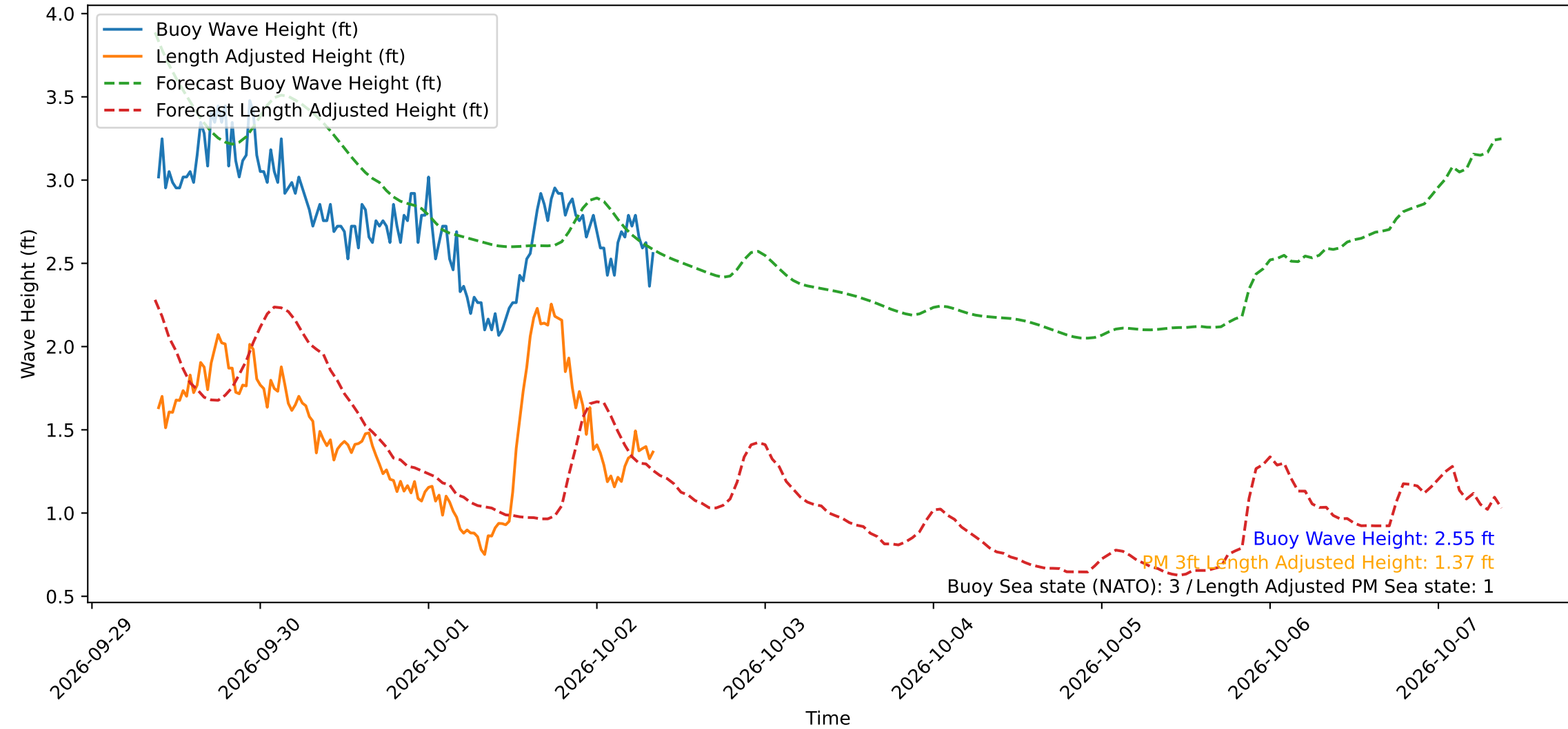
Wave Heights over Time for Red Beach at 2026-10-02 09:00:49
