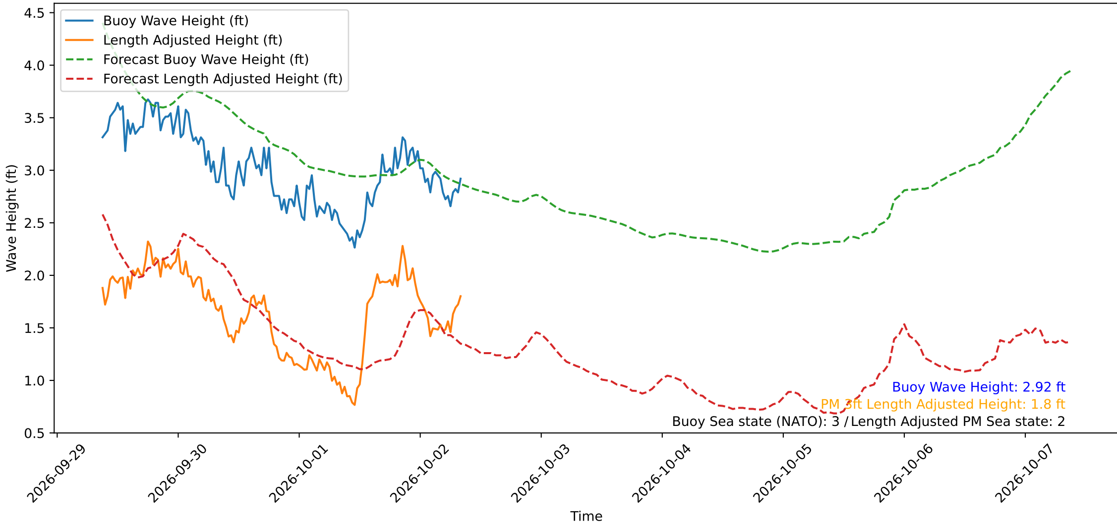
Wave Heights over Time for Oceanside Harbor at 2026-10-02 09:00:29
