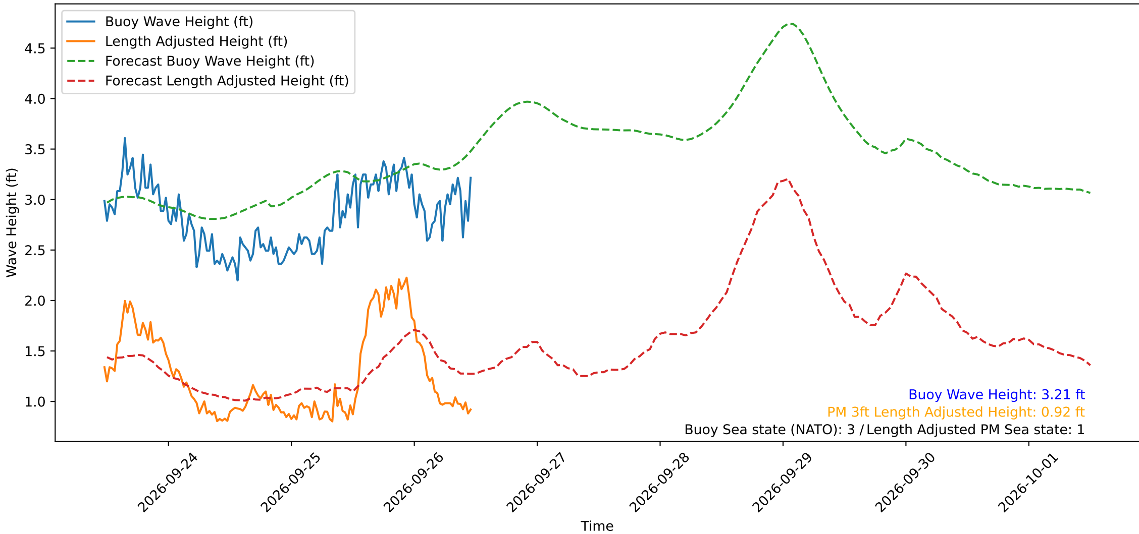
Wave Heights over Time for Oceanside Harbor at 2026-09-26 11:40:30
