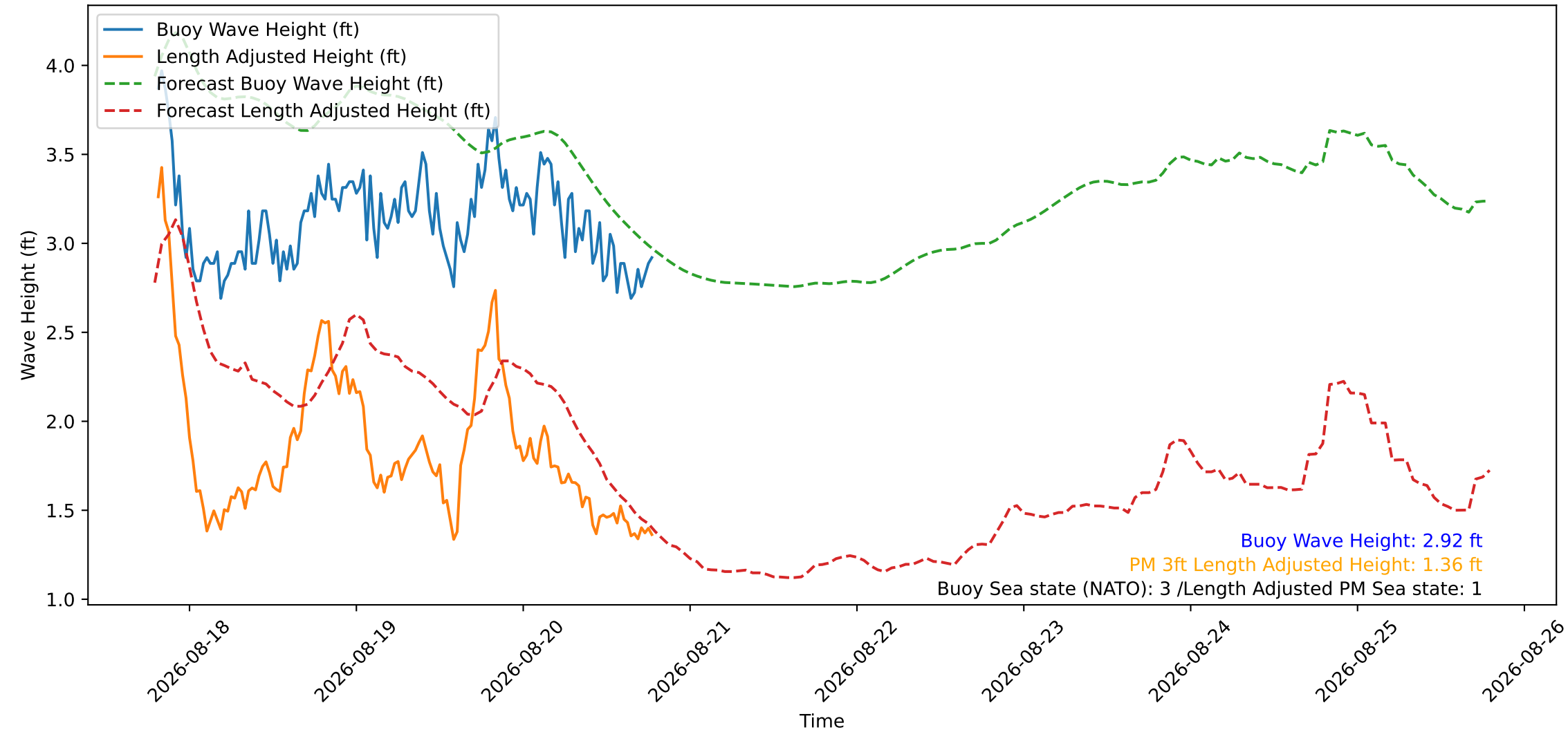
Wave Heights over Time for Green Beach at 2026-08-20 19:11:08
