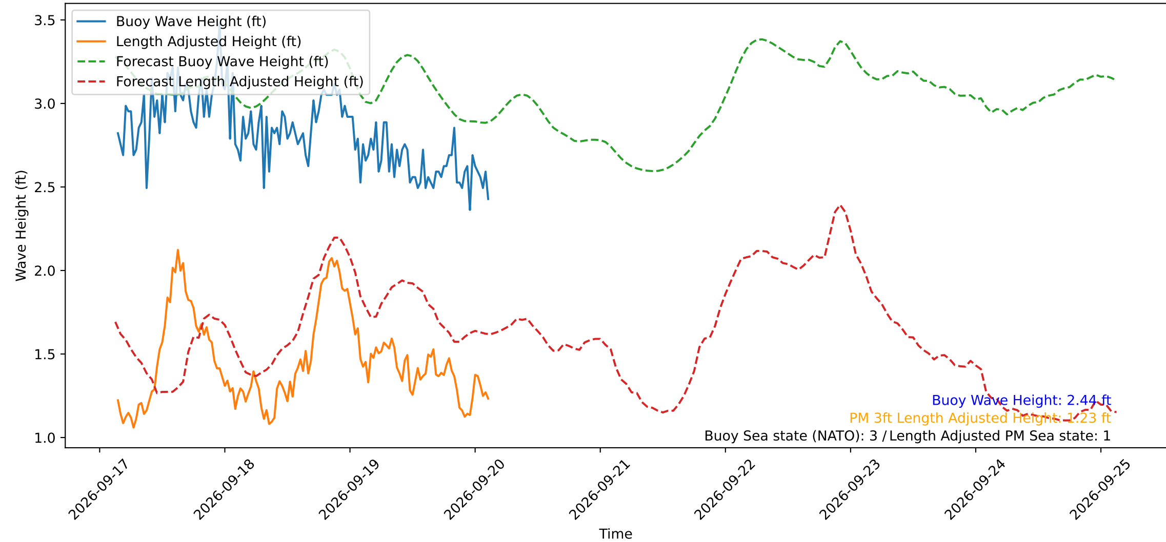
Wave Heights over Time for Green Beach at 2026-09-20 03:21:13
