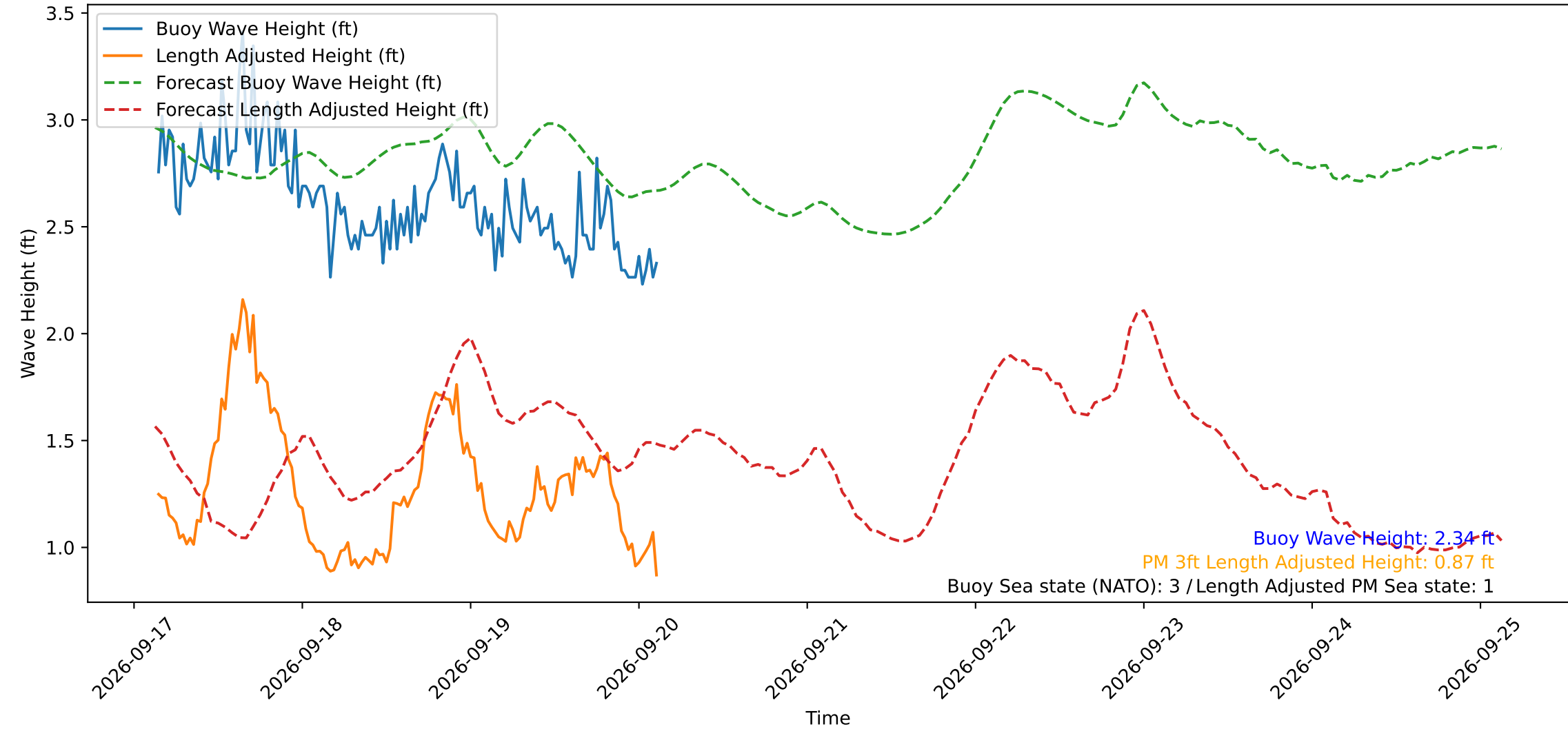
Wave Heights over Time for Red Beach at 2026-09-20 03:20:50
