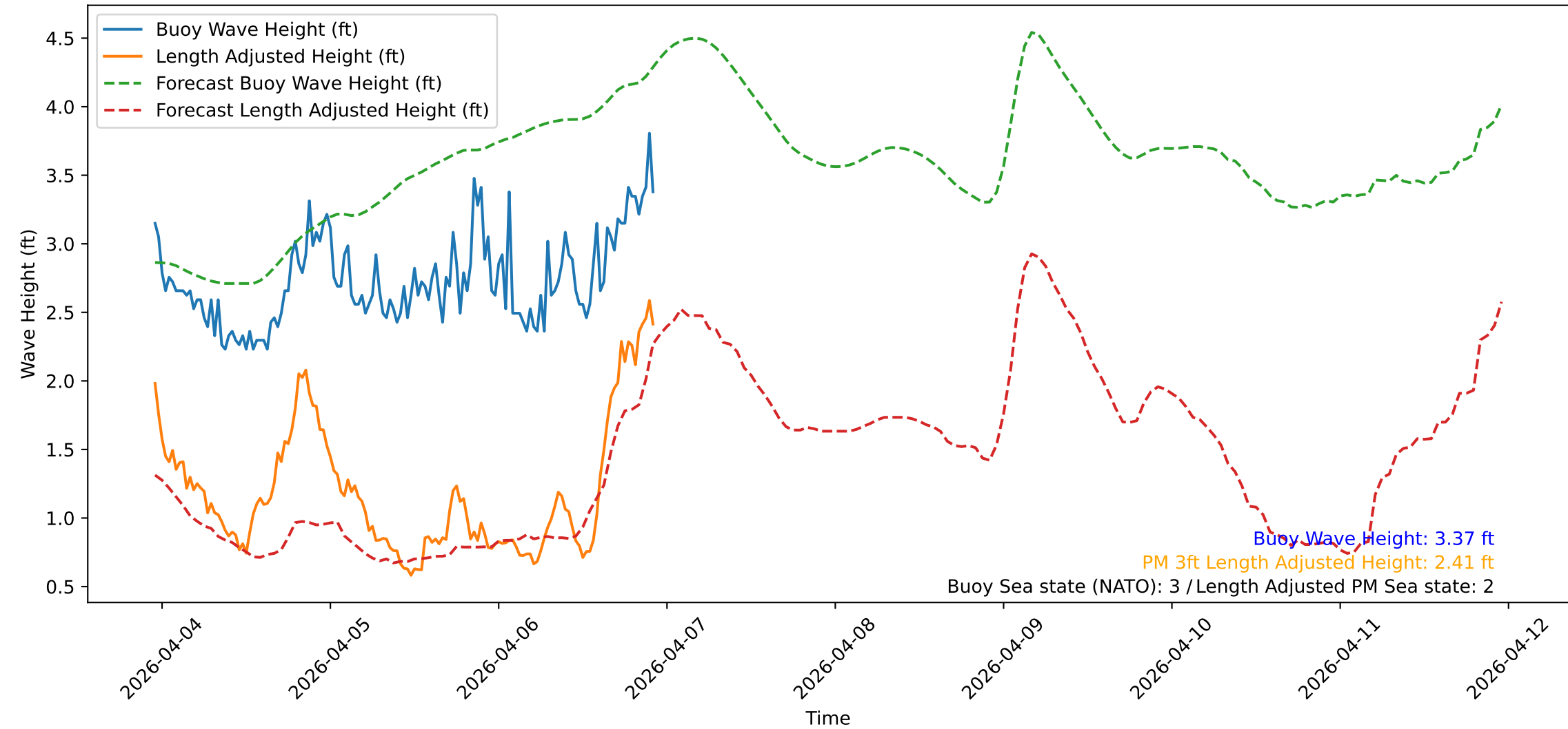
Wave Heights over Time for Green Beach at 2026-04-06 23:01:10
