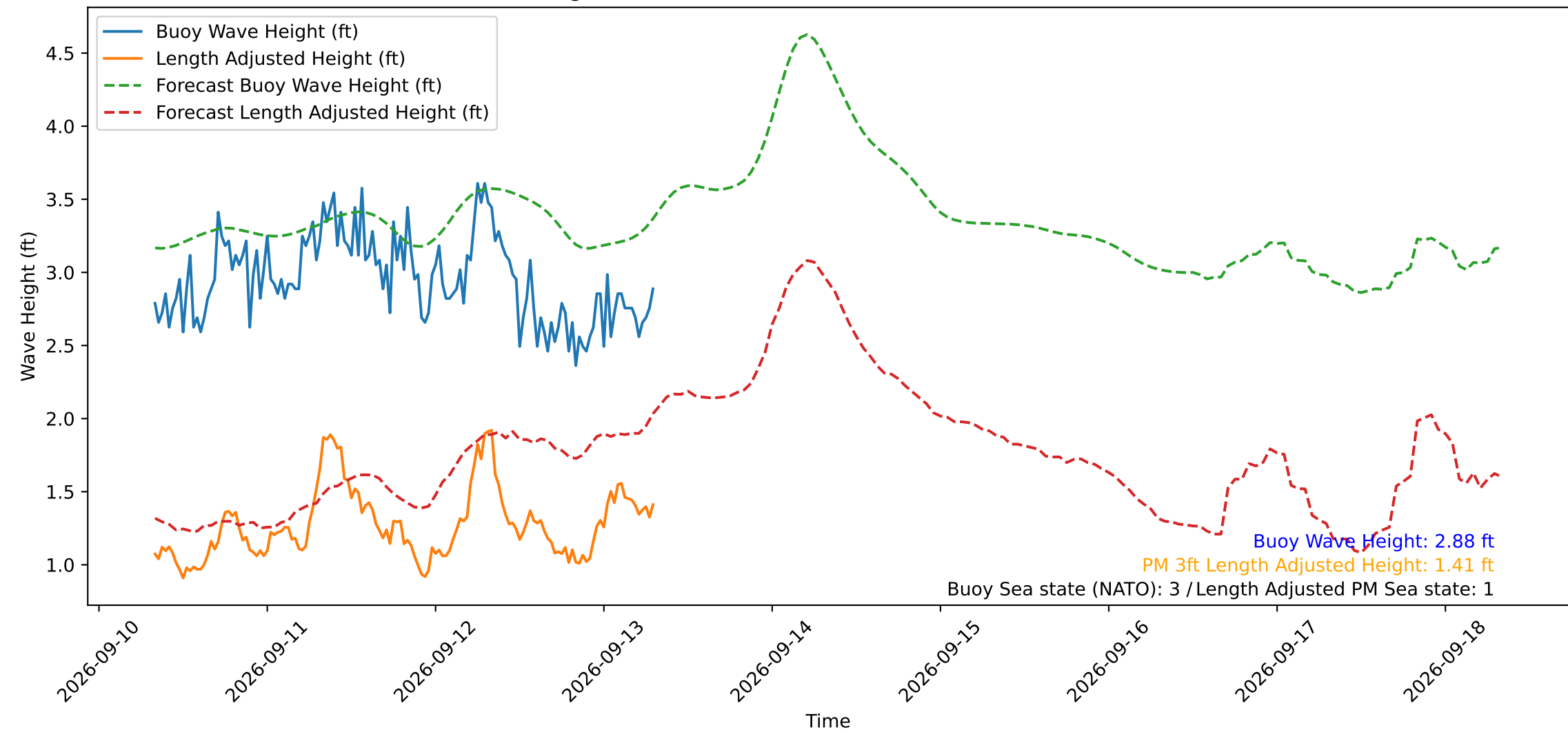
Wave Heights over Time for Green Beach at 2026-09-13 07:51:14
