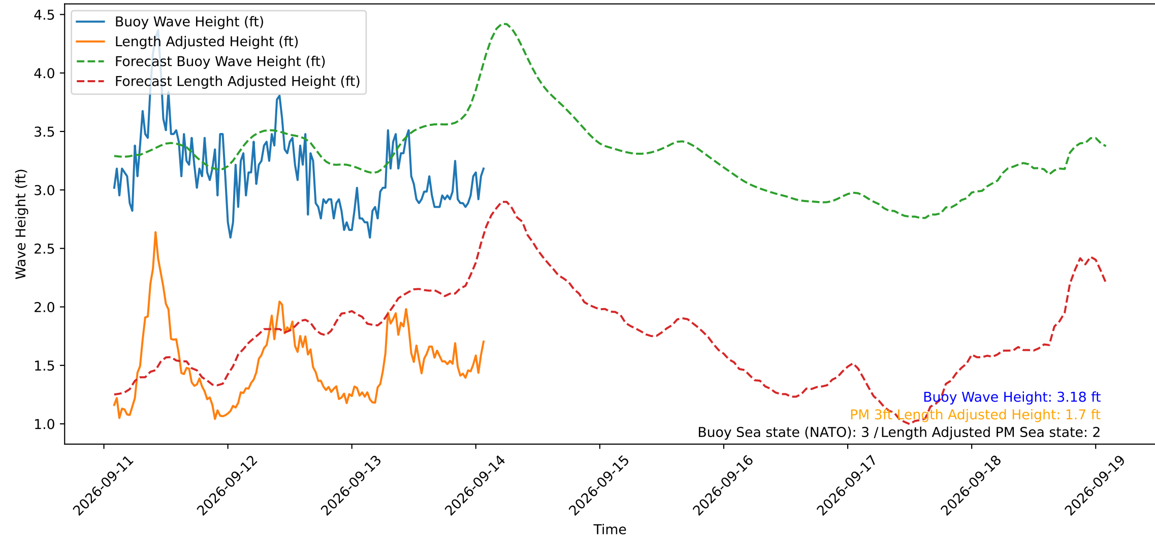
Wave Heights over Time for Oceanside Harbor at 2026-09-14 02:10:29
