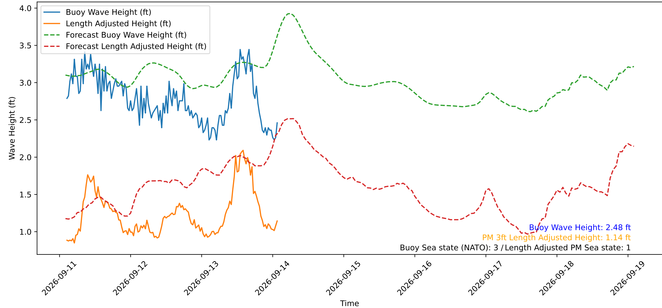
Wave Heights over Time for Red Beach at 2026-09-14 02:10:48
