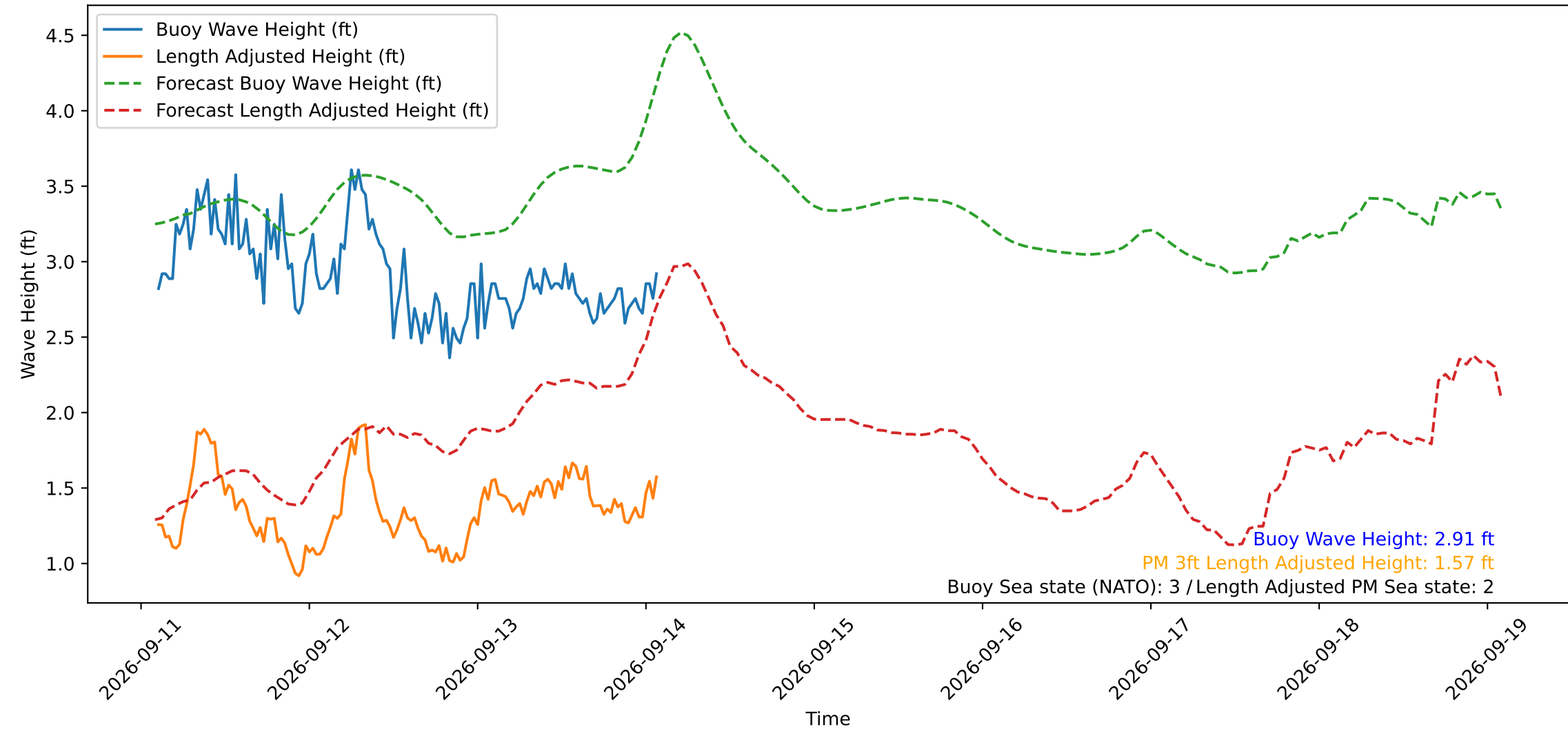
Wave Heights over Time for Green Beach at 2026-09-14 02:11:10
