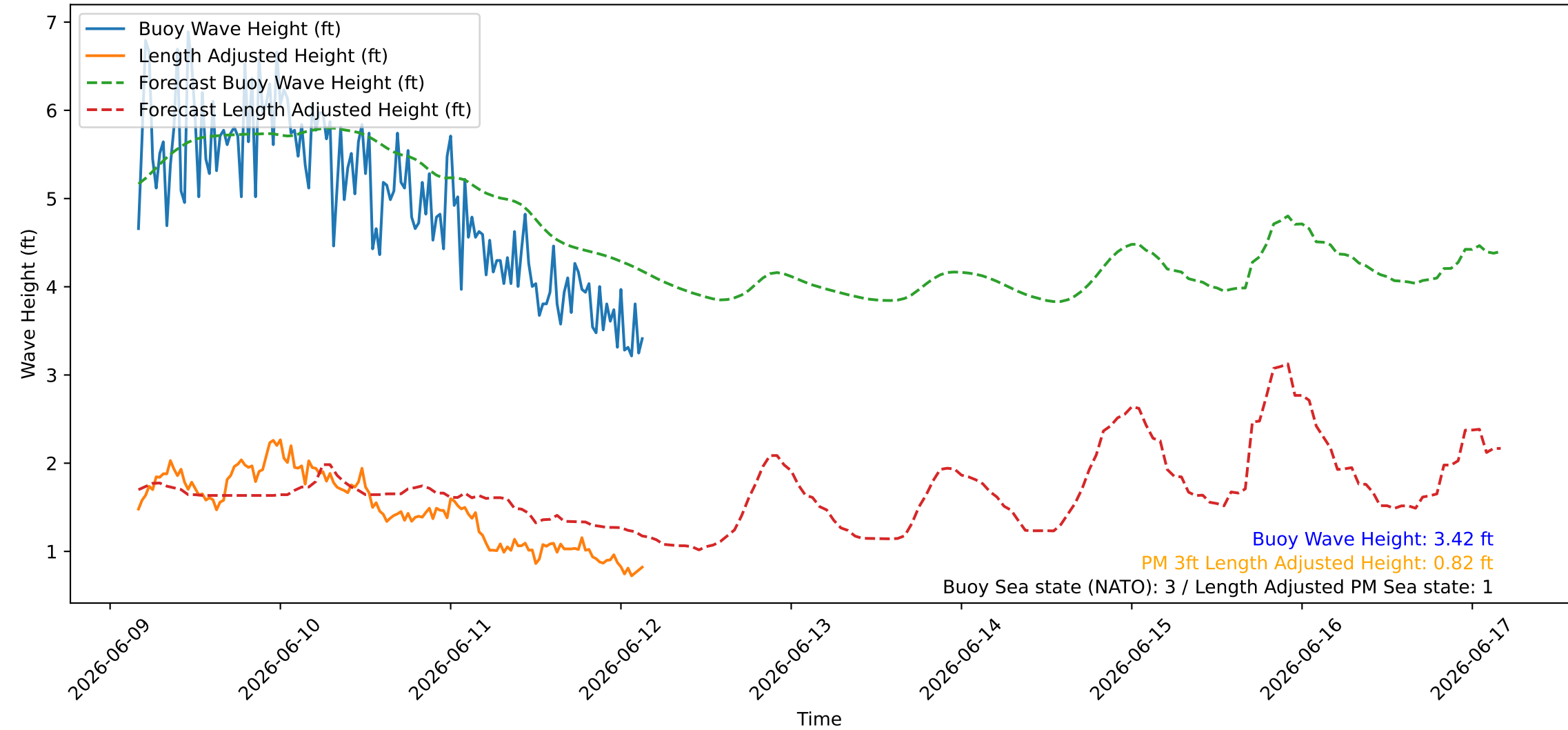
Wave Heights over Time for Green Beach at 2026-06-12 04:01:08
