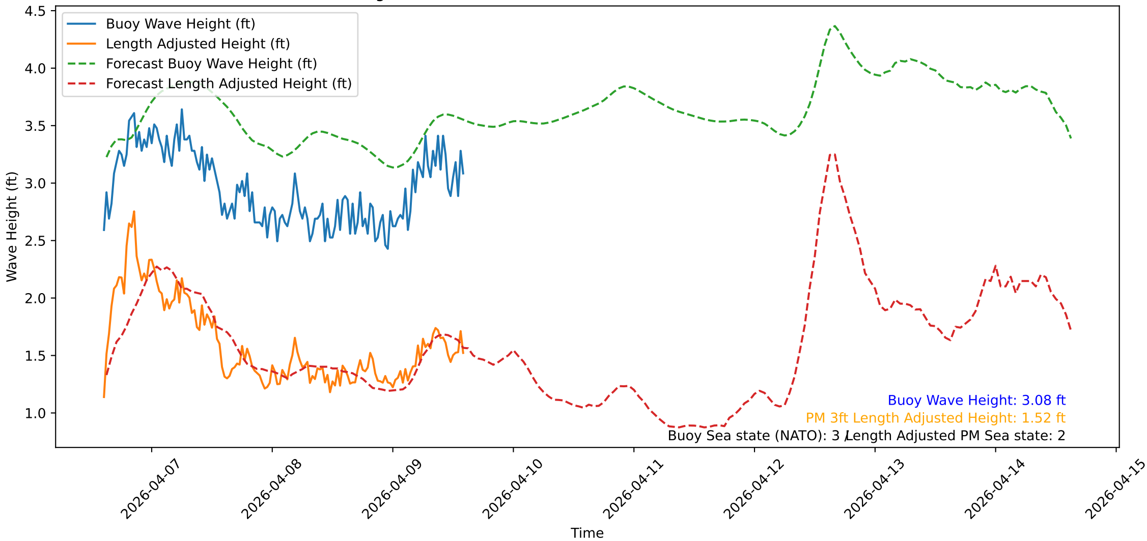
Wave Heights over Time for Oceanside Harbor at 2026-04-09 14:30:32
