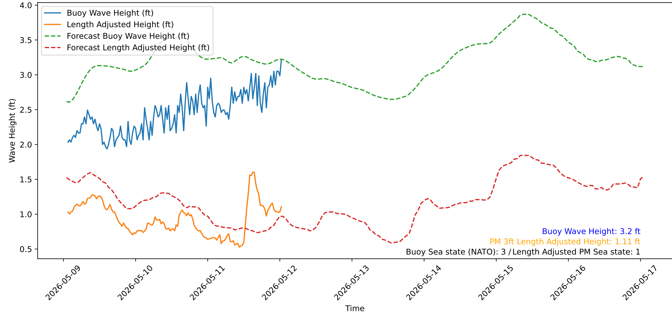
Wave Heights over Time for Red Beach at 2026-05-12 01:10:50
