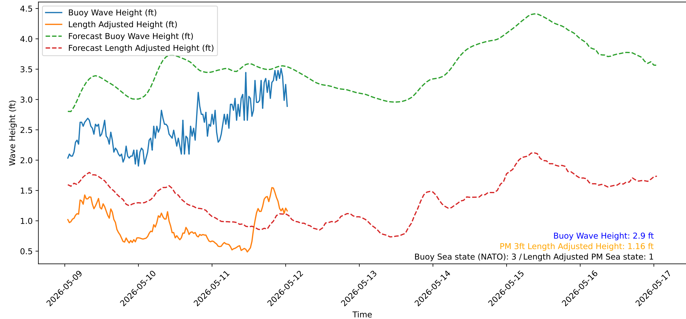
Wave Heights over Time for Green Beach at 2026-05-12 01:11:12
