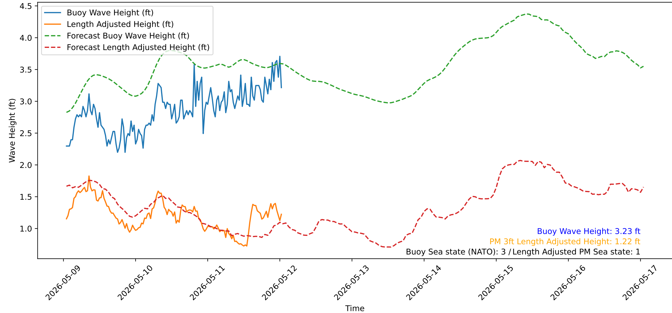
Wave Heights over Time for Oceanside Harbor at 2026-05-12 01:10:31
