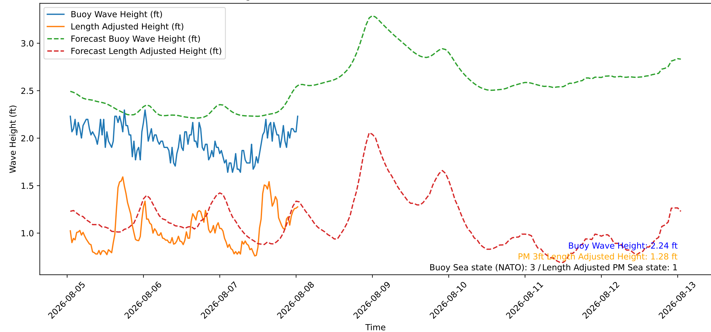
Wave Heights over Time for Oceanside Harbor at 2026-08-08 01:10:26
