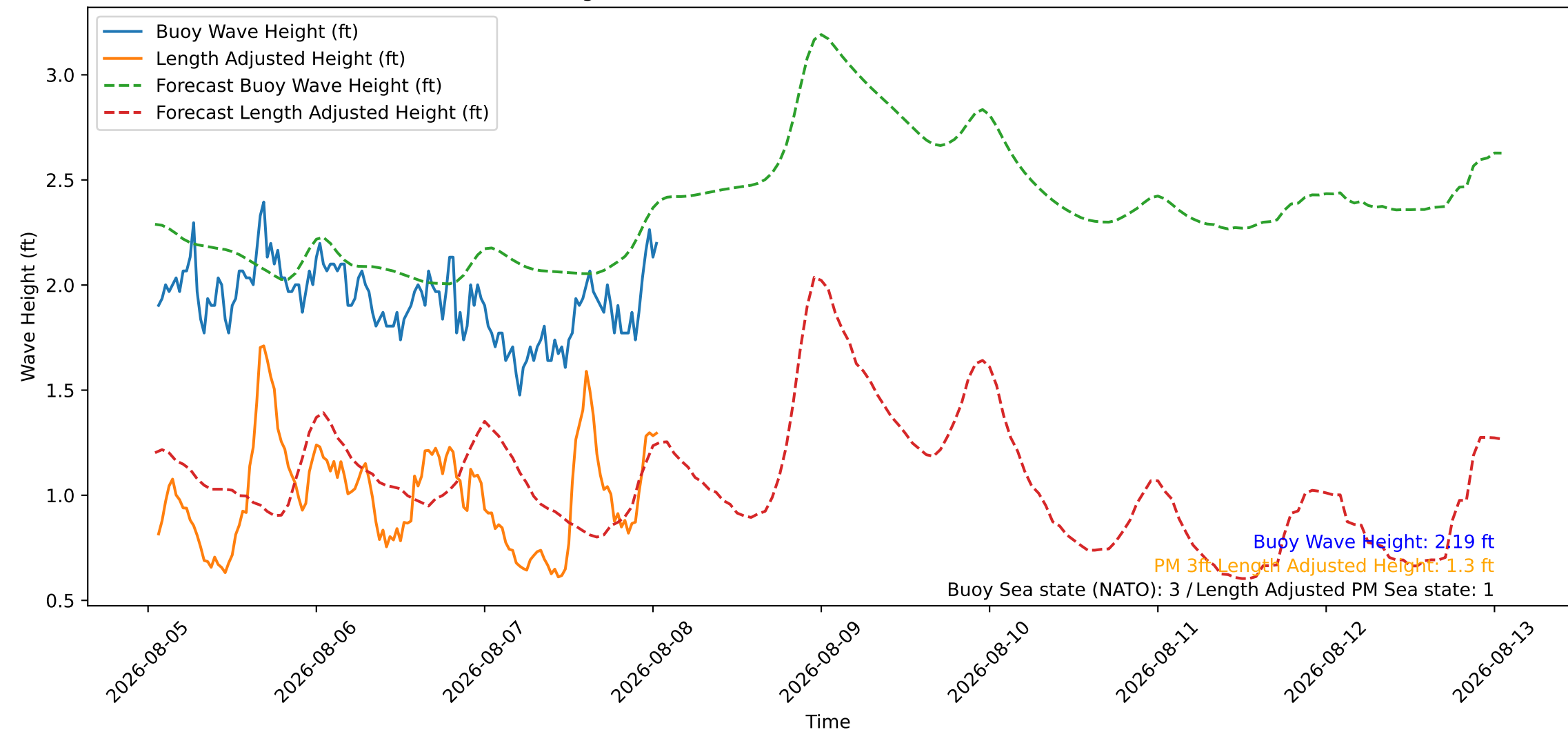
Wave Heights over Time for Red Beach at 2026-08-08 01:10:46
