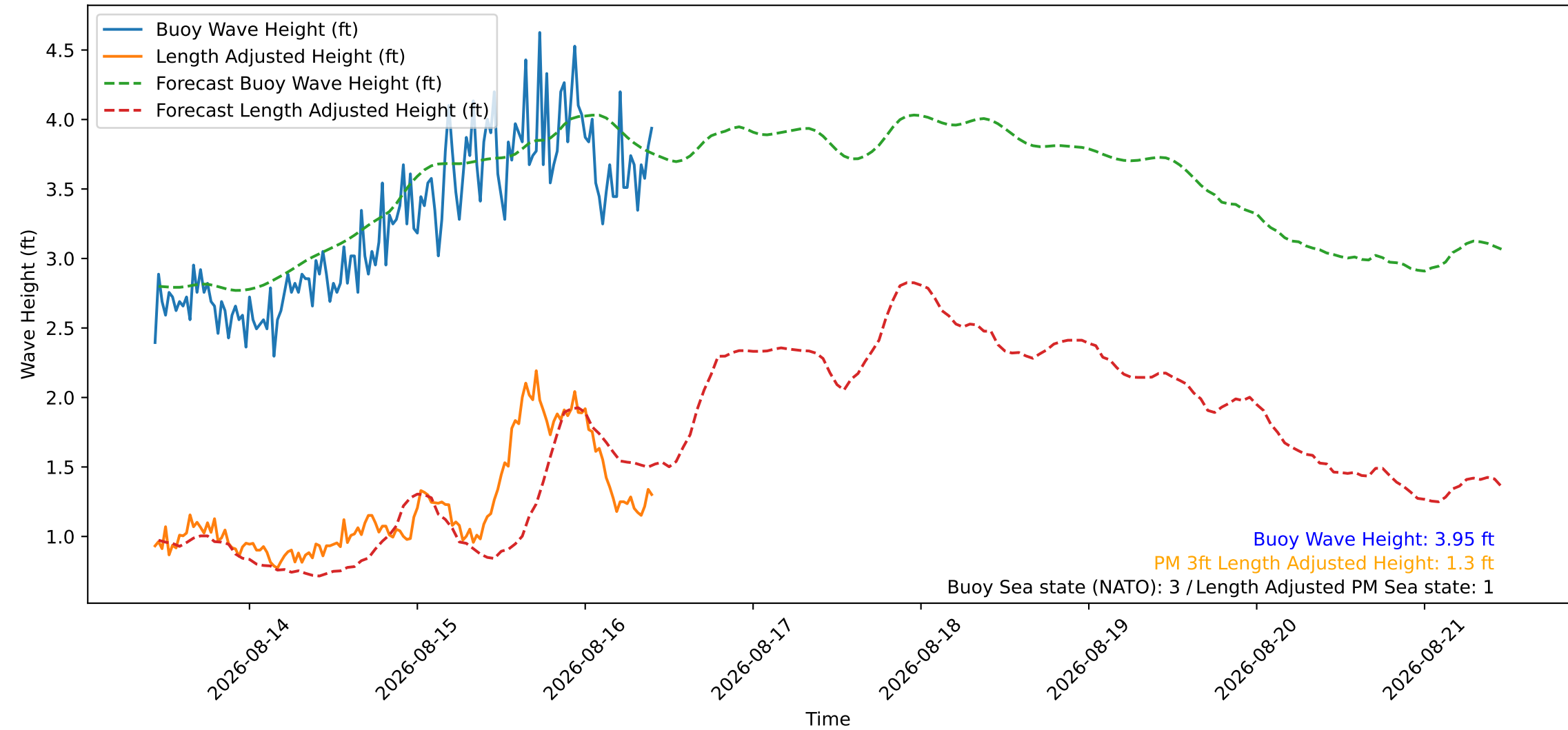
Wave Heights over Time for Oceanside Harbor at 2026-08-16 10:30:26
